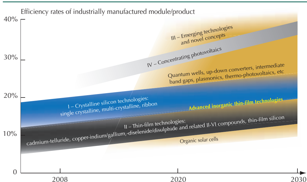
Figure 6.5 PV technology status and prospects
