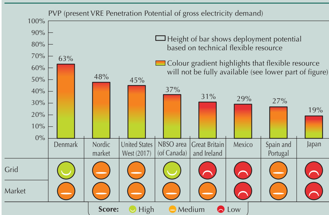
Figure 3.6 Present variable RE potential in various systems
