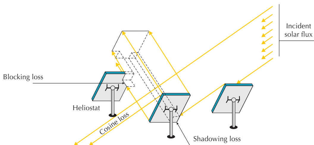
Figure 7.10 Blocking, shading and cosine losses in heliostat fields
