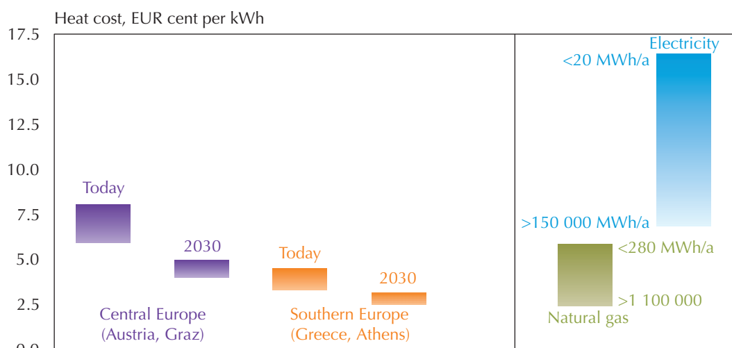
Figure 7.11 Price of solar thermal generated heat versus conventional energy sources, for solar supported heating networks and low temperature industrial process applications > 350\text{kW}_{\text{th}}
