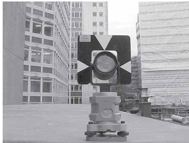
Figure 4.7c Leica target incorporating Tribrach (bottom), optical plummet section. In this instance it is a laser optical plummet which shines a laser onto the floor, prism and target plate.
