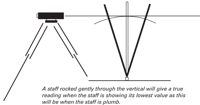
Figure 4.6 Staff plumbness.
