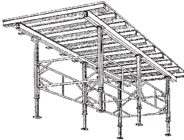
Figure 11.4 Typical aluminium table form (source, Ischebeck Titan brochure).
