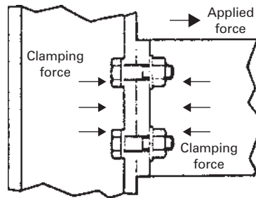
Figure 14.10 Load held by bolts in tension.
