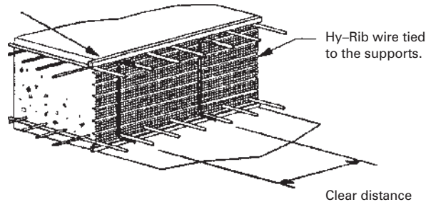
Figure 11.3 Typical Hy-Rib stop end (source, Expamet Building Products).
