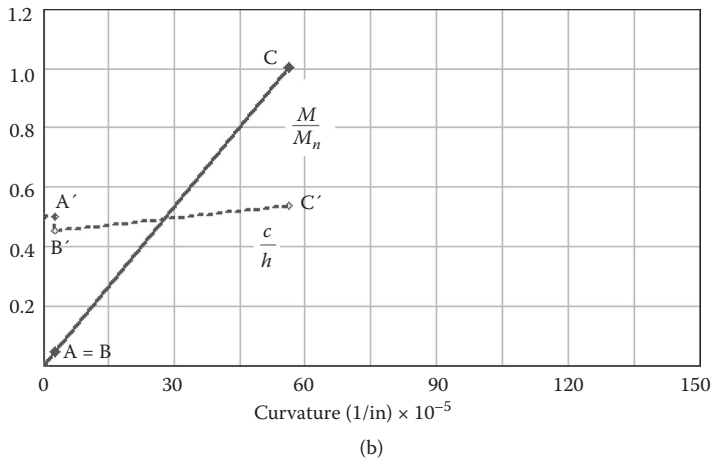
Figure 4.3 Moment-curvature diagram for RC beams reinforced with steel bars: (a) under-reinforced member ( b = 8 in., d = 16 in., A_s = 0.80 in 2 ); (b) over-reinforced member ( b = 16 in., d = 8 in., A_s = 5.67 in 2 ).
