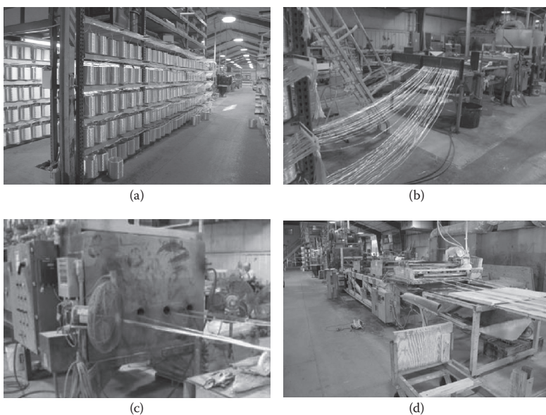
Figure 2.2 Phases of the manufacturing process of GFRP bars: (a) raw glass fibers in rovings; (b) glass fibers drawn through a resin bath for impregnation and a metal die; (c) solid bar emerging from the curing oven; (d) cured bar ready to be cut at the desired length.
