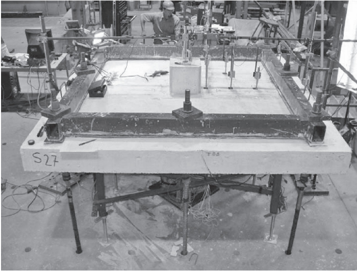
(a) Test setup for 8 in. (200 mm) thick slab
