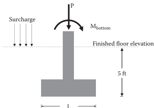
Figure 10.1 Schematic view of footing under column B3.
