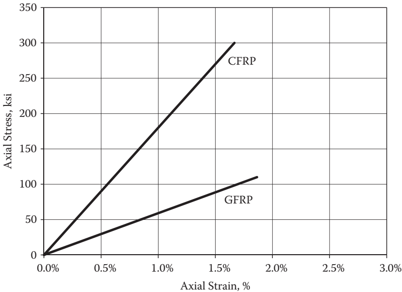
Figure 3.3 Typical tensile stress–strain curve of no. 3 GFRP and CFRP bars.
