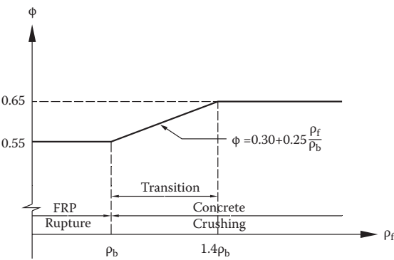
Figure 4.9 Strength-reduction factor as per ACI 440.1R-06.
