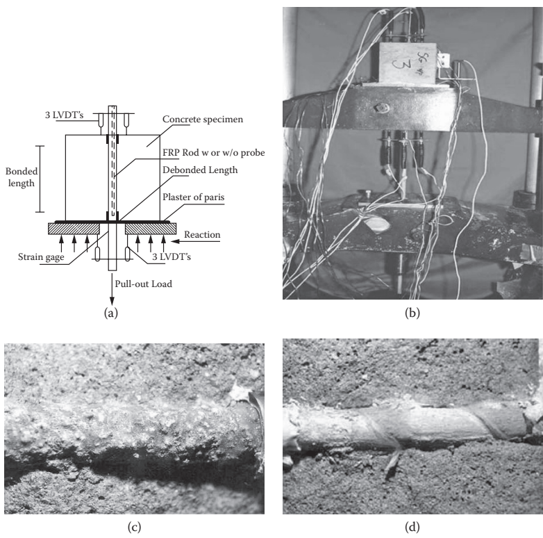
Figure 3.7 (a) Direct pullout bond test schematic; (b) typical pullout bond test setup; (c, d) typical failure modes of a GFRP bar specimen.
