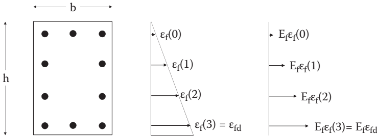
Figure 9.8 Neutral axis depth c = 0 .
