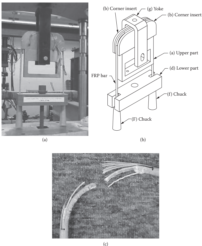
Figure 3.14 (a) Typical test setup; (b) assembled test fixture sketch; (c) typical failure mode of a bent GFRP.
