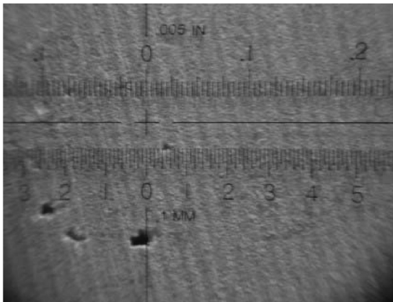
Figure 3.16 Voids in the cured material due to lack of glass.
