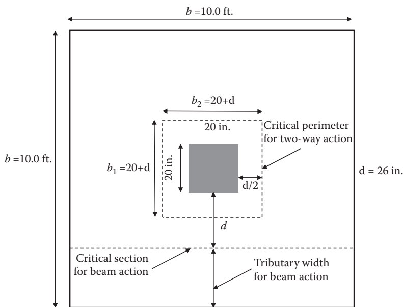
Figure 10.3 Critical cross sections for shear strength checks.
