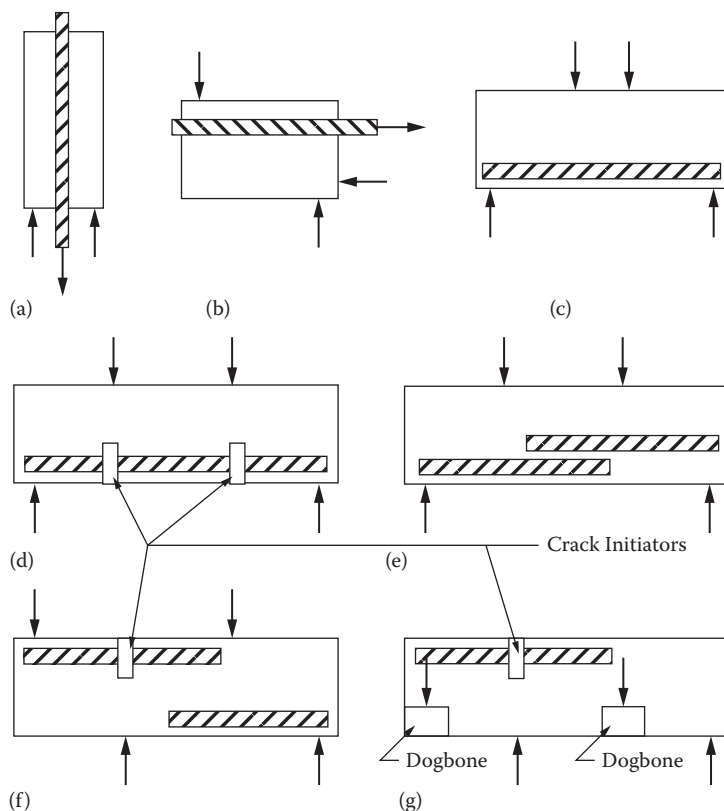
Figure 3.6 Types of test methods for different bond values of FRP reinforcement in concrete: (a) pullout specimen; (b) beam-end specimen; (c) simple beam specimen; (d) hinged beam-end specimen; (e) splice specimen; (f) cantilever beam specimen (without dogbones); and (g) cantilever beam specimen (with dogbones) (ACI 440-3R).
