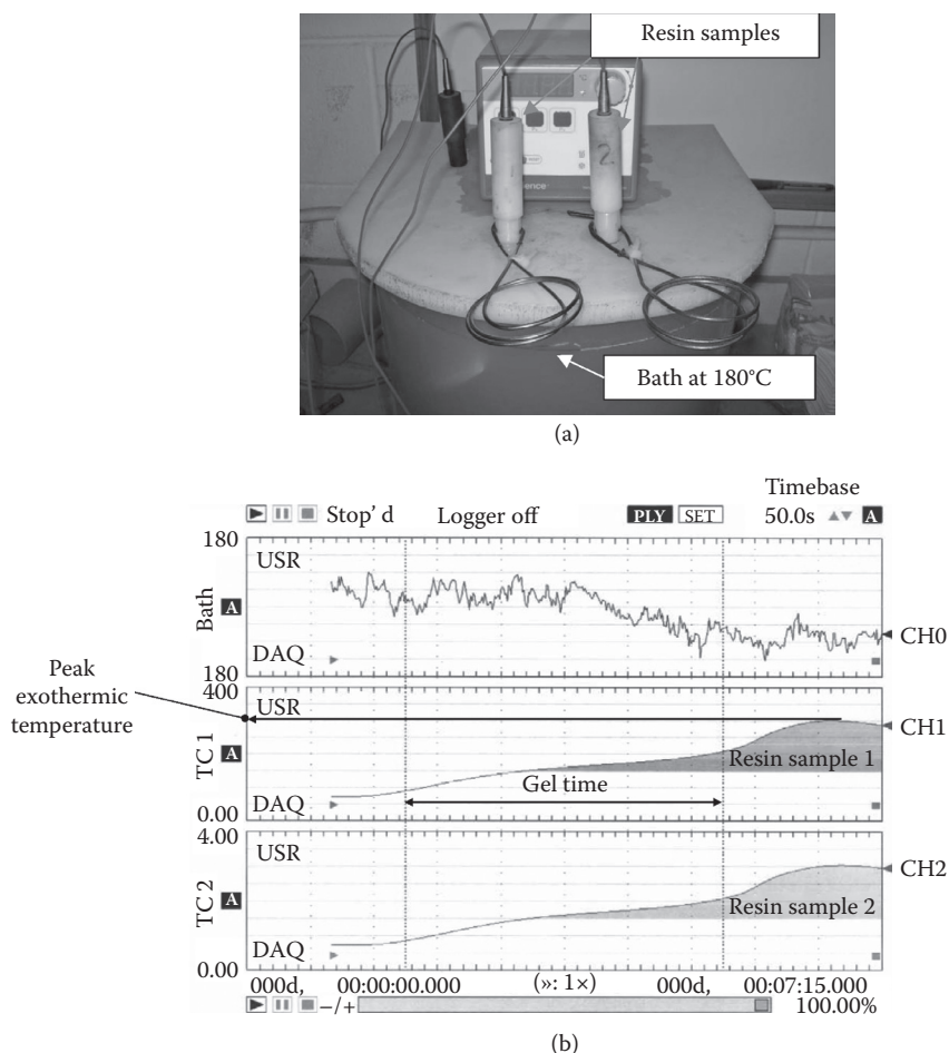
Figure 2.5 Test method for resin gel time and peak exothermic temperature: (a) test setup; (b) typical test result.
