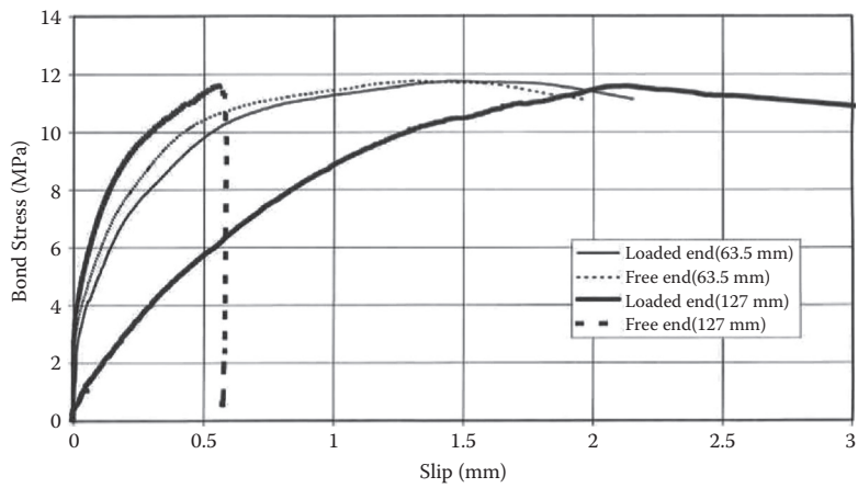
Figure 3.8 Typical free and loaded end bond-slip curves of a no. 4 GFRP bar.
