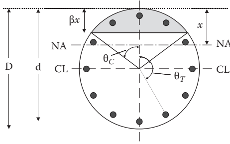
Figure 5.4 Cross section of a circular column with N.A. within the cross section.
