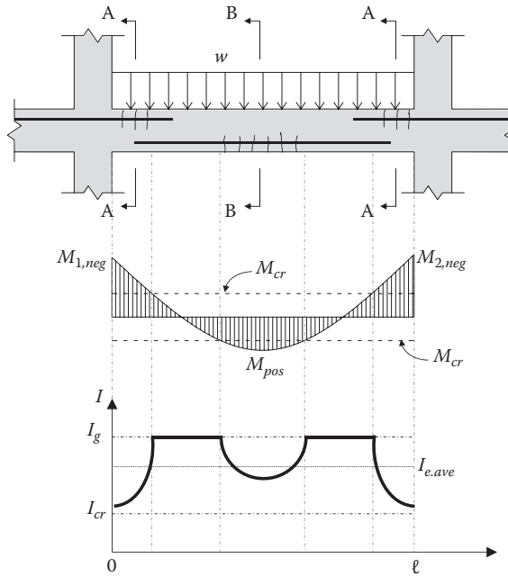
Figure 4.12 Moment of inertia for a continuous beam.
