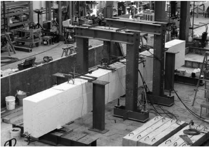
Figure 4.15 Test setup for shear test. (A. K. Matta et al. ACI Structures Journal 110 (4): 617–628, 2013.)
