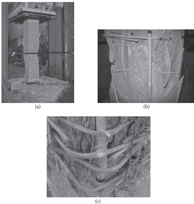
Figure 5.1 Concrete columns of rectangular cross section reinforced with GFRP longitudinal bars and ties. (a) overall view of failed column with 12-inch tie spacing; (b) detail of longitudinal bar buckling for column with 12-inch tie spacing; and (c) detail of longitudinal bar and tie rupture for column with 3-inch tie spacing; (De Luca, Matta, and Nanni. 9th International Symposium on Fiber Reinforced Polymer Reinforcement for Concrete Structures (FRPRCS-9) , D. Oehlers, M. Griffith, and R. Seracino, eds., July 13–15, 2009, Sydney, Australia, CD-ROM, 4, 2010.)
