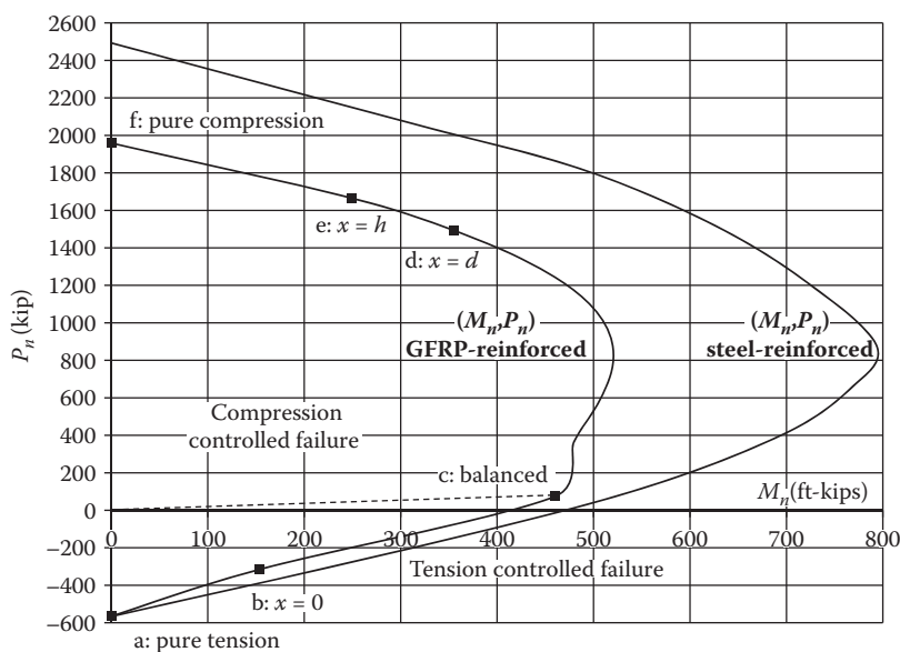
Figure 5.5 Interaction diagrams of GFRP and steel RC columns (square cross section).
