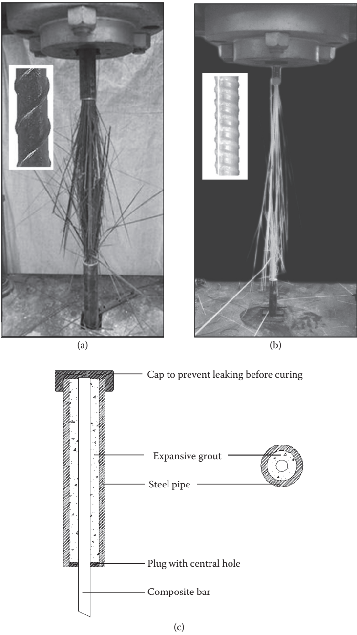
Figure 3.4 Successful axial tension tests: (a) 1.5 in. (38.1 mm) diameter bar; (b) 3/8 in. (9.5 mm) diameter bar; and (c) anchor schematics.
