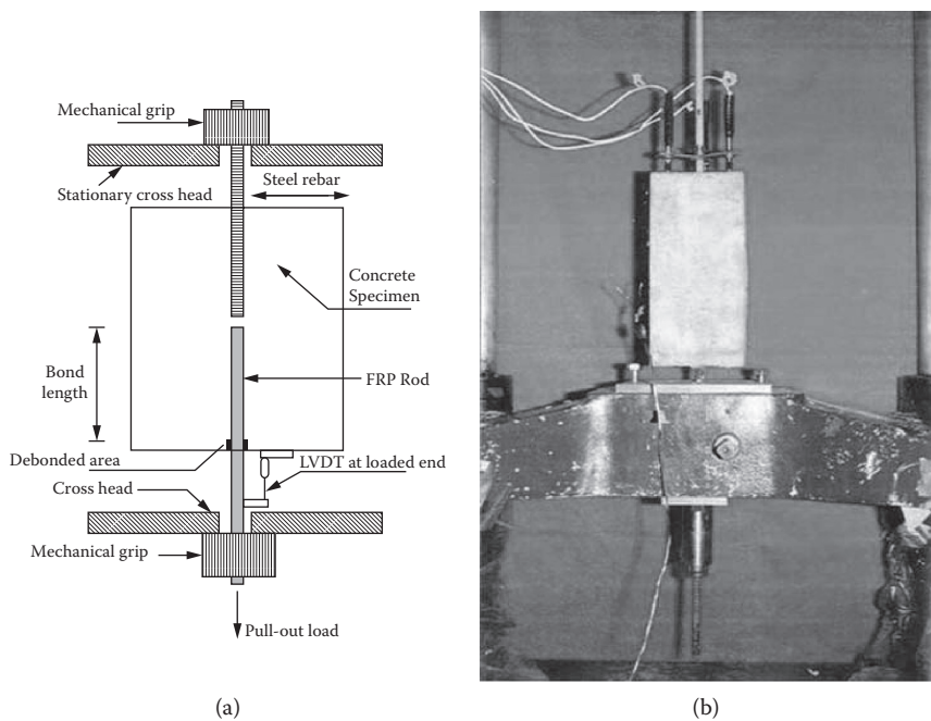
Figure 3.9 Rod-rod pullout bond test: (a) schematic and (b) photographic views.
