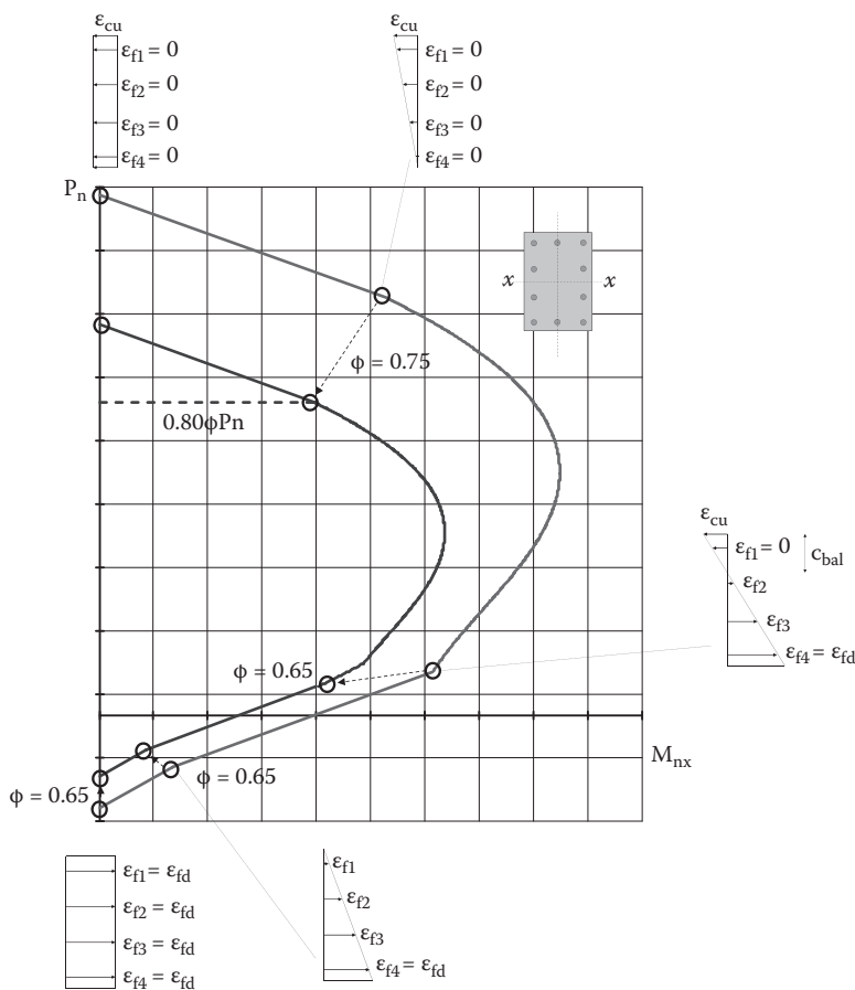
Figure 5.7 Rectangular section P_n – M_{nx} diagram.
