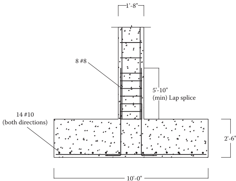
Figure 10.4 Final reinforcement layout.
