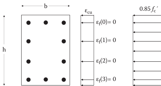
Figure 9.5 Pure compression.
