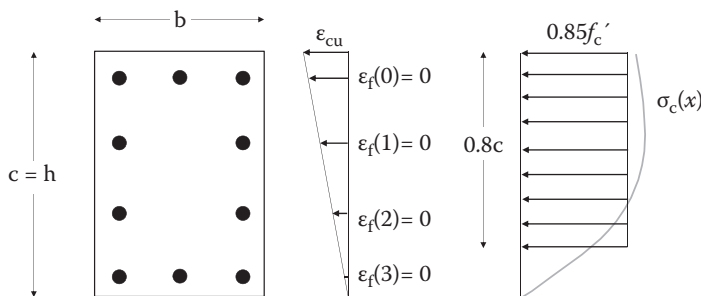
Figure 9.6 Neutral axis at the lowest level of fibers.
