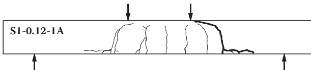
Figure 4.16 Crack pattern of large-sized GFRP-RC beam subject to shear-compression failure. (A. K. Matta et al. ACI Structures Journal 110 (4): 617–628, 2013.)
