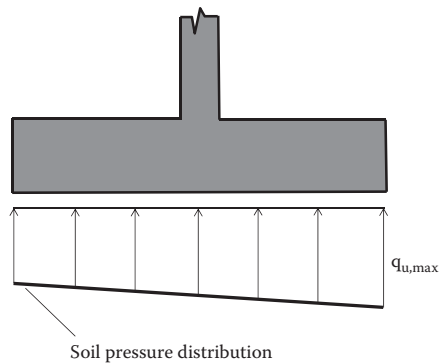
Figure 10.2 Soil pressure distribution.
