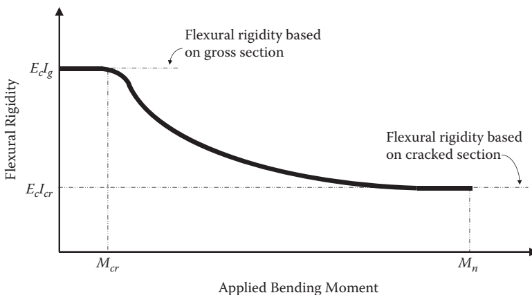
Figure 4.13 Flexural rigidity versus applied bending moment relationship.
