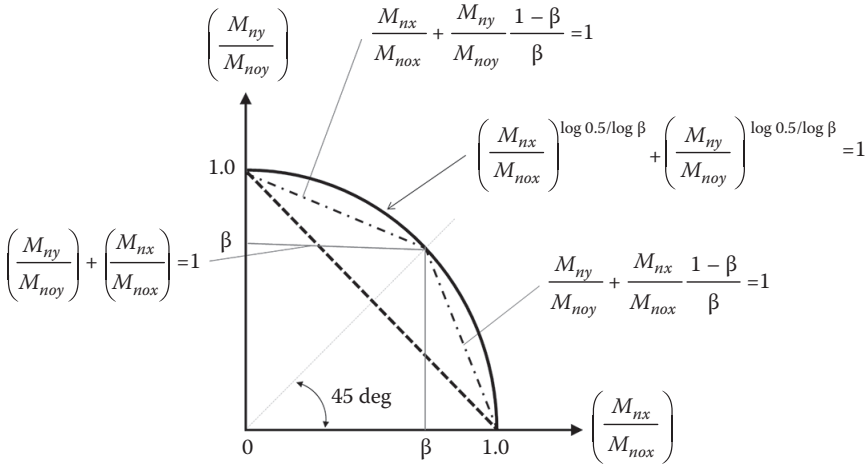
Figure 5.11 Adimensional load contour at a constant P_n .
