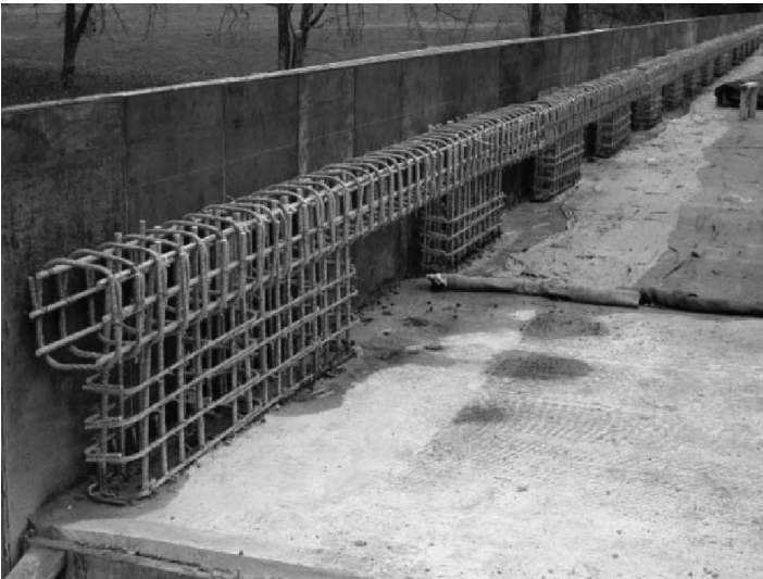
Figure 1.7 GFRP cages prior to casting a bridge railing (Greene county, Missouri).
