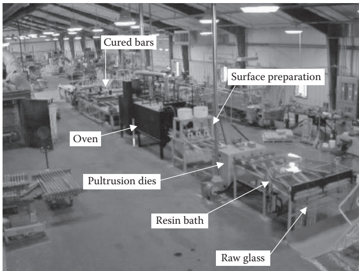
Figure 2.1 Overall view of the production line of GFRP bars.
