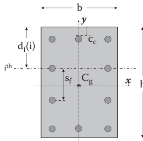
Figure 9.4 Generic rectangular cross section.
