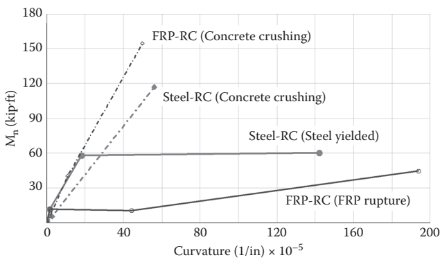
Figure 4.5 Moment-curvature diagram for steel and GFRP beams. Note: 1 ft-kip = 1.36 KN-m; 10^{-5} 1/in. = 3.9 \cdot 10^{-4} 1/m.
