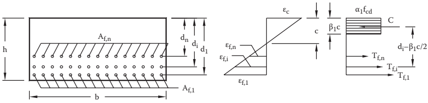
Figure 4.11 Flexural member with multiple layers of FRP reinforcement.
