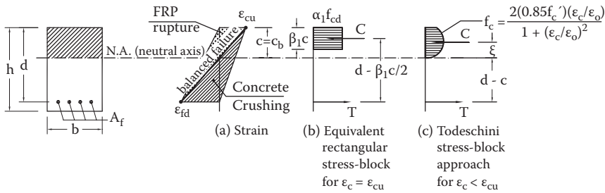
Figure 4.2 Failure mode regions for FRP RC flexural members.
