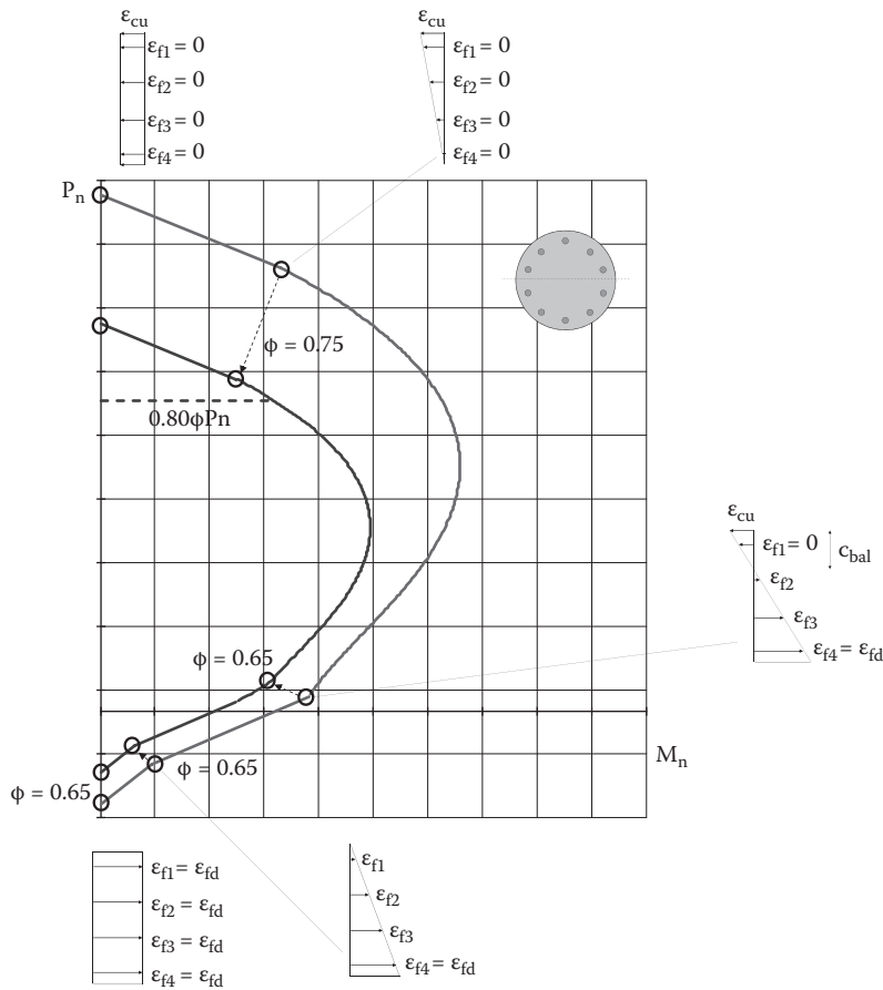
Figure 5.9 Circular section P_n – M_n diagram.
