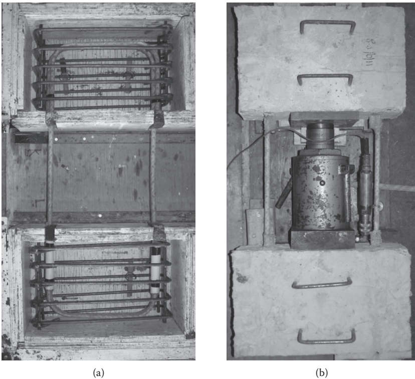
Figure 3.13 Views of the (a) test setup and (b) a failed specimen.
