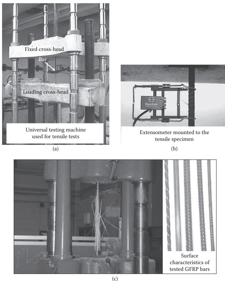
Figure 3.2 (a) Typical tensile test setup; (b) close-up view of the extensometer used to measure the axial deformation; (c) typical failure mode of a GFRP bar specimen.
