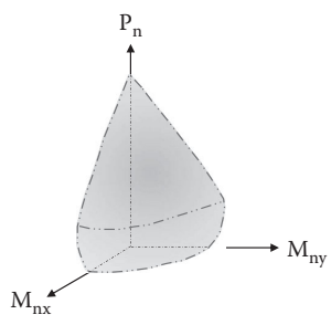
Figure 5.10 Interaction surface for the case of compression and biaxial bending.
