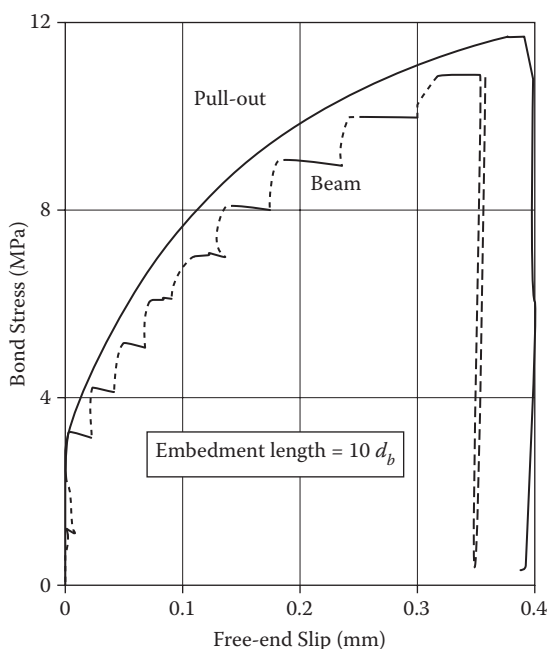
Figure 3.12 Comparison of the test results obtained by direct pullout versus beam-type pullout on no. 4 GFRP bar.
