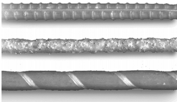
Figure 2.3 Surface deformation patterns for commercially available FRP bars: ribbed (top); sand-coated (middle); and wrapped and sand-coated (bottom).
