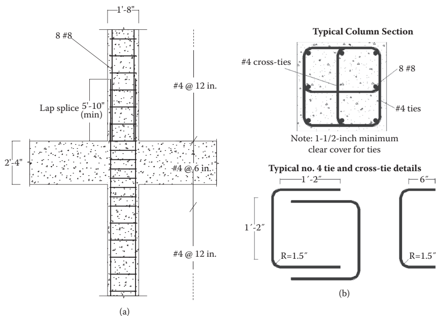
Figure 9.10 (a) Reinforcement layout; (b) typical detail.
