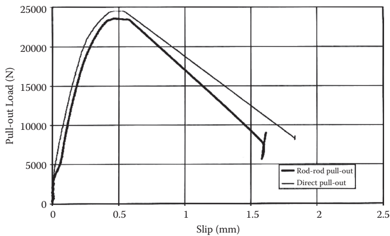
Figure 3.10 Comparison of the test results obtained by direct pullout versus rod-rod pullout on no. 4 GFRP bar.
