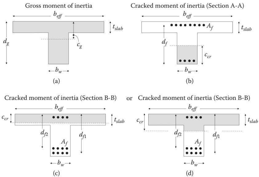
Figure 4.14 Gross and cracked moments of inertia of a T-beam.
