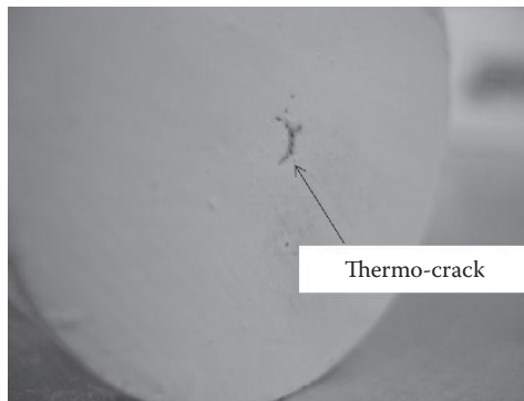
Figure 2.4 Thermocracking due to undercuring of the resin.
