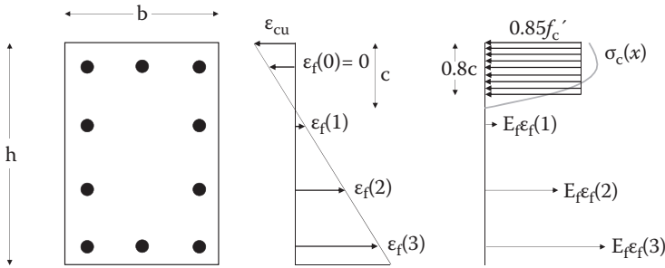
Figure 9.7 Neutral axis depth h \geq c \geq c_{\text{bal}} .
