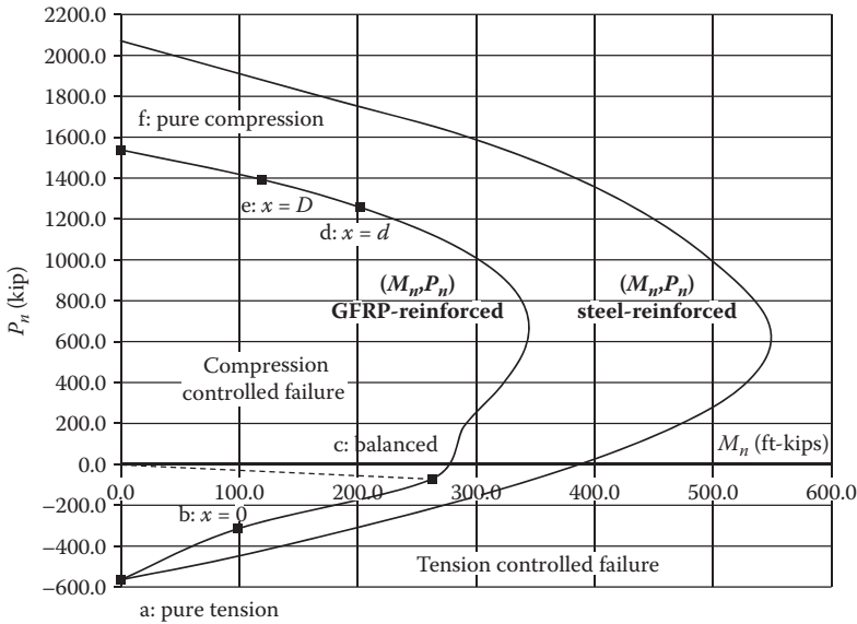
Figure 5.6 Interaction diagrams of GFRP and steel RC columns (circular cross section).
