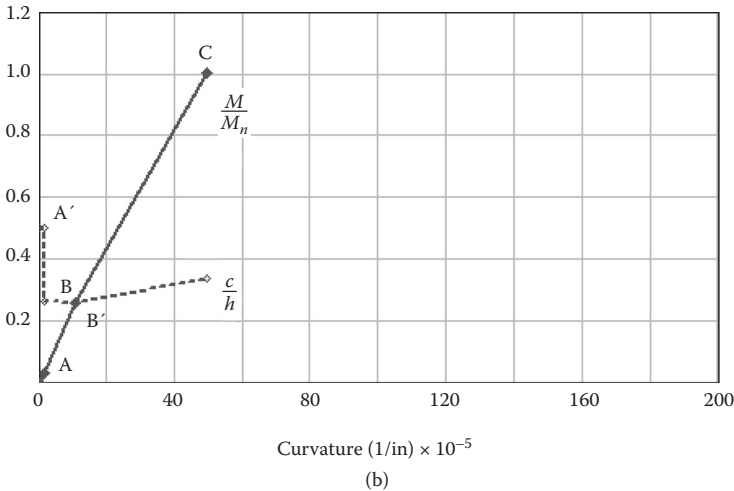
Figure 4.4 Moment-curvature diagram for RC beams reinforced with FRP bars: (a) FRP rupture ( b = 8 in., d = 16 in., A_f = 0.35 in 2 .); (b) concrete crushing ( b = 8 in., d = 16 in., A_f = 5.55 in 2 .)
