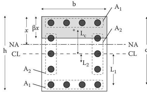
Figure 5.3 Cross section of a rectangular column with N.A. within the cross section.
