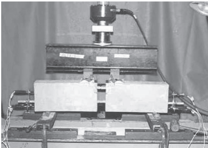
Figure 3.11 Beam-type pullout bond test: (a) schematic and (b) photographic views.
