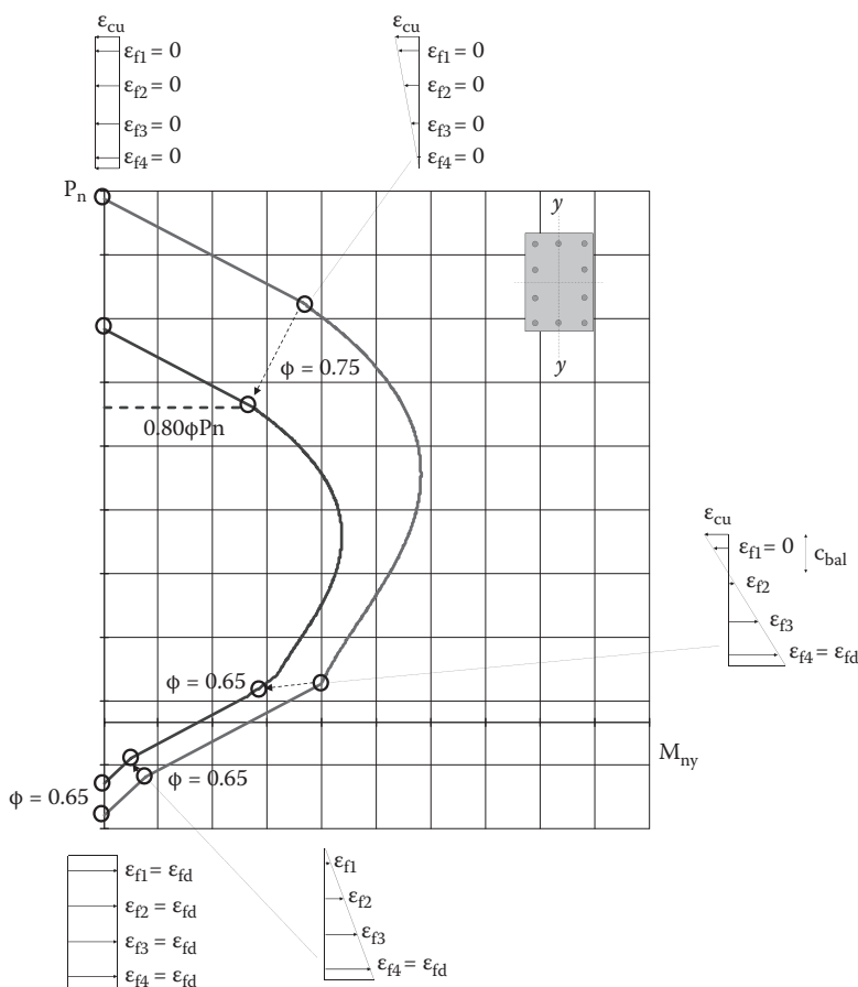
Figure 5.8 Rectangular section P_n – M_{ny} diagram.
