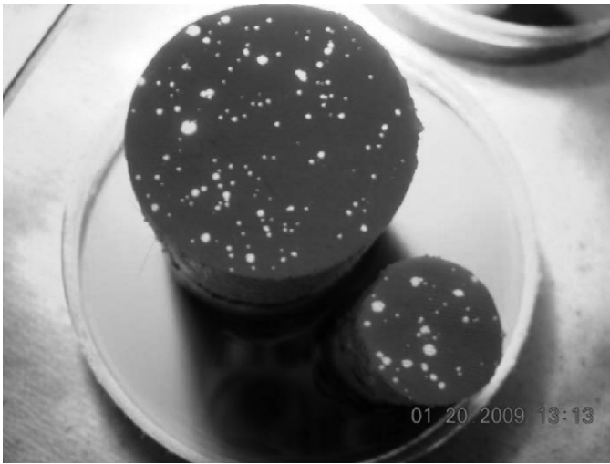
Figure 3.19 Voids due to the presence of hollow glass fibers.
