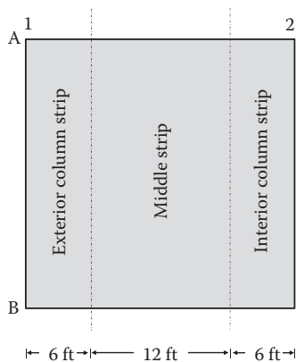
Figure 8.2 Column and middle strips relative to the design panel.
