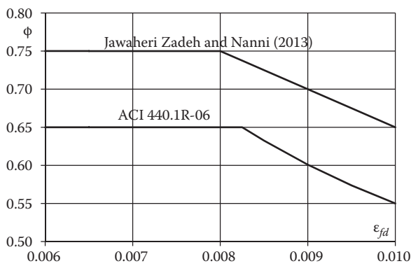
Figure 4.10 Comparison of the strength-reduction factors ( \epsilon_{fu} = 0.01 ).
