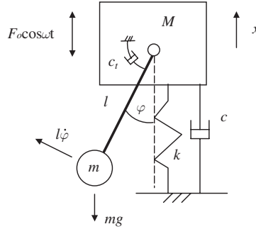
Figure 5.12 Pendulum absorber.
