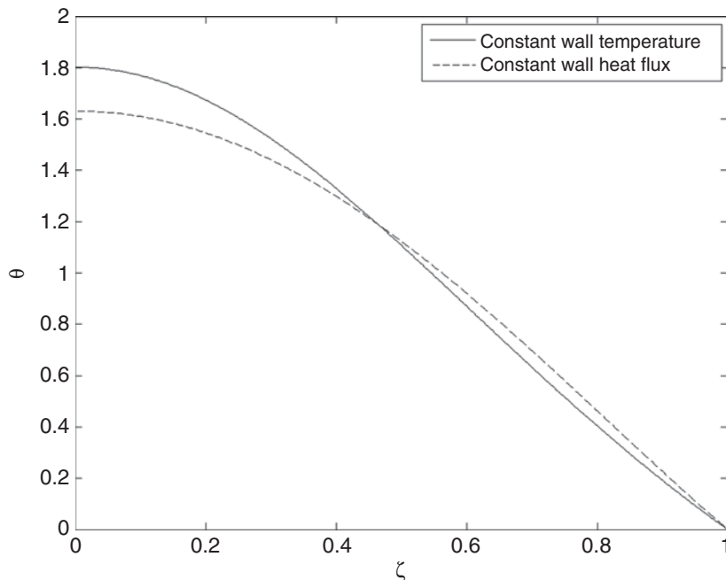
Figure 12.7 Temperature versus radial position for laminar pipe flow with different boundary conditions: (i) constant wall temperature and (ii) constant wall heat flux.
