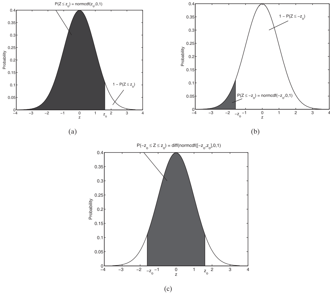
Figure 8.5 Relationship of cdf to normcdf: (a) Z \leq z_0 (b) Z \leq -z_0 (c) -z_0 \leq Z \leq z_0 .
