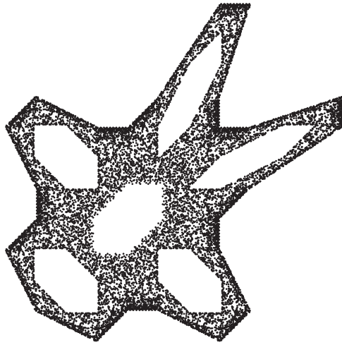
Figure 6.34 Gingerbread man.
