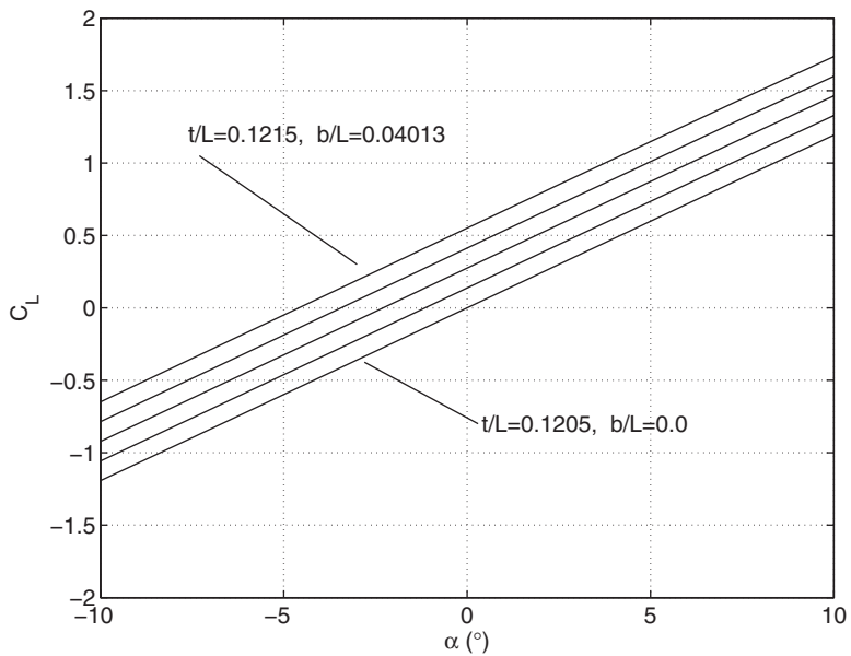
Figure 11.33 Lift coefficient C_L versus angle of attack \alpha for \xi_{off} = -0.093 and \eta_{off} = 0, 0.02, 0.04, 0.06 , and 0.08 .
