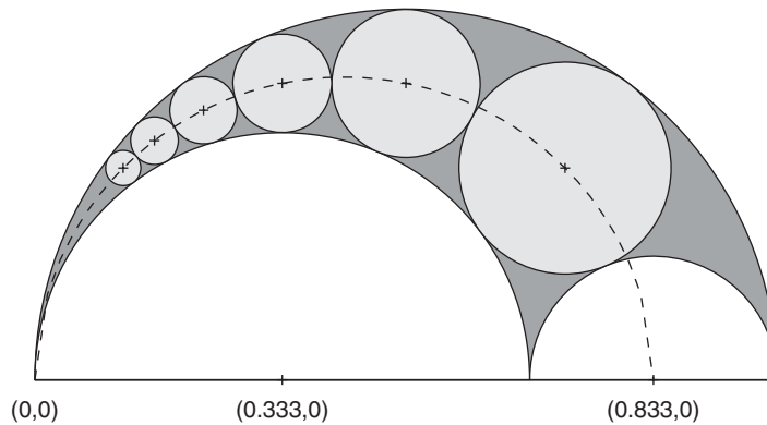
Figure 6.49 Pappus chain.
