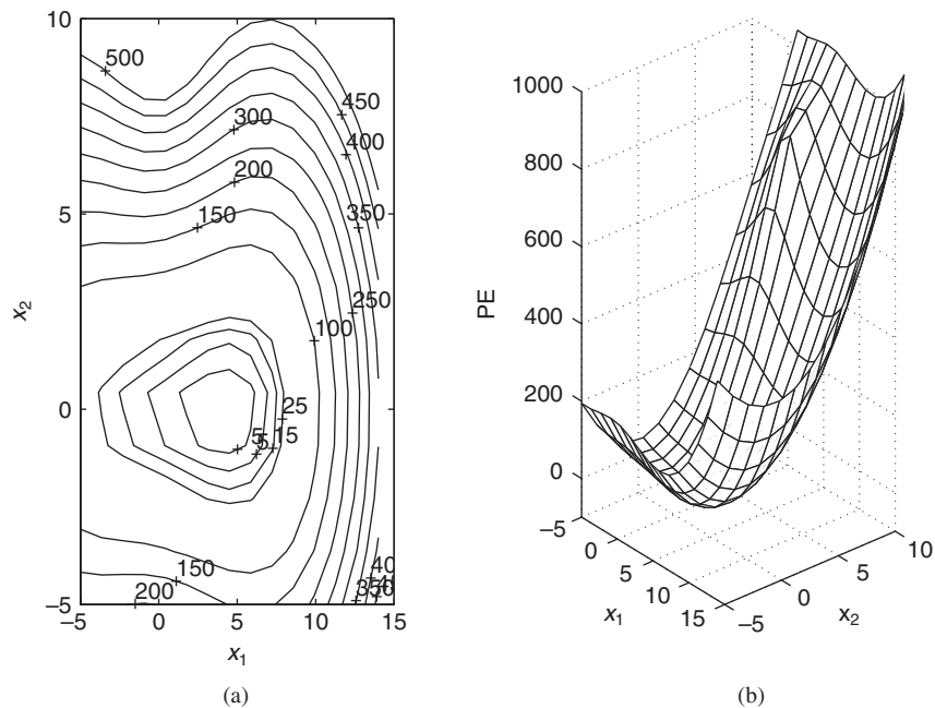
Figure 13.23 (a) Contour and (b) surface plots of the PE function for the two-spring system shown in Figure 13.22.
