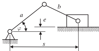
Figure 2.7 Slider–crank mechanism.
