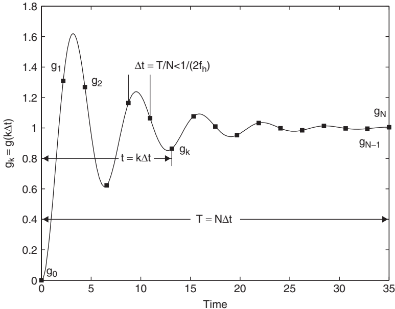
Figure 5.4 Sampled waveform.
