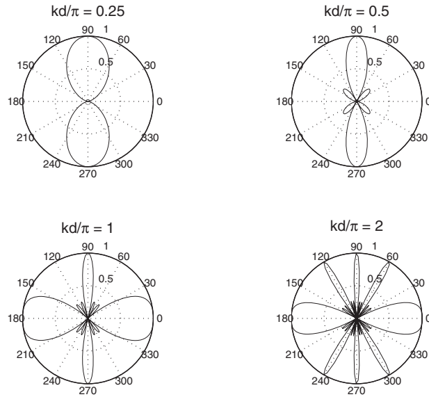
Figure 6.48 Radiation pattern of an acoustic array for N = 2 .
