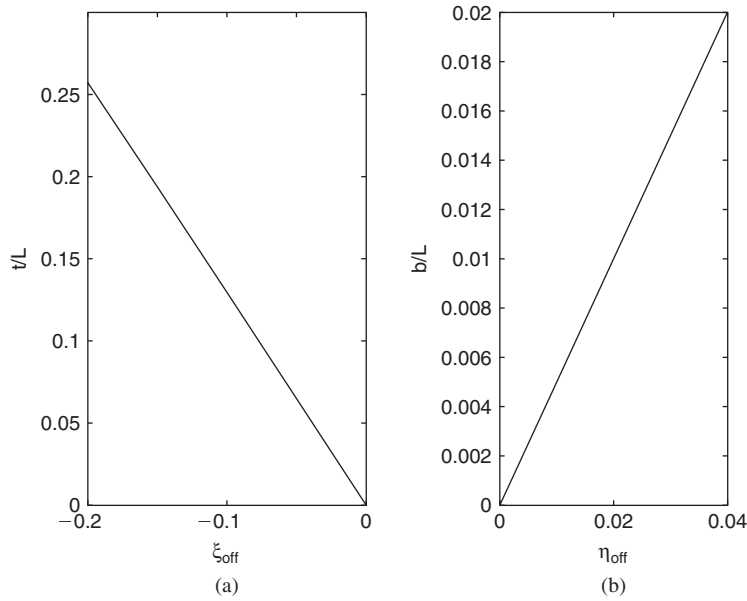
Figure 11.31 (a) Foil thickness versus \xi offset. (b) Foil camber versus \eta offset. In figure (a), five curves are drawn for \eta_{\text{off}}/R = 0, 0.01, 0.02, 0.03 , and 0.04 . In figure (b), five curves are drawn for \xi_{\text{off}}/R = -0.2, -0.15, -0.10, -0.05 , and 0.0 . Note that in each plot the five curves are virtually on top of one another.
