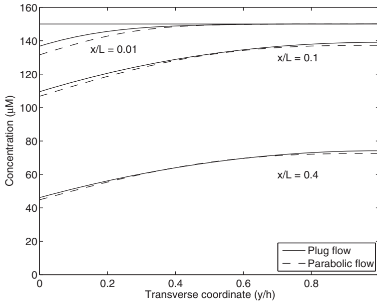
Figure 14.7 Oxygen concentration versus the transverse coordinate \hat{y} at \hat{x} = 0.01, 0.1 , and 0.4 . The horizontal line at C = 150 \mu\text{M} represents the inlet concentration C_{\text{in}} .
