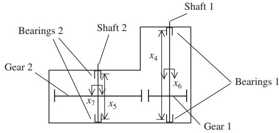
Figure 13.8 Gear reducer.
