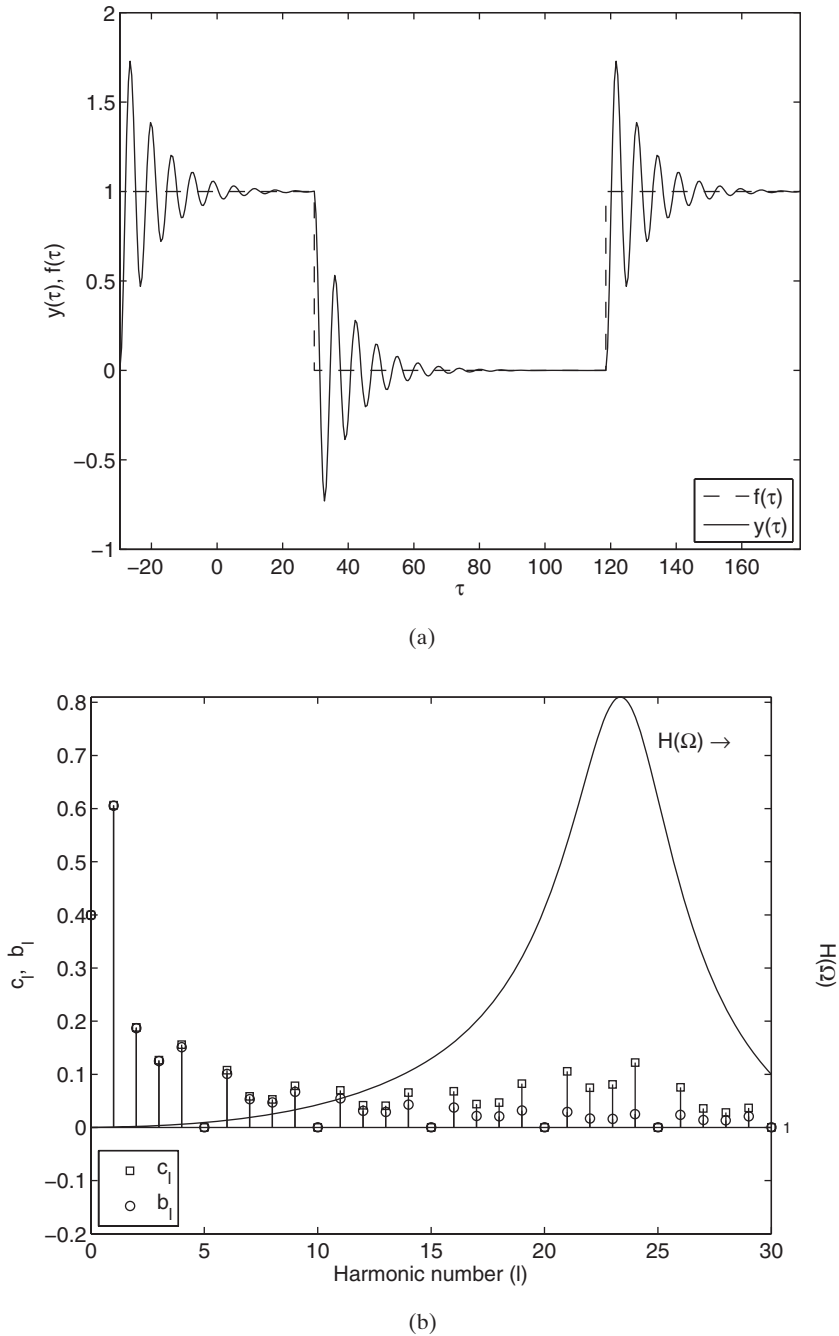
Figure 9.12 Comparison of a periodic pulse train in the (a) time domain and (b) frequency domain.
