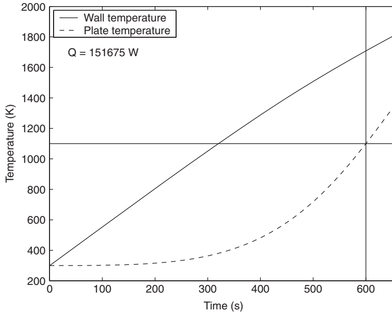
Figure 12.21 Temperature as a function time in the plate and in the furnace.
