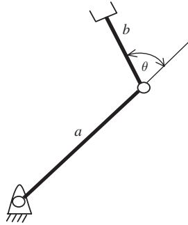
Figure 13.9 Planar two-link manipulator.
