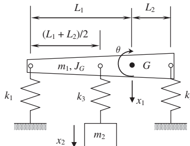
Figure 9.36 Three-degree-of-freedom system.
