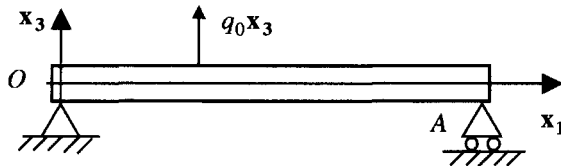
Figure 13.3. Beam subjected to a sinusoidal load
