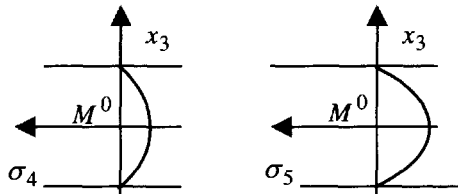
Figure 6.8. Transverse shear stress variations
