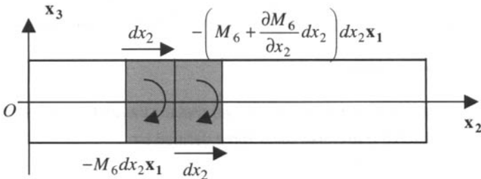
Figure 5.10. Couples acting on two elements next to the edge x_1 = a_1
