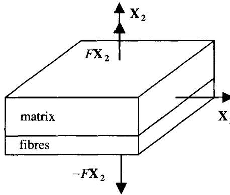
Figure 3.2. Transverse tension
