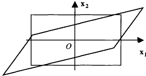
Figure 2.4. Strains when S_{16} \neq 0
