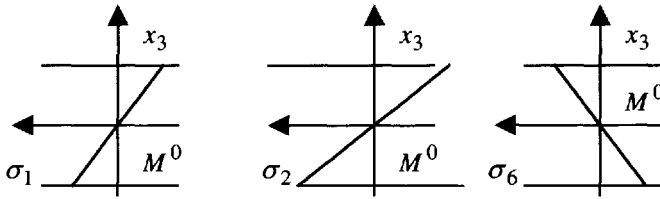
Figure 6.6. Stress variations
