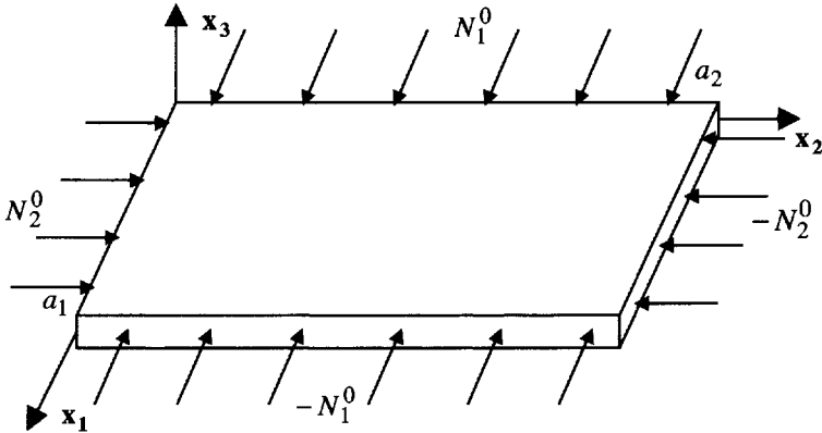
Figure 9.6. Buckling of balanced, asymmetrical plate
