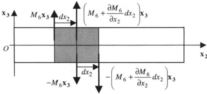
Figure 5.11. Equivalent forces acting on two elements next to the edge x_1 = a_1
