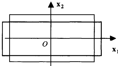
Figure 2.5. Strains when S_{16} = 0
