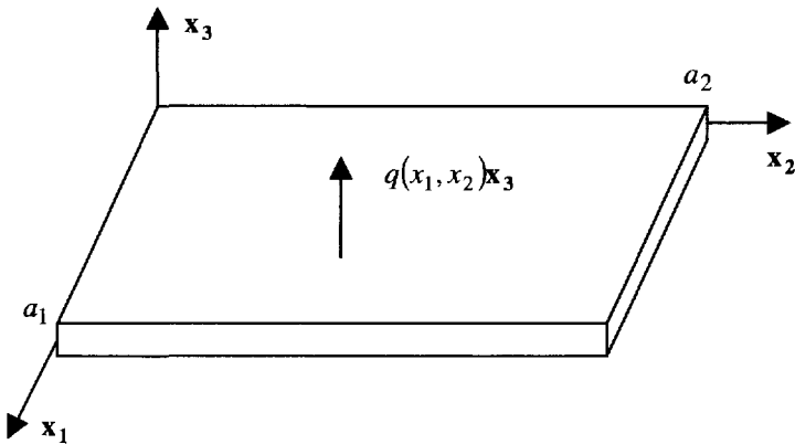
Figure 9.1. Cross-ply asymmetrical plate in flexure
