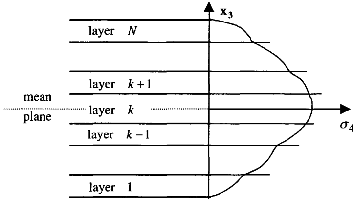
Figure 5.16. Transverse shear stress distribution
