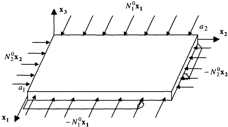
Figure 6.12. Buckling loads
