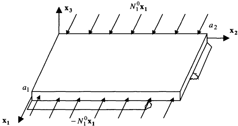
Figure 6.13. Compression loading in one direction
