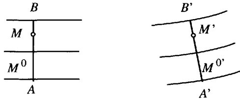
Figure 15.4. Displacements in Kirchhoff-Love type analysis
