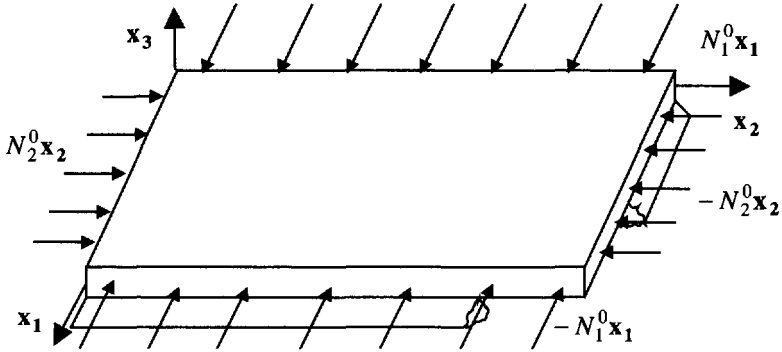
Figure 8.3. Buckling loading
