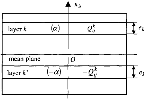
Figure 5.4. Balanced laminate
