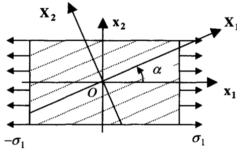
Figure 4.7. Tensile test off-axis
