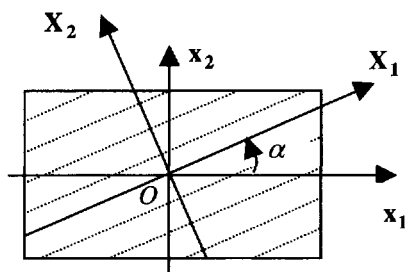
Figure 2.2. Off-axis directions
