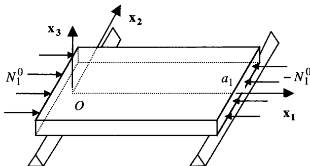
Figure 11.2. Plate in buckling situation
