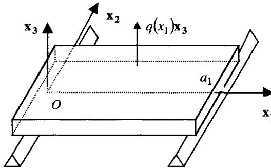
Figure 11.1. Plate in cylindrical flexure
