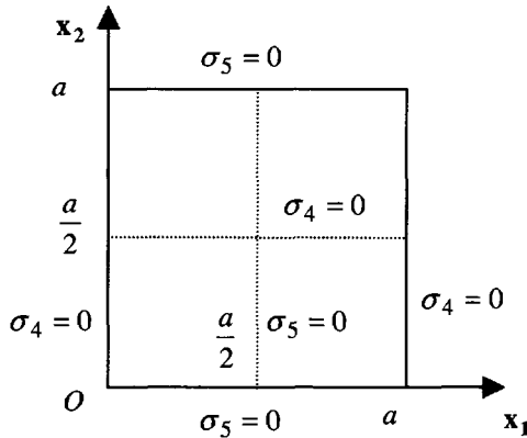
Figure 6.9. Zero transverse shear stresses
