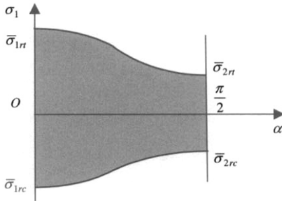
Figure 4.3. Tsai-Hill criterion, simple tension
