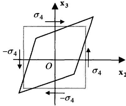
Figure 1.3. Simple shear
