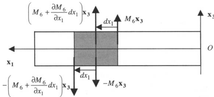
Figure 5.14. Equivalent forces acting on two contiguous edge elements x_2 = a_2
