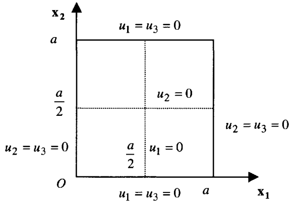
Figure 6.3. Zero displacement
