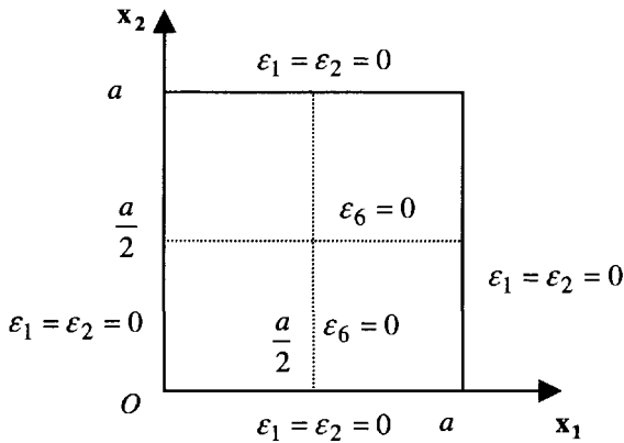
Figure 6.5. Zero strain
