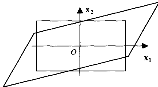
Figure 2.7. Strains when S_{16} \neq 0 , S_{26} \neq 0 , S_{36} \neq 0
