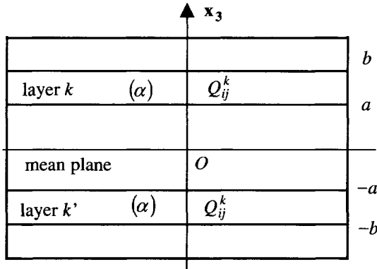
Figure 5.3. Mirror symmetry
