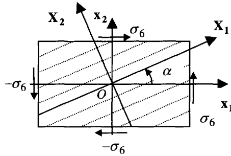
Figure 2.6. Shear in off-axis directions
