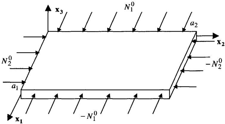
Figure 9.3. Buckling asymmetrical cross-ply plate
