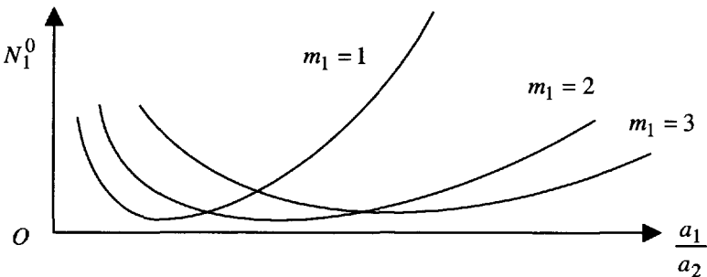
Figure 6.14. Critical buckling loads
