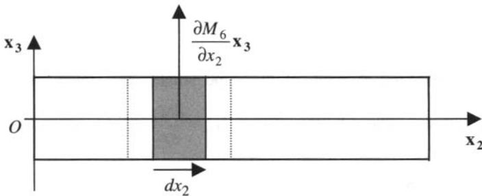
Figure 5.12. Linear equivalent force density acting on two half-elements next to the edge x_1 = a_1
