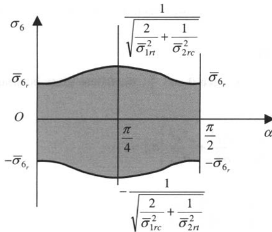
Figure 4.6. Tsai-Hill criterion for pure shear
