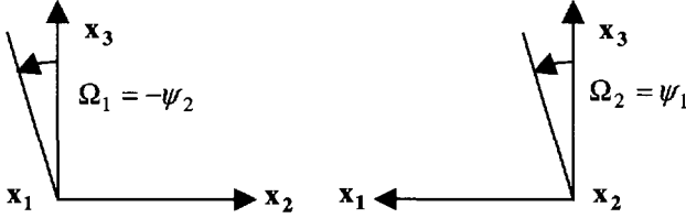
Figure 15.3. Infinitesimal rotations
