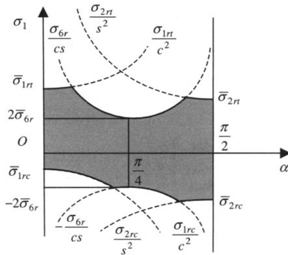
Figure 4.2. Maximum stress criterion, simple tension
