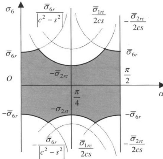
Figure 4.5. Maximum stress criterion for pure shear
