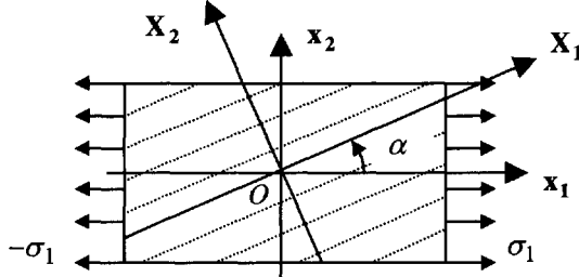
Figure 2.3. Tension off-axis
