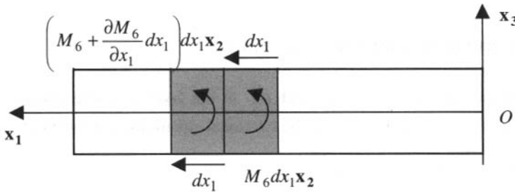
Figure 5.13. Couples acting on two contiguous edge elements x_2 = a_2
