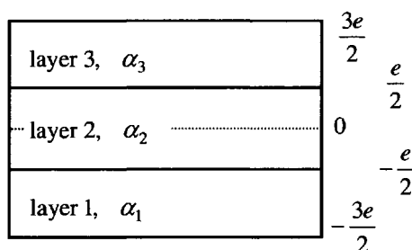
Figure 5.7. Three layer plate
