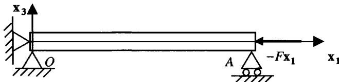
Figure 13.4. Beam buckling
