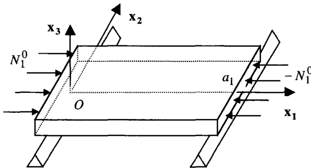
Figure 10.2. Plate subjected to buckling
