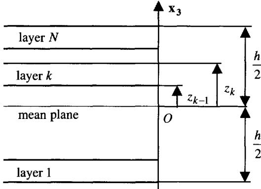
Figure 5.2. Distribution of layers in the composite
