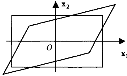
Figure 2.8. Strains when S_{16} = S_{26} = S_{36} = 0
