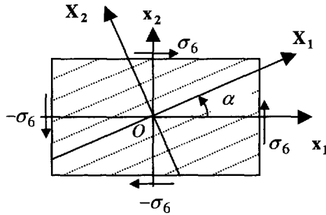
Figure 4.4. Off-axis shear
