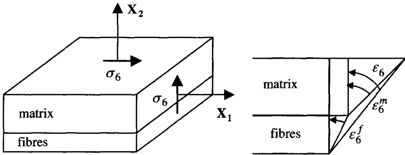
Figure 3.3. Shear
