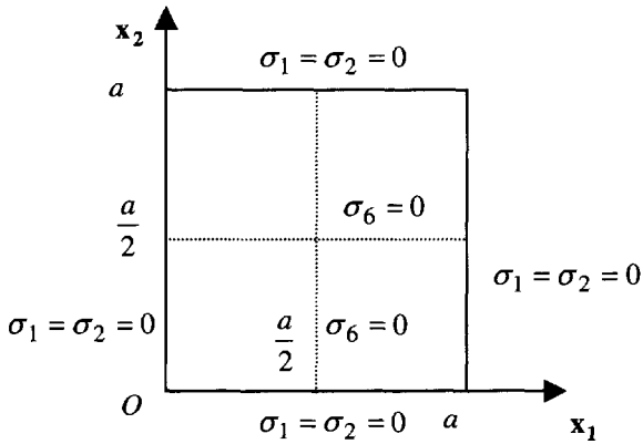
Figure 6.7. Zero stresses
