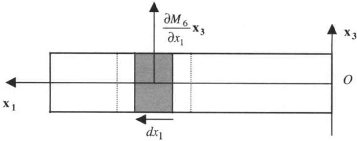
Figure 5.15. Equivalent linear force density acting on two contiguous edge half elements x_2 = a_2
