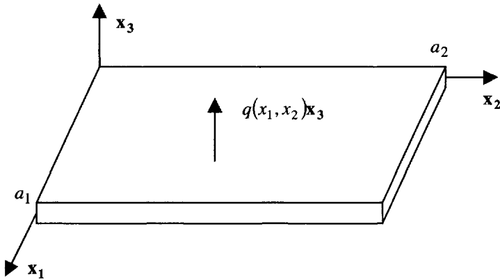
Figure 9.4. Asymmetrically balanced plate in flexure
