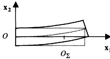
Figure 13.2. Beam element deformed in the plane ( O|x_1, x_2 )
