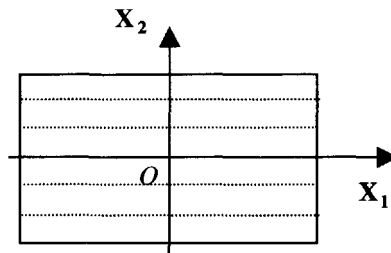
Figure 2.1. Orthotropic axes
