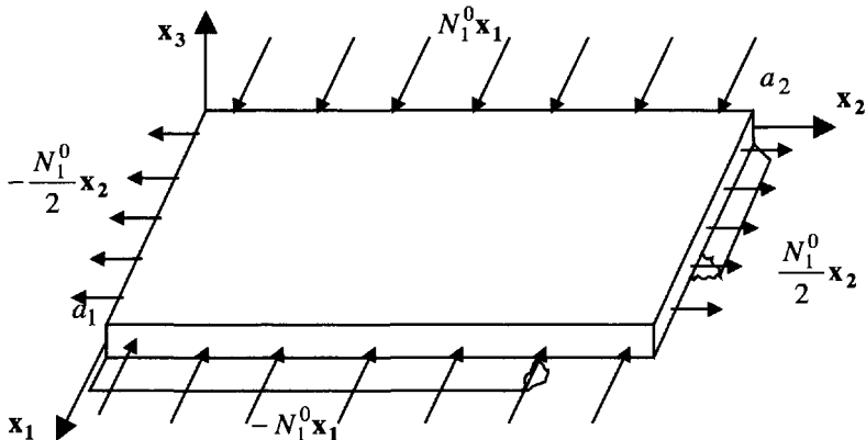
Figure 6.16. Compression and tension loads
