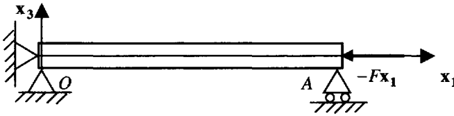
Figure 14.2. Beam buckling
