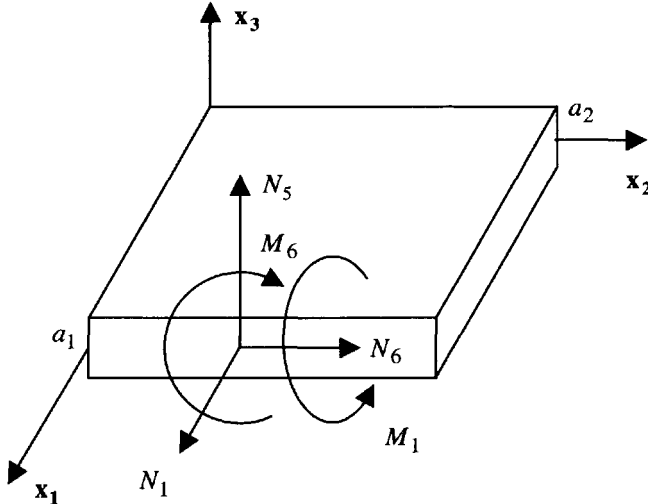
Figure 5.9. Loading boundary conditions
