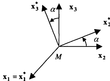
Figure 1.4. Isotropic plane
