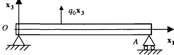
Figure 14.1. Beam subjected to a sinusoidal load
