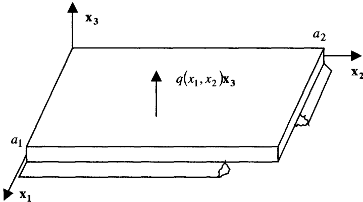
Figure 6.1. Transversely loaded plate
