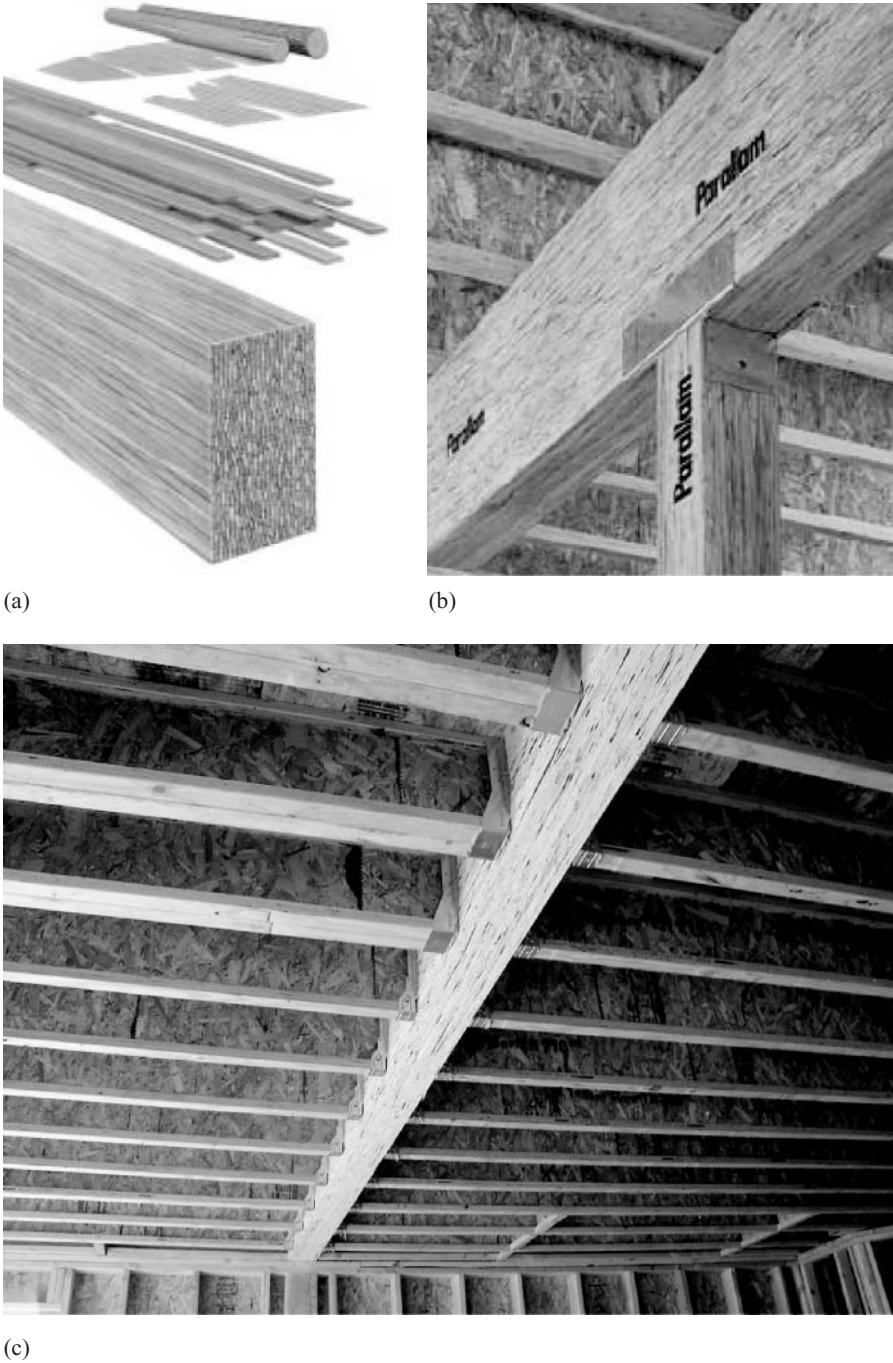
Fig. 1.13. Parallam (PSL) – manufacturing process and in construction; photos (a) and (b) courtesy of Weyerhaeuser (iLevel TrusJoist).
