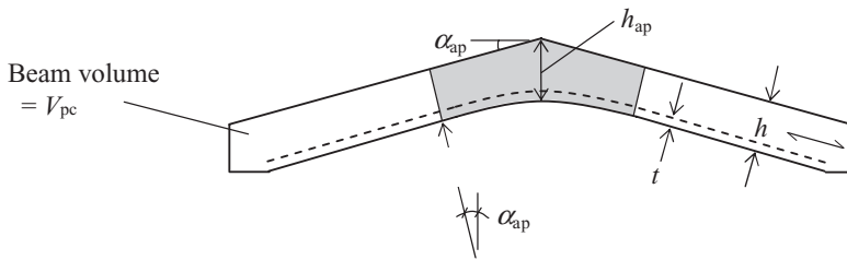
(c) Pitched cambered beam
