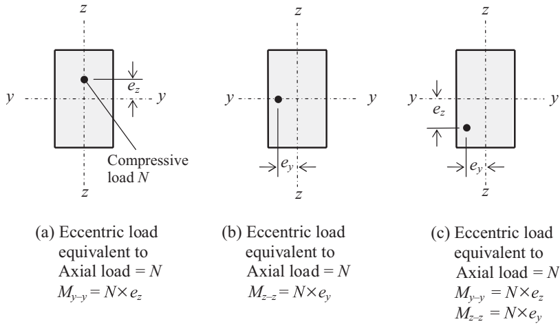
Fig. 5.9. Eccentric loading.
