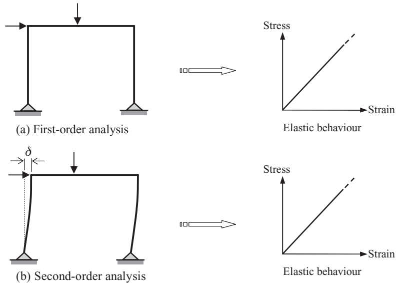
Fig. 2.1. First- and second-order linear elastic analysis.
