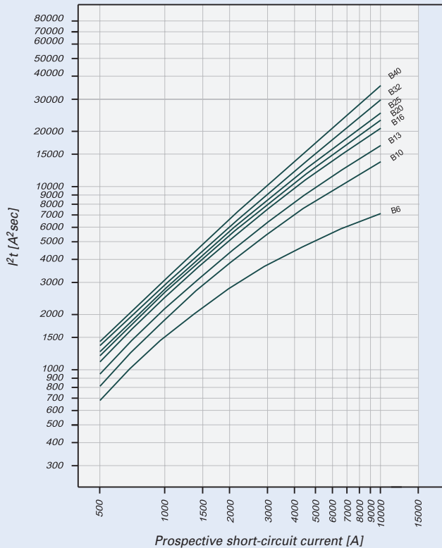
Let-through energy I^2t PFL7, characteristic B, 1+N-pole
