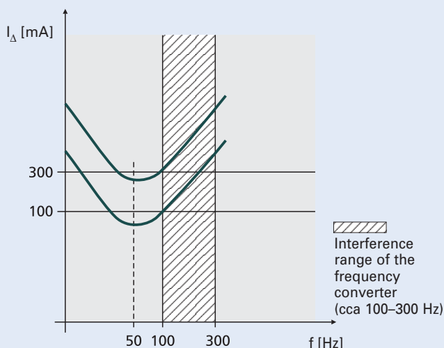
Tripping characteristic
