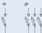
Connection diagram
