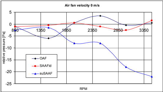
Figure 51. Values for pressure intake port 1, without vehicle movement simulation
