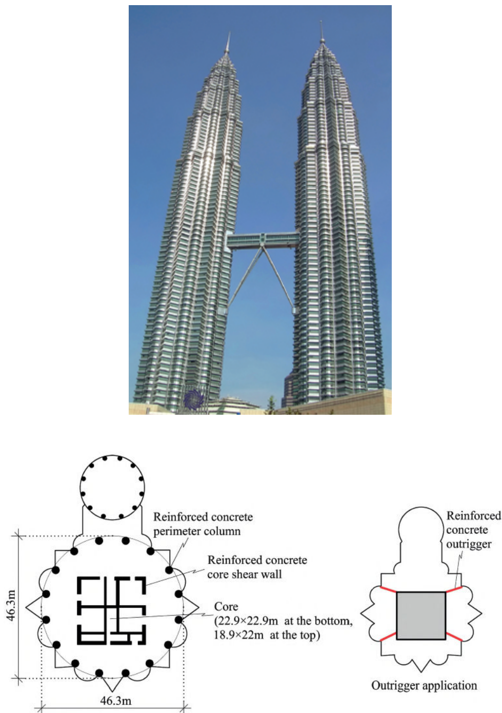
FIGURE 3.31 The Petronas Twin Towers, Kuala Lumpur, Malaysia, 1998
