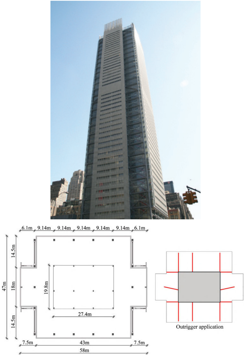
FIGURE 3.43 New York Times Tower, New York, USA, 2007 (photo courtesy of Antony Wood/CTBUH and plan courtesy of Ilkay Guryay)
