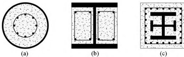
FIGURE 3.2 Composite elements by cross-section
