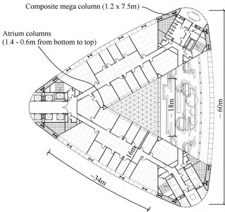
FIGURE 4.37 Commerzbank Tower plan
