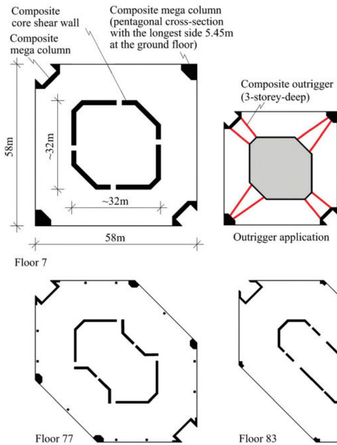
FIGURE 4.15 SWFC plans
