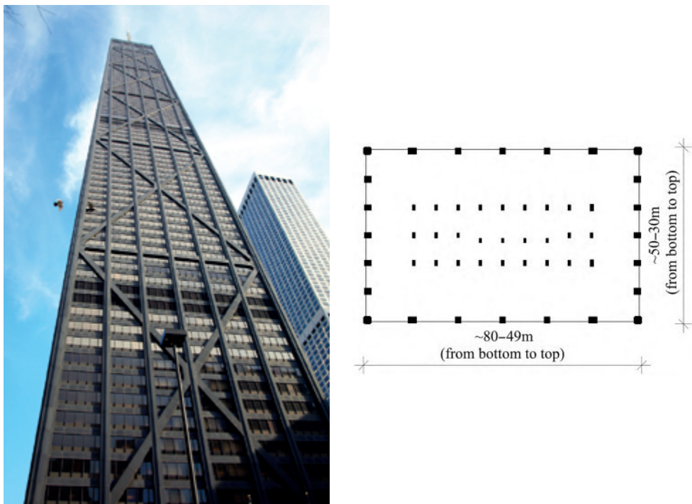
FIGURE 3.67 John Hancock Center, Chicago, USA, 1969 (photo courtesy of Marshall Gerometta / CTBUH)
