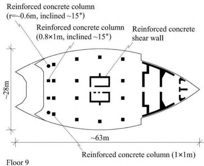
FIGURE 4.5 BWTC plan
