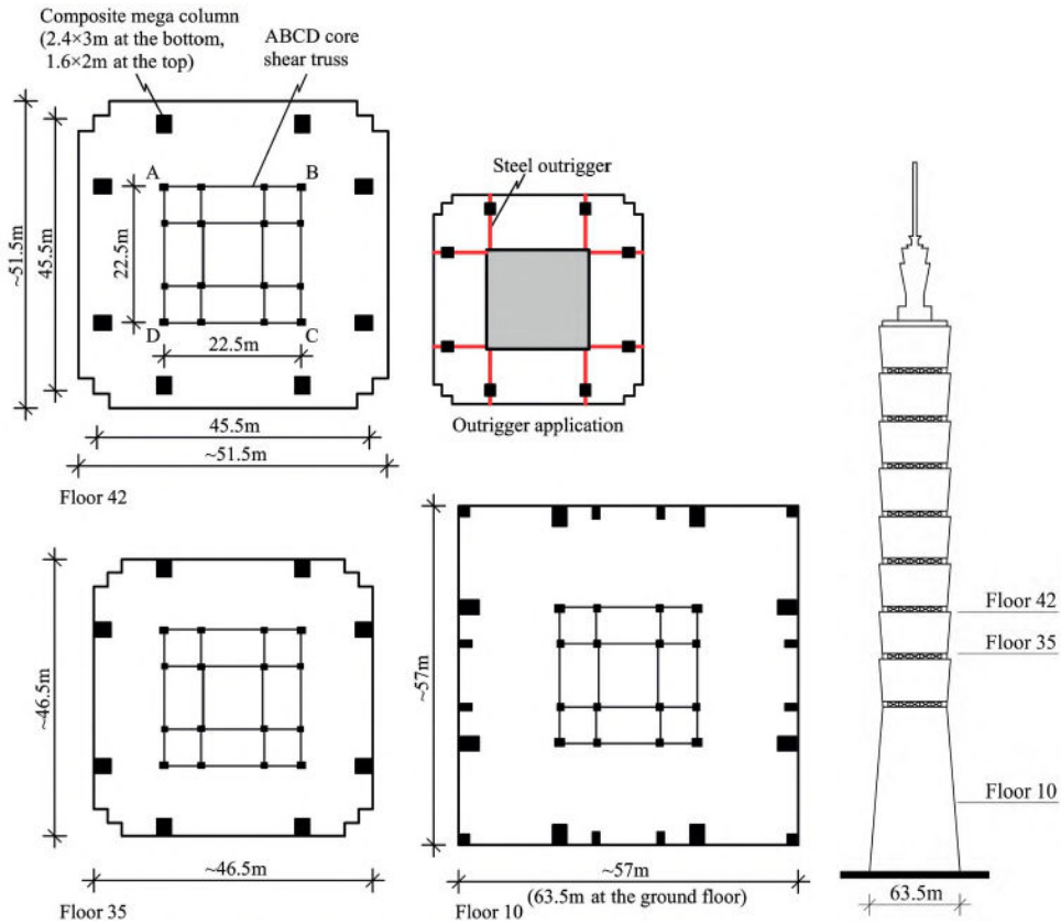
FIGURE 4.13 Taipei 101 schematic section and plans
