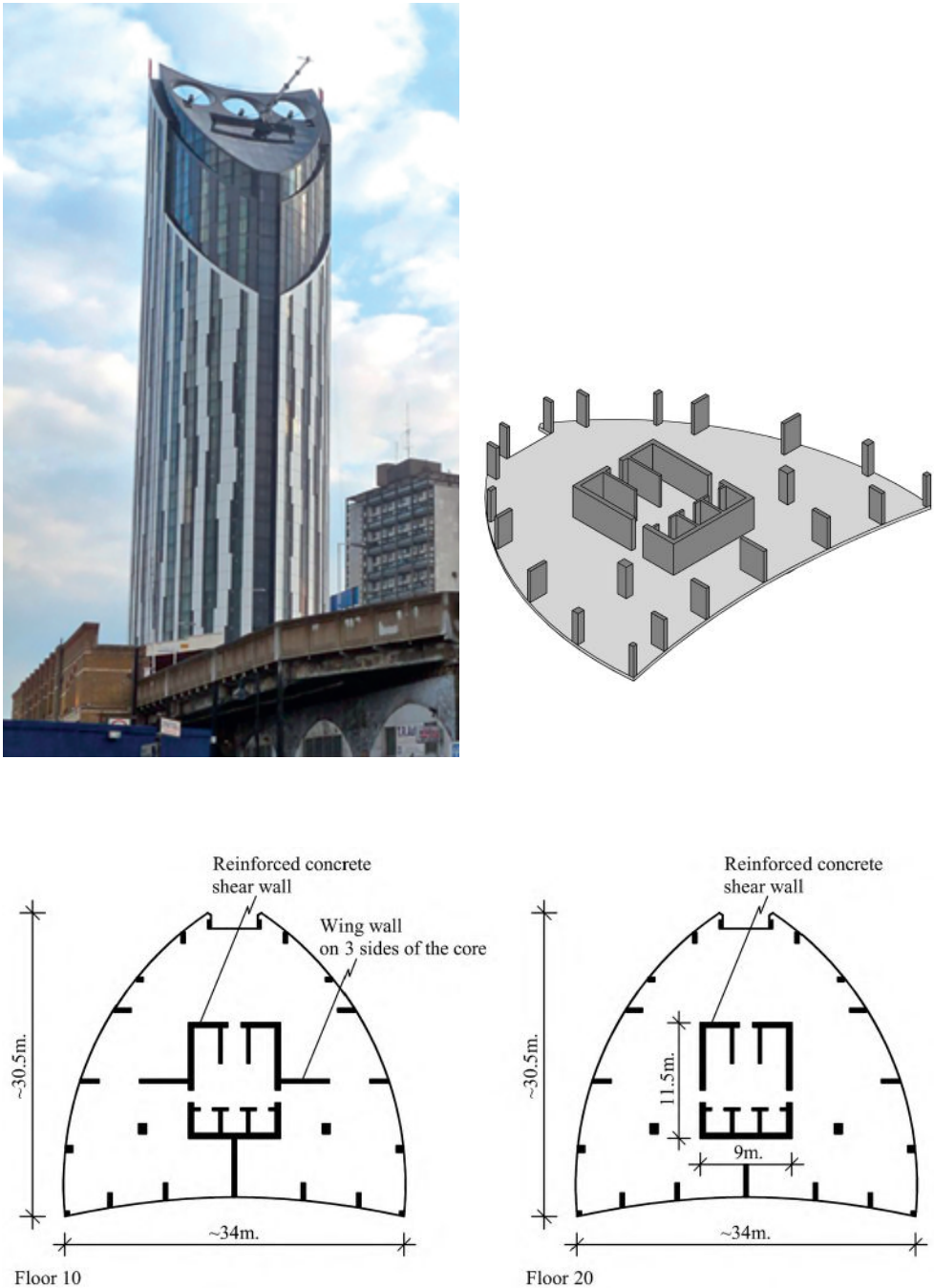
FIGURE 3.20 Strata, London, UK, 2010
