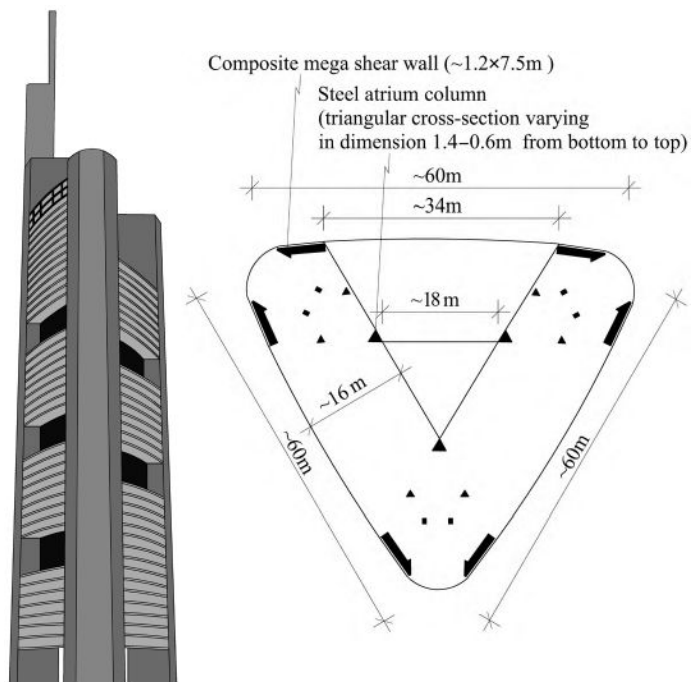
FIGURE 3.23 Commerzbank Tower, Frankfurt, Germany, 1997
