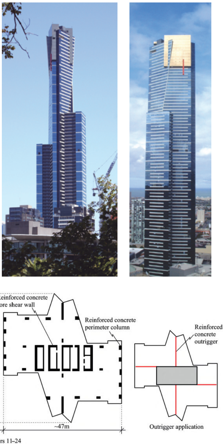
FIGURE 3.33 Eureka Tower, Melbourne, Australia, 2006 (photos courtesy of David Randerson)
