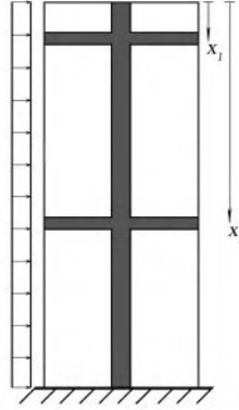
FIGURE 3.51 Location of two outrigger levels at distances x_1 and x_2 from the top
