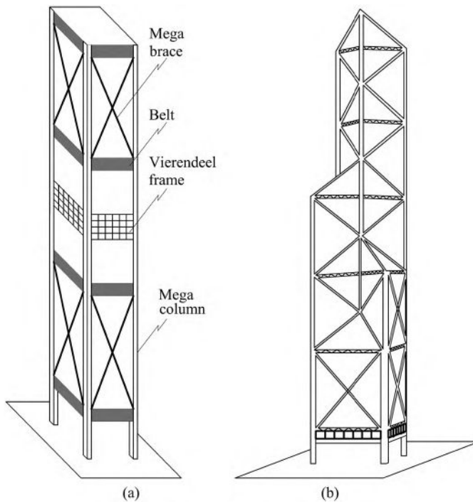
FIGURE 3.21 Mega column (mega frame, space truss) system
