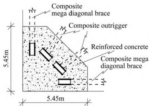
FIGURE 4.17 SWFC composite mega column section
