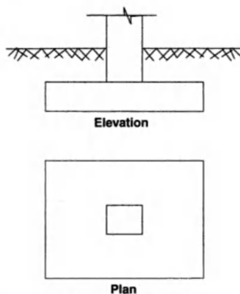
Figure 13.2 Spread footing
