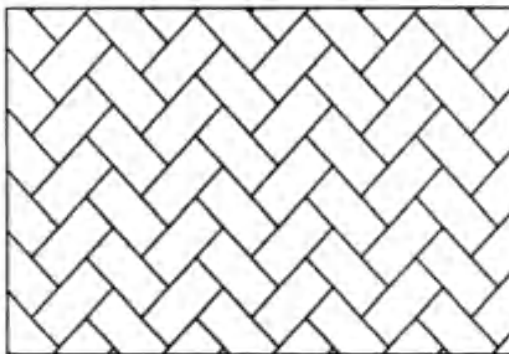
Figure 15.19 Zigzag bond
