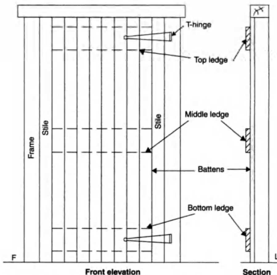
Figure 17.3 Battened, ledged and framed door
