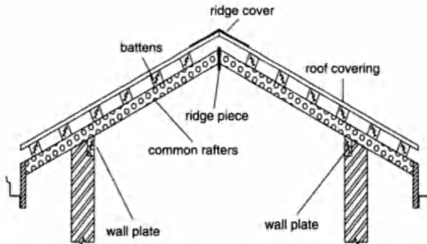
Figure 18.2 Couple roof
