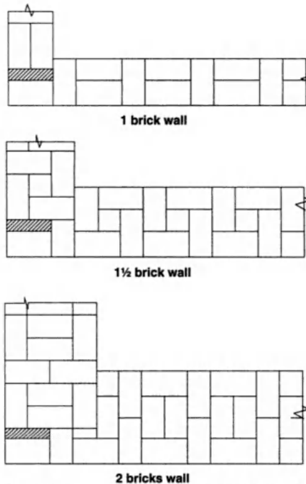
Figure 15.14 Courses 2, 4, 6, etc. of double Flemish bond
