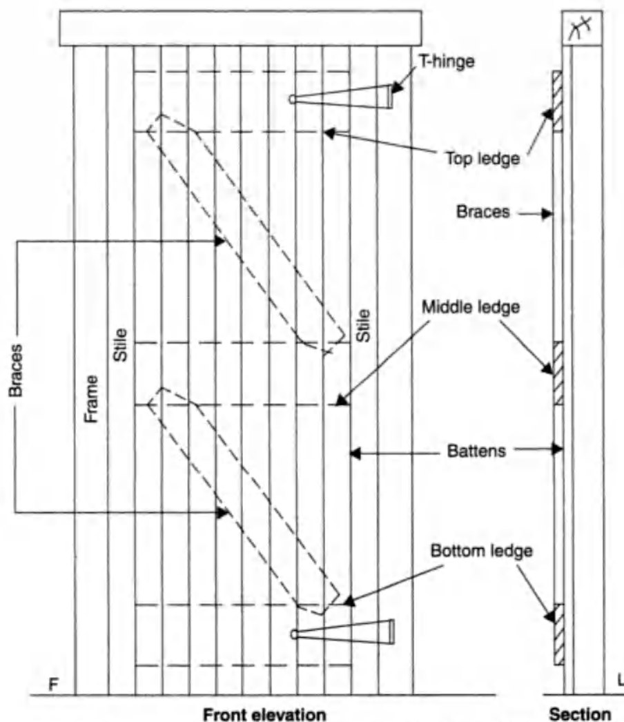
Figure 17.2 Battened, ledged and braced door
