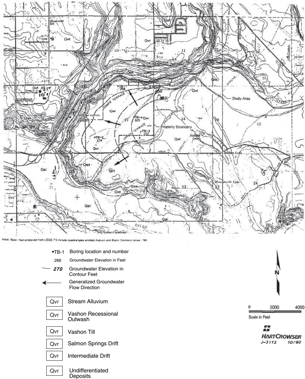
Figure 5-9 Map of groundwater elevation and surficial geology. Source: R. W. Thorpe and Associates.
