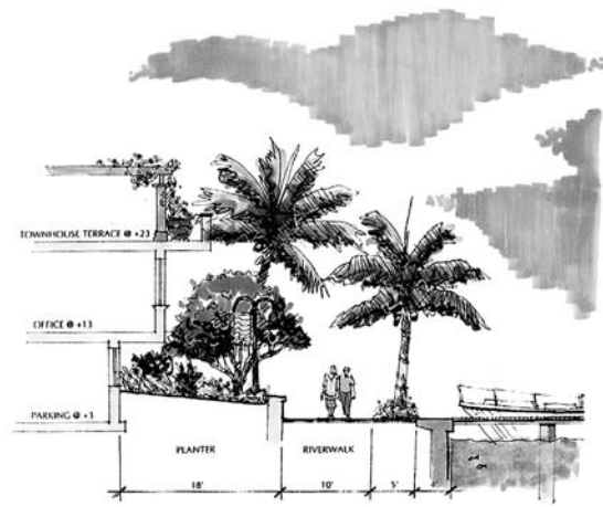
SECTION @ BLDG. ON NEW RIVER VIEW LOOKING NORTH SCALE: 3/16"=1'-0"
