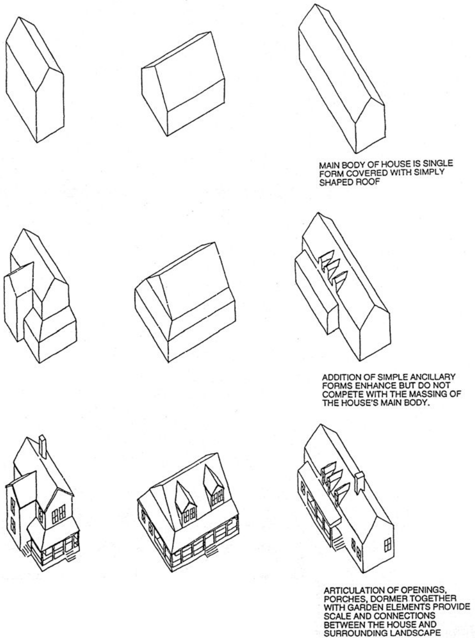
Figure 8-26 Design guidelines and illustrations showing examples of desired building massing and façade articulation. Source: Wallace Roberts & Todd, LLC, with Turnbull Griffin Haesloop Architects.
