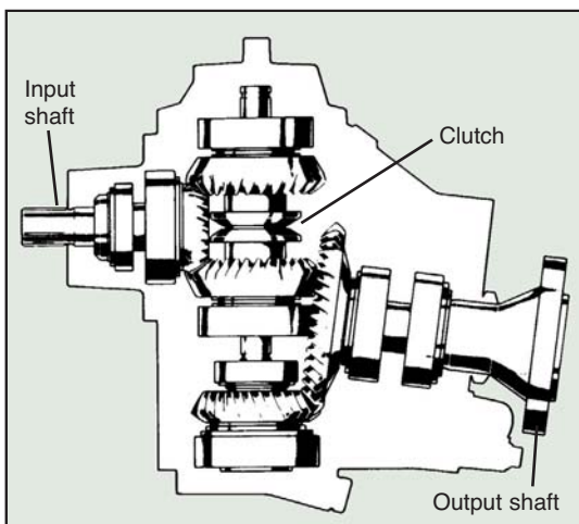
Fig 22 Volvo MS2 gear train.
