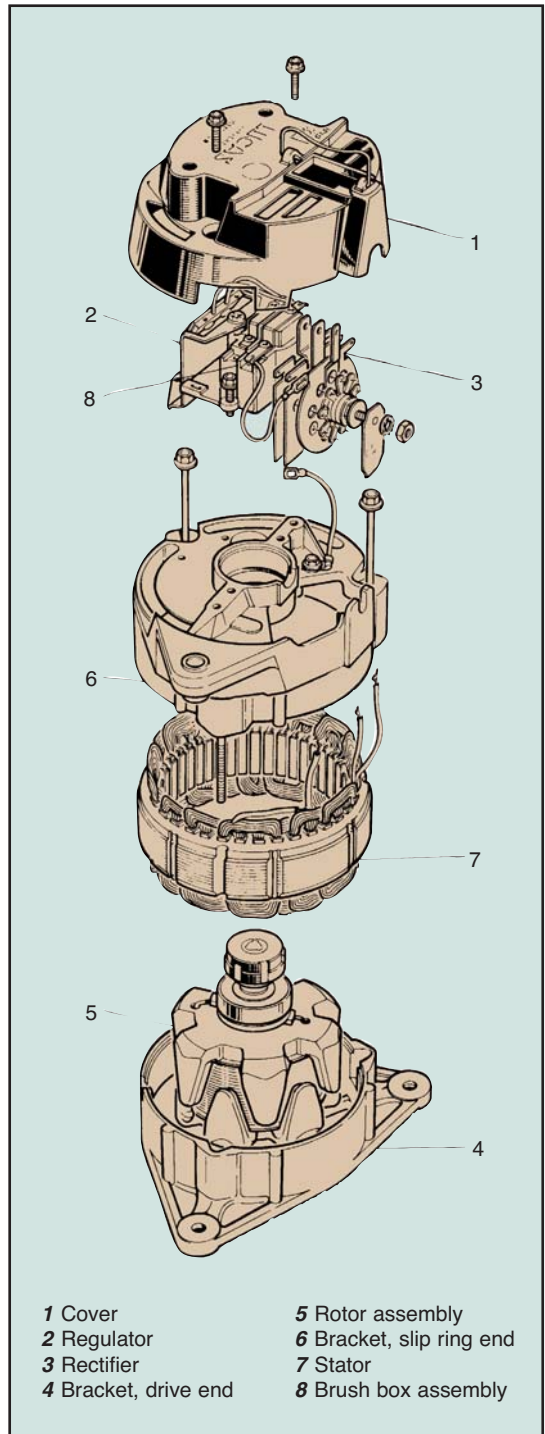
Fig 19 ACR alternator.
