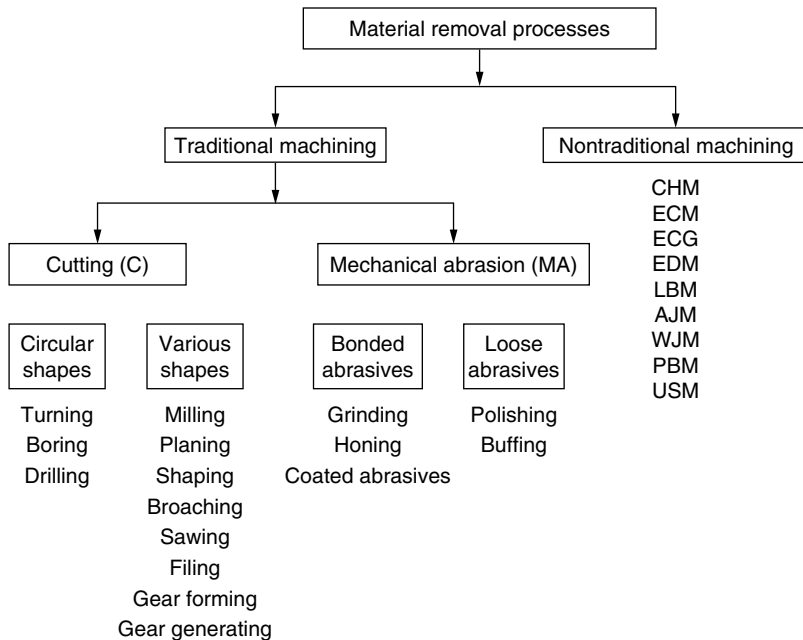
Figure 1.2 Material removal processes.
