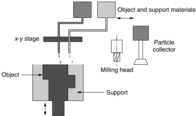
Figure 8.4 Liquid thermal polymerization.
