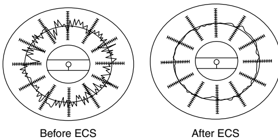
Figure 6.15 Effect of ECS on out-of-roundness profiles.
