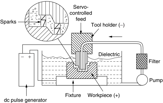
Figure 5.7 EDM schematic.
