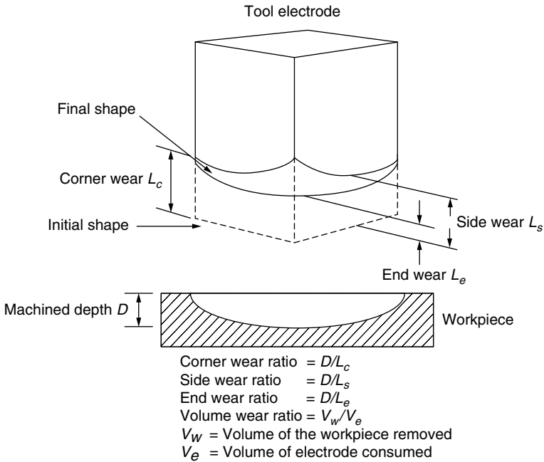
Figure 5.9 Types of electrode wear in EDM (Metals Handbook, 1989).
