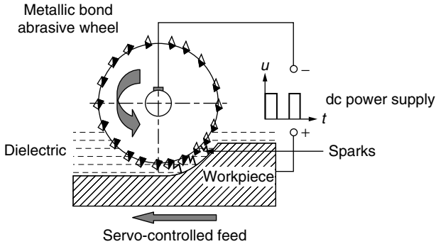
Figure 7.15 AEDG machining system components.
