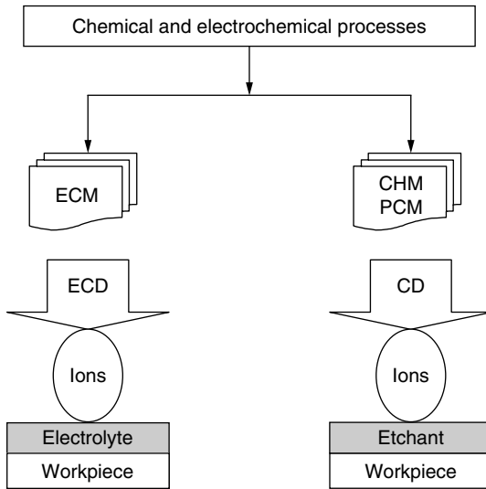
Figure 1.8 Electrochemical and chemical machining processes.
