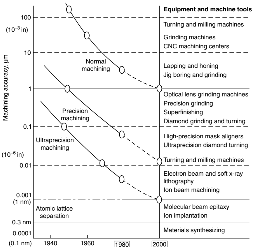
Figure 1.1 Machining accuracies (Tanigushi, 1983).
