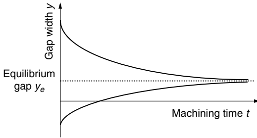
Figure 4.7 Attainment of equilibrium gap at a constant feed rate and various initial gaps.
