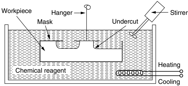
Figure 3.1 CHM setup.
