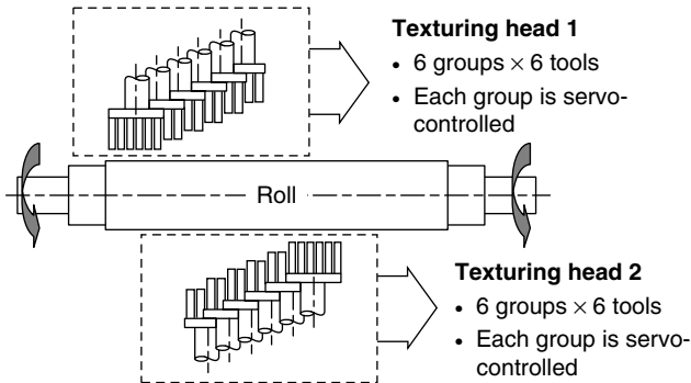
Figure 5.26 EDT machining system.
