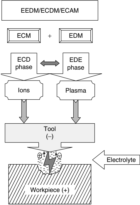
Figure 7.6 EEDM process components.
