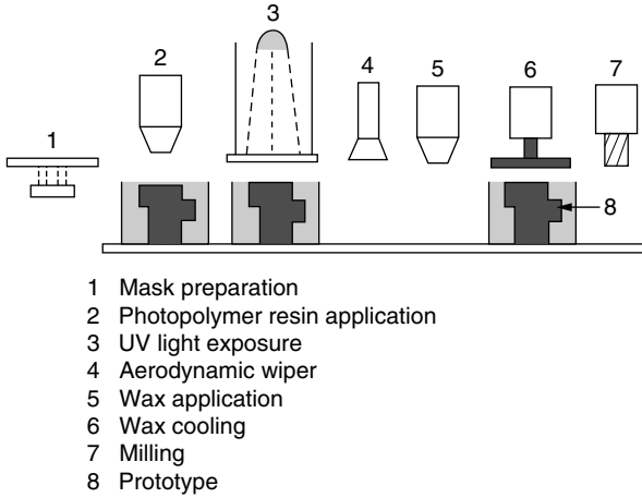
Figure 8.3 Solid ground curing steps.
