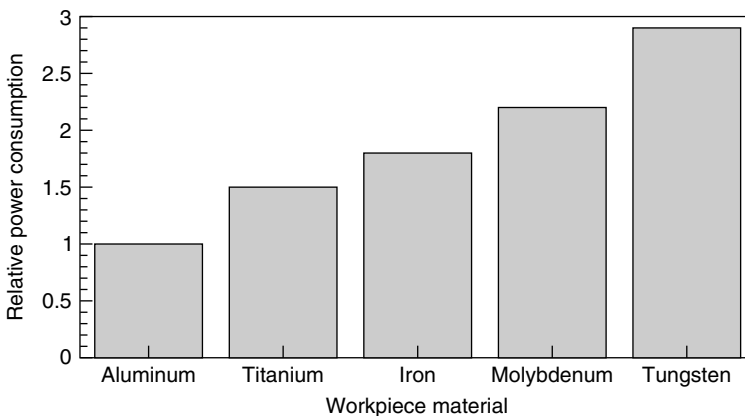
Figure 5.46 Relative power consumption for different materials (El-Hofy, 1995).
