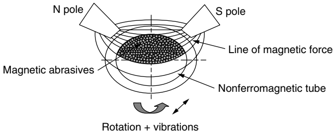
Figure 2.32 Magnetic finishing of nonmagnetic tubes.
