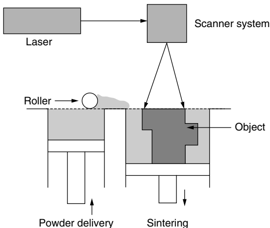
Figure 8.10 Selective laser sintering.
