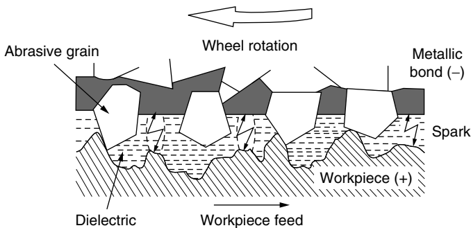
Figure 7.16 Material removal mechanisms in AEDG.
