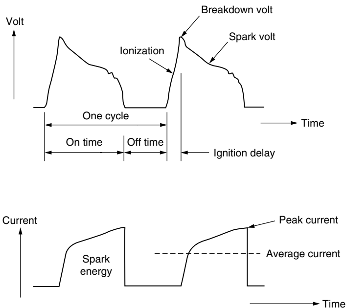
Figure 5.4 Voltage and current waveforms during EDM.
