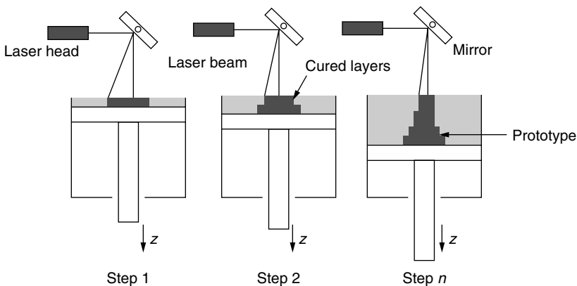
Figure 8.1 Principles of stereolithography.
