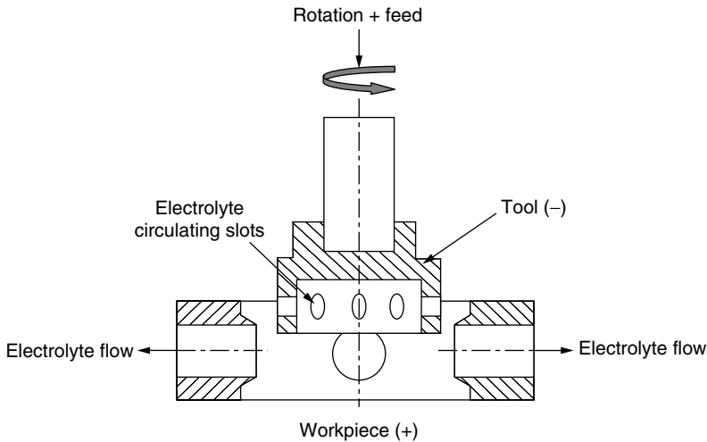
Figure 4.32 Electrochemical deburring using a rotating tool.
