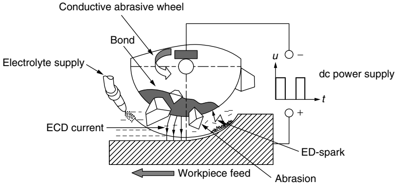
Figure 7.22 ECDG schematic diagram.
