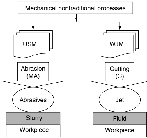
Figure 1.6 Mechanical machining processes.
