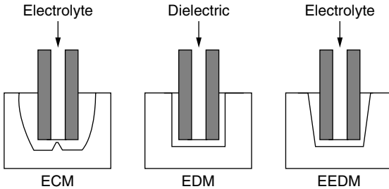
Figure 7.11 Holes drilled by ECM, EDM, and EEDM.
