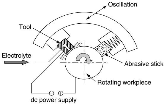
Figure 6.11 Superfinishing using separate EC electrode (Youssef, 1971).
