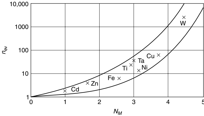
Figure 5.45 The number of pulses required (vertical) versus the relative machinability index (Kaczmarek, 1976).
