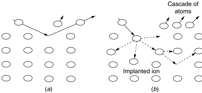
Figure 5.57 Mechanism of material removal at (a) low and (b) high energy levels (McGeough, 1988).
