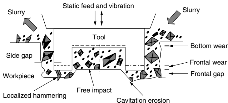
Figure 2.10 Material removal mechanisms in USM (Thoe et al., 1995).
