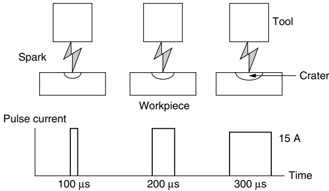
Figure 5.15 Effect of pulse on-time (energy) on removal rate and surface roughness.
