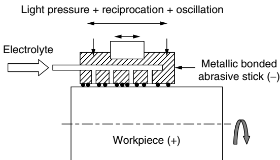
Figure 6.12 ECS using metallic bond diamond stick (Youssef, 1971).
