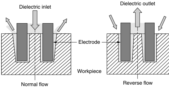
Figure 5.11 Common dielectric flushing modes.
