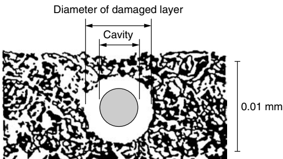
Figure 5.47 Cross section of cavity by single EBM pulse in chromium molybdenum steel (Kaczmarek, 1976).
