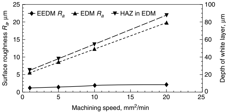
Figure 7.8 Effect of machining speed on the surface roughness and the damaged layer in EDM and EEDM.
