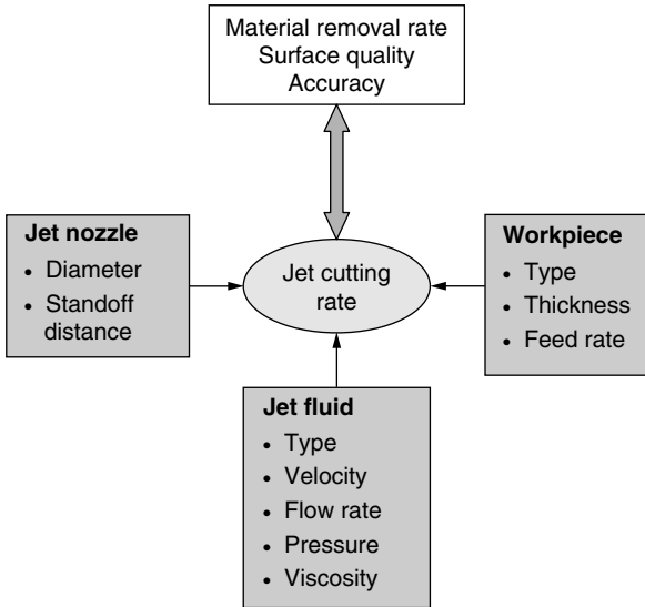
Figure 2.21 Factors affecting WJM performance.
