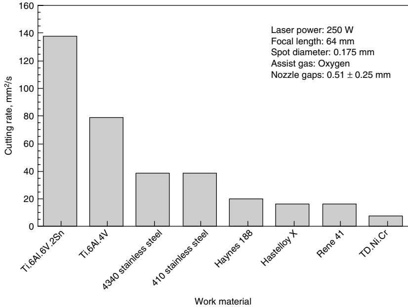
Figure 5.36 Machining speeds of aerospace alloys in gas-assisted LBM (El-Hofy, 1995).
