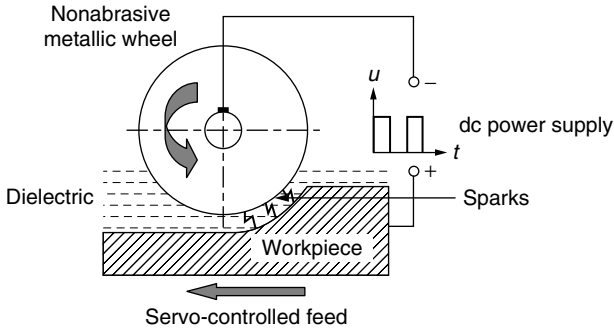
Figure 7.12 EDG schematic.
