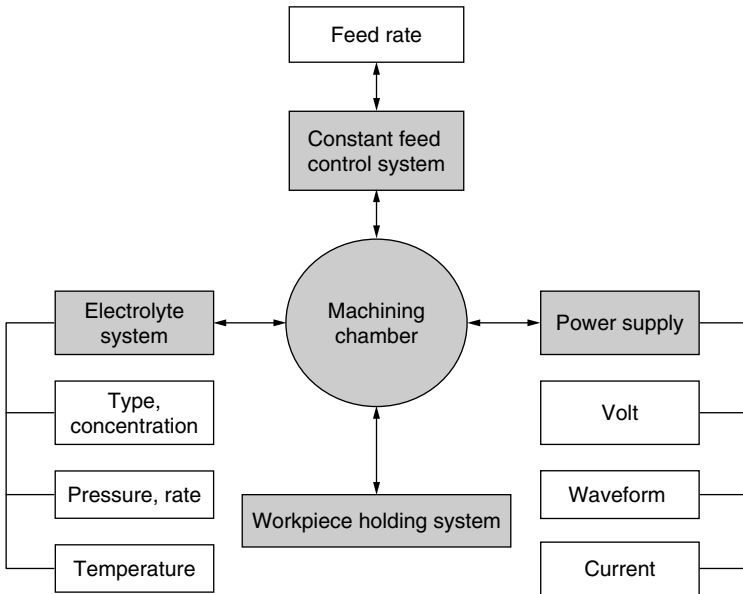
Figure 4.3 ECM system components.
