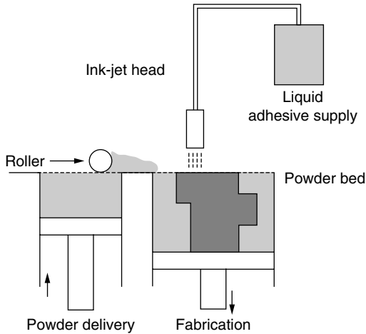
Figure 8.12 Three-dimensional printing.
