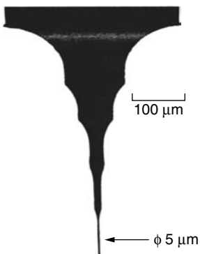
Figure 5.28 Micropin produced by WEDG (Masuzawa and Tonshof, 1997).
