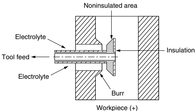
Figure 4.31 Hole deburring.
