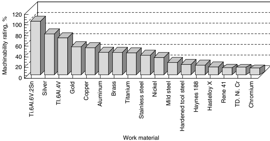
Figure 5.35 Machinability of some materials in LBM (El-Hofy, 1995).
