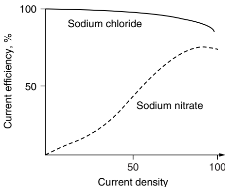
Figure 4.4 Effect of current density on current efficiency for different electrolytes.
