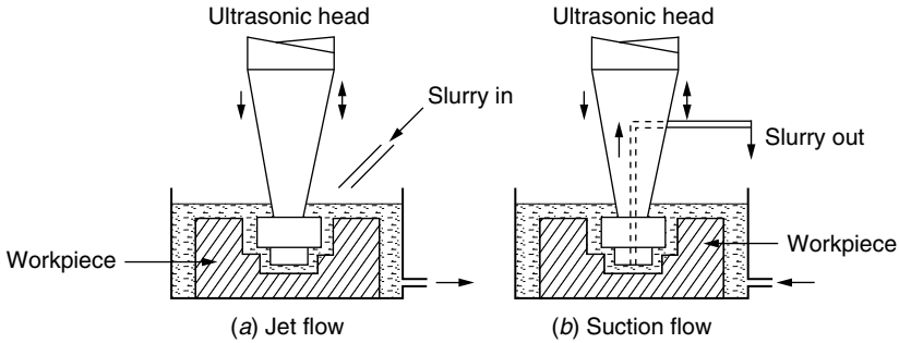
Figure 2.9 Slurry injection methods.
