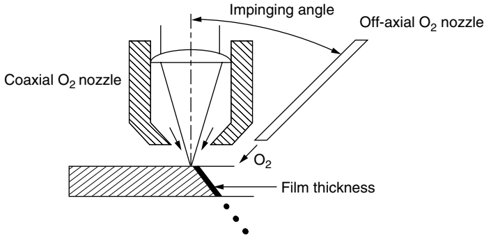
Figure 5.39 Off-axis gas-assisted laser cutting (Hsu and Molian, 1995).
