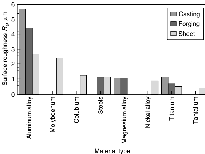
Figure 3.6 CHM average roughness of some alloys after removing 0.25 to 0.4 mm (El-Hofy, 1995).
