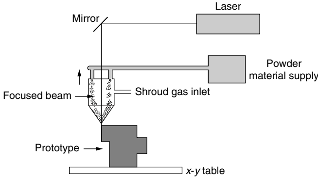
Figure 8.11 LENS process.
