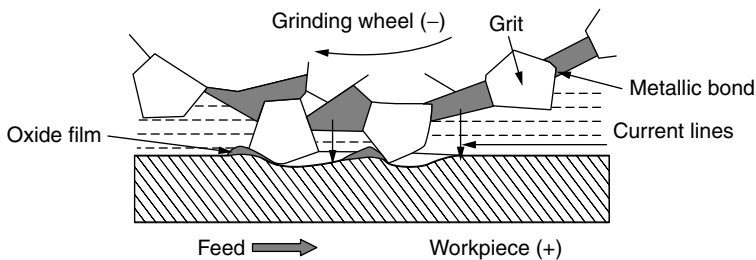
Figure 6.5 ECD and MA in the machining gap during ECG.
