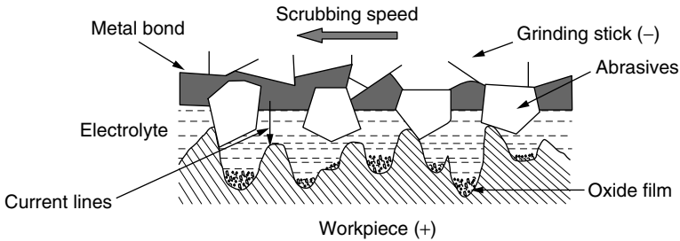
Figure 6.13 Metal removal mechanisms in ECG.
