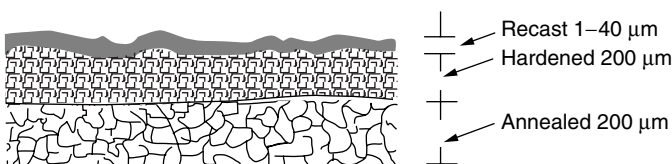
Figure 5.16 EDM heat-affected zones.
