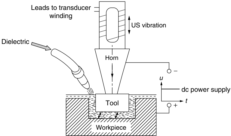
Figure 7.20 EDMUS schematic.
