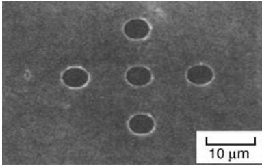
Figure 5.29 Microholes produced by EDM (Masuzawa and Tonshof, 1997).
