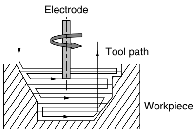
Figure 5.19 EDM die milling.
