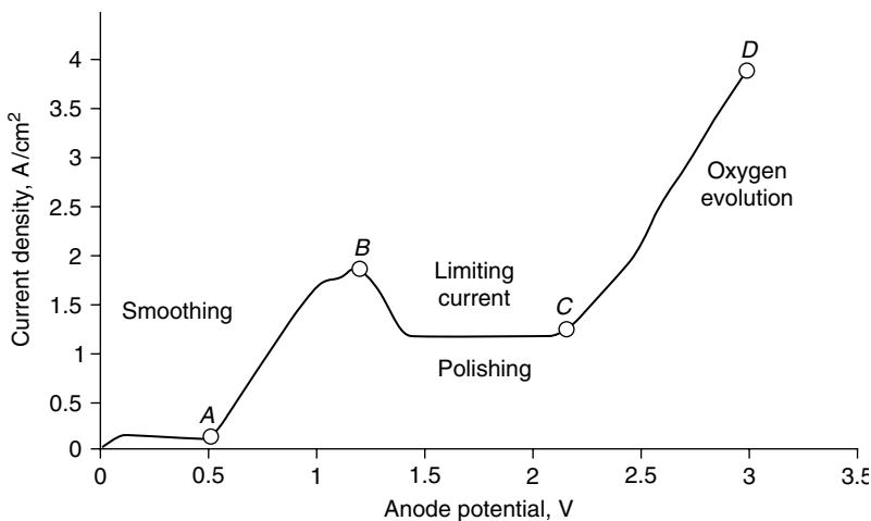
Figure 3.14 Current density and anode potential during the EP process.
