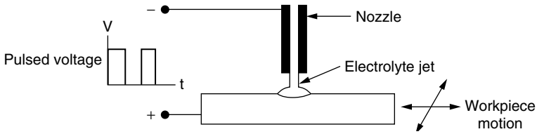
Figure 4.18 Electrolyte jet ECM.
