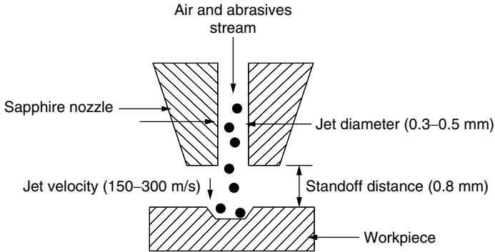
Figure 2.25 AJM terminology.
