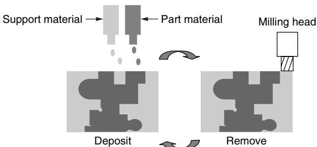
Figure 8.9 Shape deposition manufacturing.
