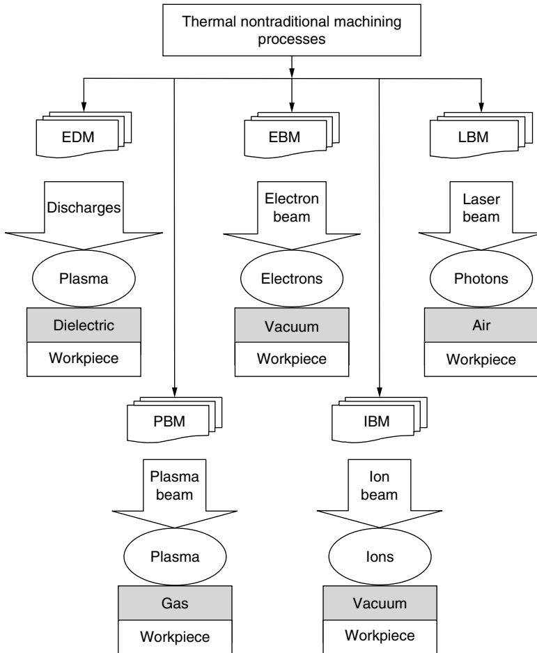
Figure 1.7 Thermal nonconventional processes.
