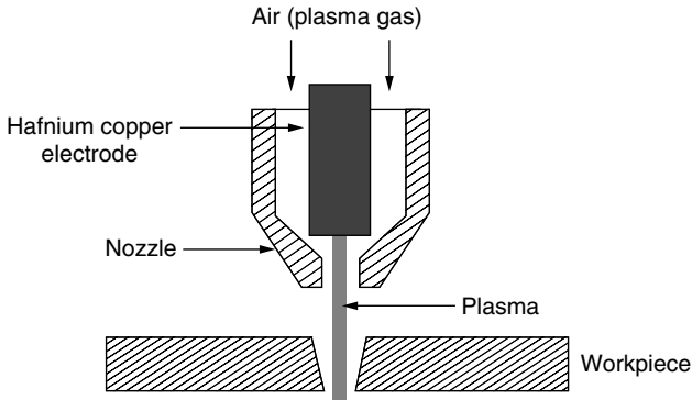
Figure 5.52 Air plasma.
