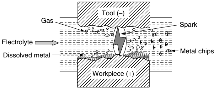
Figure 7.7 Surface formations in EEDM (El-Hofy and Khayry, 1995).
