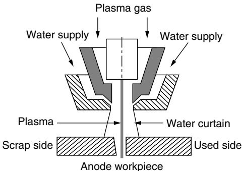
Figure 5.51 Water-shielded plasma.
