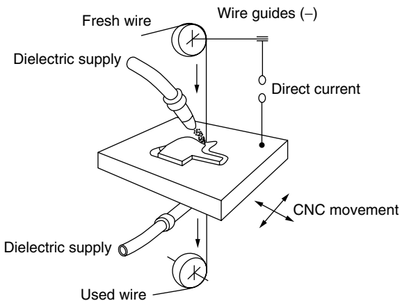
Figure 5.23 Wire EDM schematic.
