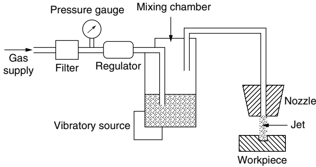
Figure 2.24 AJM system.
