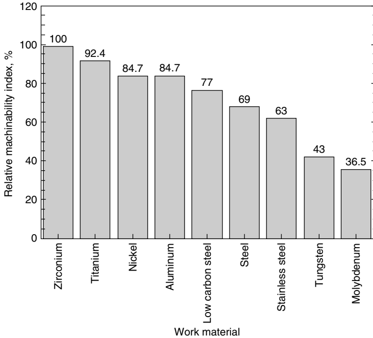
Figure 4.11 Relative machinability for different materials at constant current density (El-Hofy, 1995).
