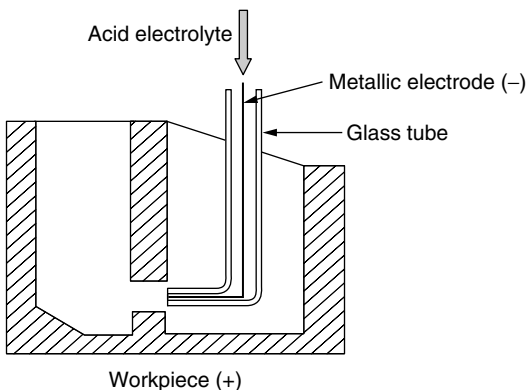
Figure 4.27 ES drilling in inaccessible positions.
