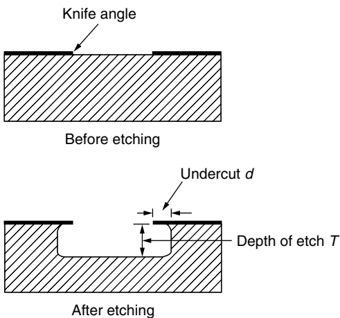
Figure 3.2 Etch factor after CHM.
