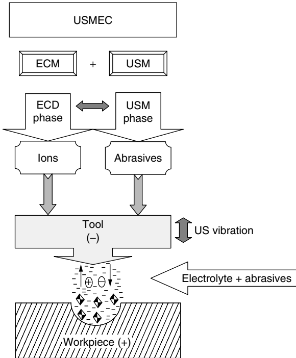
Figure 6.19 USMEC components.
