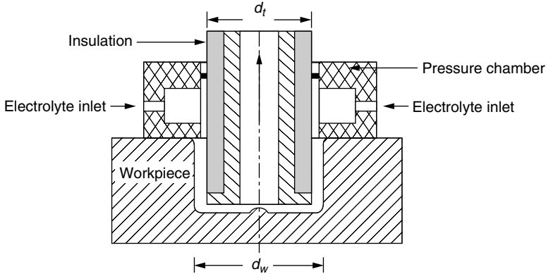
Figure 4.22 Hole drilling using back pressure.
