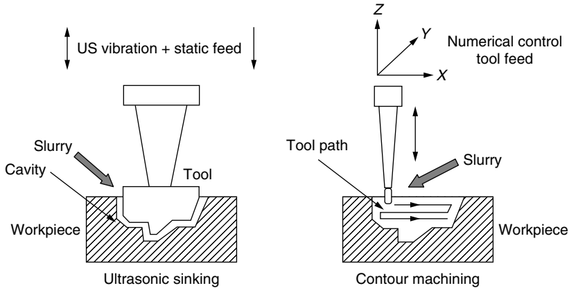
Figure 2.13 Ultrasonic sinking and contour machining.
