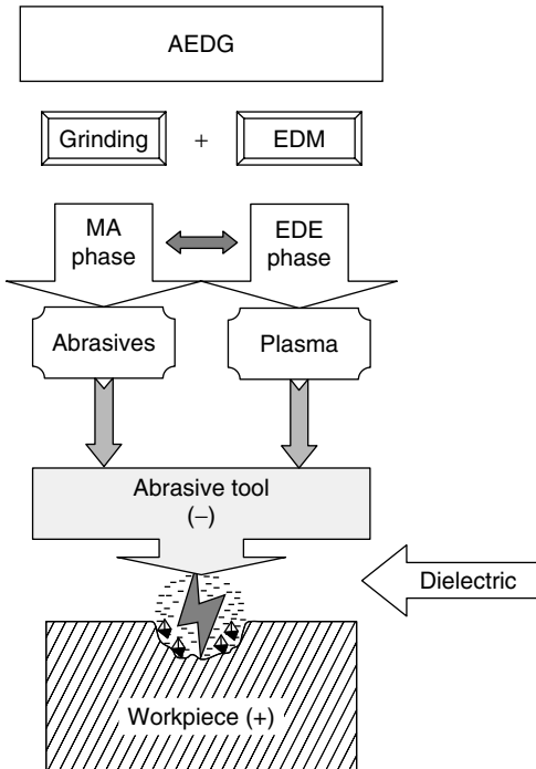
Figure 7.17 Elements of AEDG.
