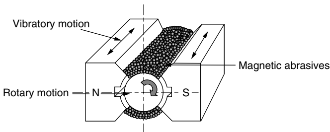
Figure 2.29 MAF schematic.
