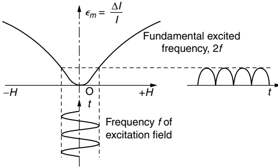
Figure 2.5 Magnetostrictor excited by a variable magnetic field without magnetizing (Kaczmarek, 1976).
