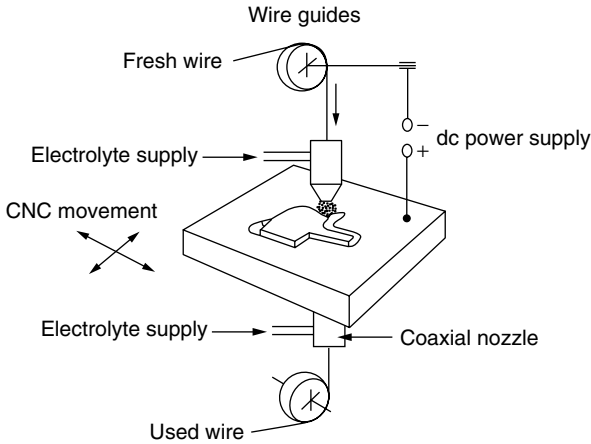
Figure 7.2 Electroerosion dissolution wire machining.
