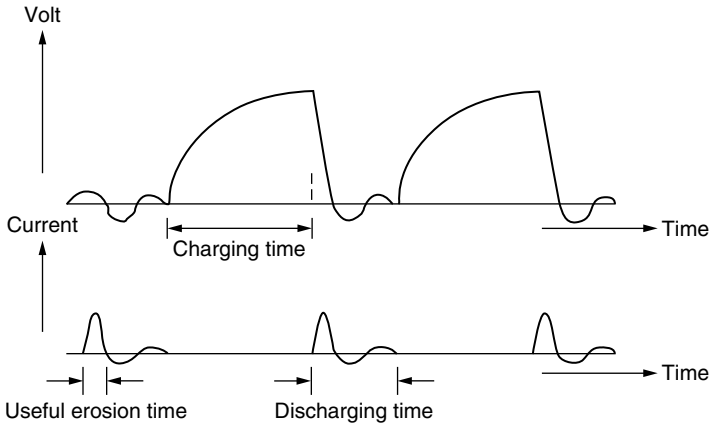
Figure 5.6 Periodic discharges in RC-type generator.
