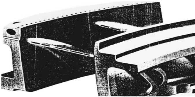
Figure 5.38 Cooling holes in turbine vane (Corfe, 1983).
