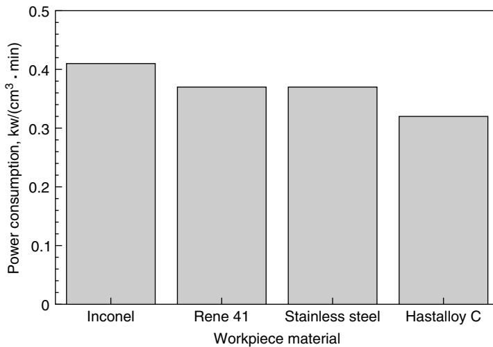
Figure 5.54 Power consumption in plasma beam rough turning (El-Hofy, 1995).
