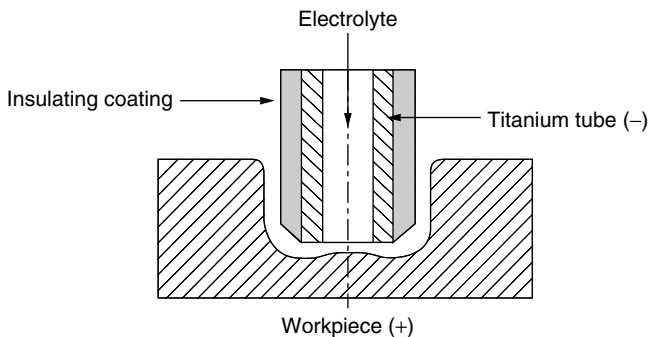
Figure 4.23 STEM schematic.
