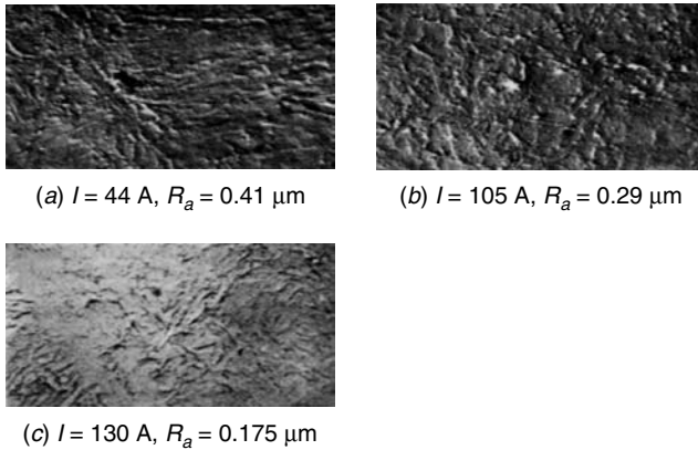
Figure 4.15 The appearance of different ECM surfaces at various currents for NC6 heat-treated tool steel (Kaczmarek, 1976).
