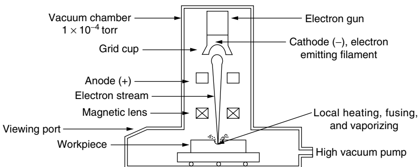
Figure 5.43 Components of an EBM system.
