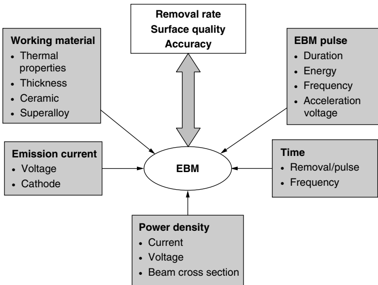
Figure 5.44 Parameters affecting EBM performance.
