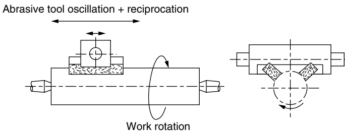
Figure 6.10 Vibratory superfinishing schematic.
