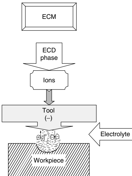
Figure 4.9 ECM process components.
