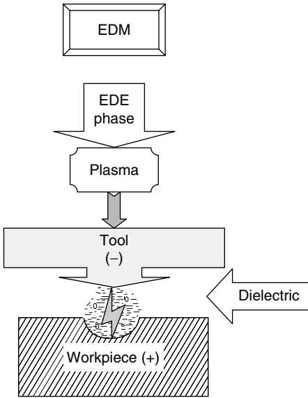
Figure 5.1 EDM components.
