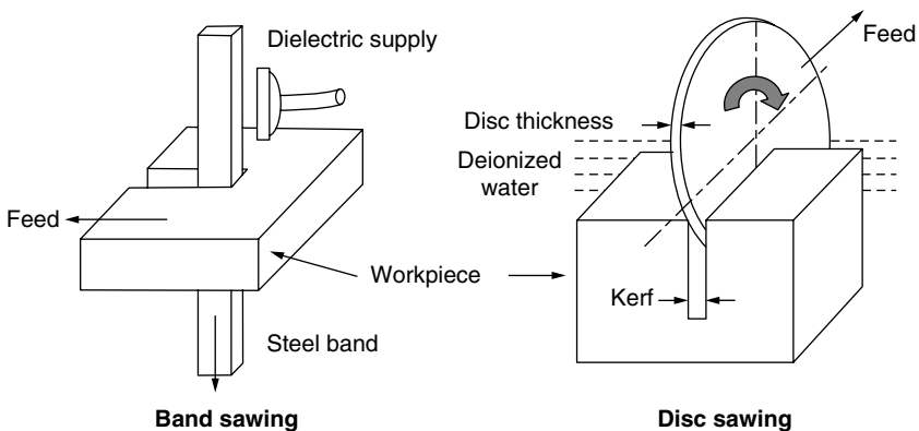
Figure 5.17 ED sawing schematic.
