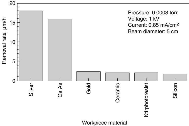
Figure 5.58 Removal rates for different materials (El-Hofy, 1995).
