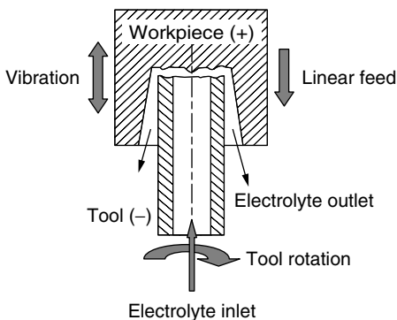
Figure 7.3 EEDM drilling.
