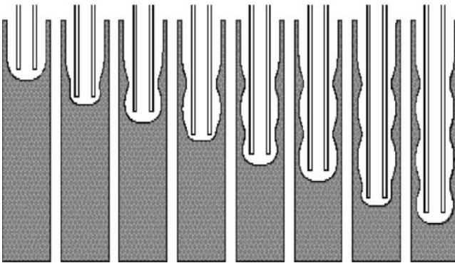
Figure 4.24 Turbulated cooling holes produced by STEM ( www.win.tue.nl/ ).
