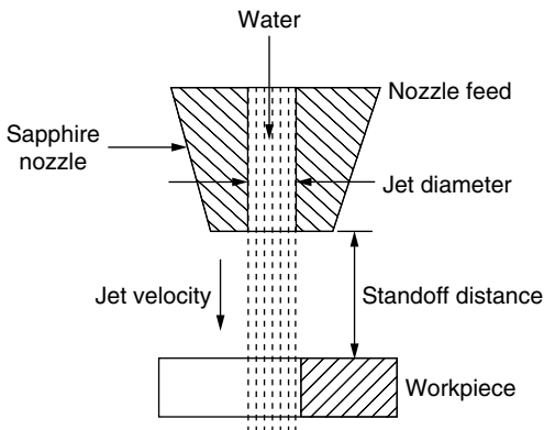
Figure 2.20 WJM terminology.
