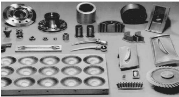
Figure 4.17 ECM components ( www.unl.edu/ ).
