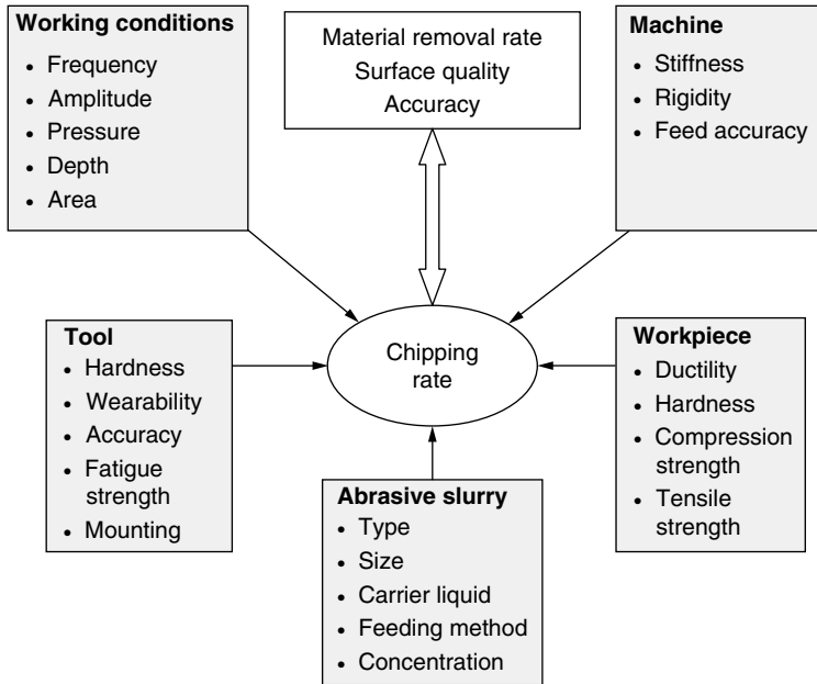
Figure 2.11 Factors affecting USM performance.
