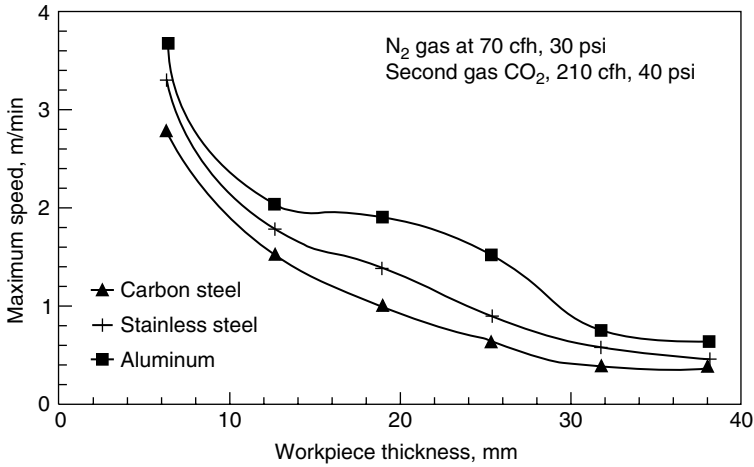
Figure 5.53 Machinability of different material in gas-shielded plasma (El-Hofy, 1995).
