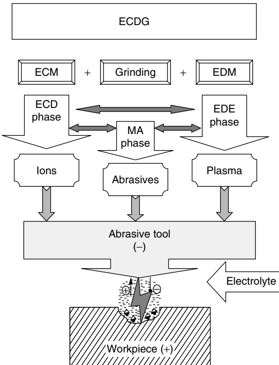
Figure 7.23 Material removal mechanisms in ECDG.
