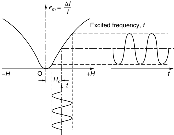
Figure 2.6 Magnetostriction due to a variable magnetic field after polarization (Kaczmarek, 1976).
