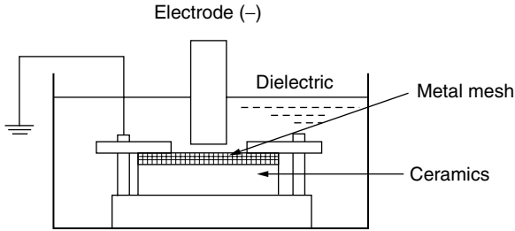
Figure 5.24 EDM of insulating ceramics (Fukuzawa et al., 1995).
