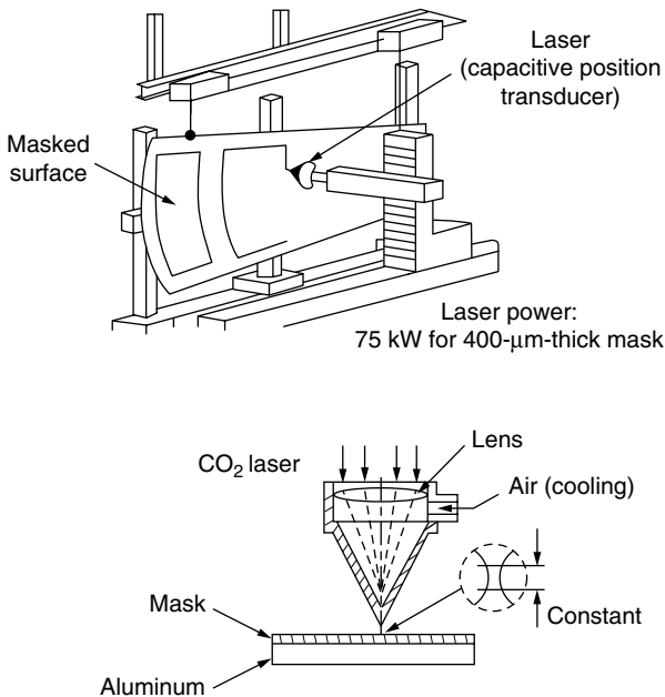
Figure 3.5 Laser cutting of masks for CHM of large surfaces (Thusty, 1999).
