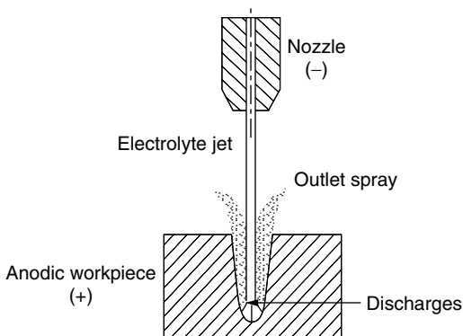
Figure 4.28 Electrochemical jet drilling.
