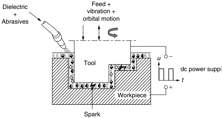
Figure 7.18 AEDM system.
