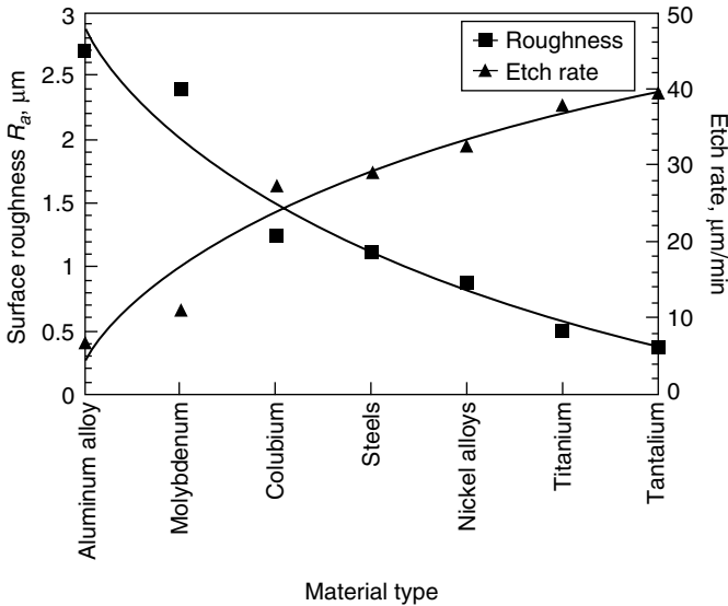
Figure 3.7 Surface roughness and etch rate of some alloys after removing 0.25 to 0.4 mm (El-Hofy, 1995).
