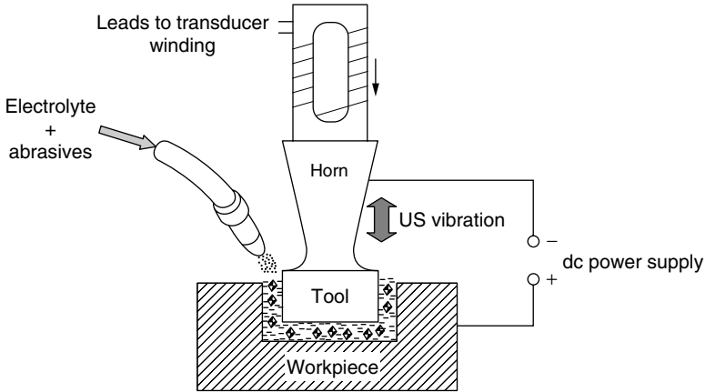
Figure 6.18 USMEC schematic.
