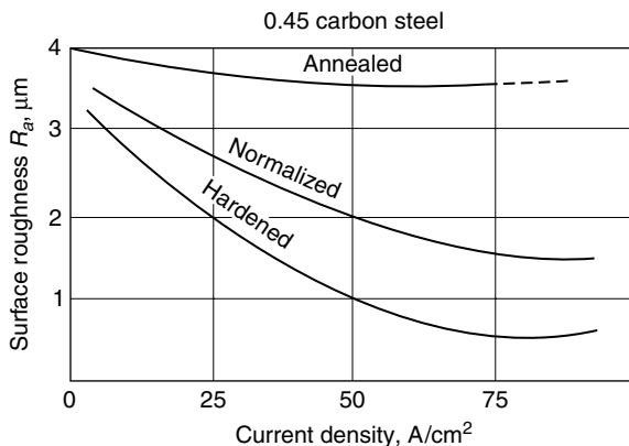
Figure 4.16 Effect of heat treatment on surface roughness for steel (Kaczmarek, 1976).
