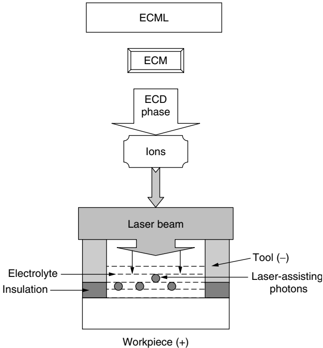
Figure 6.20 ECML schematic.
