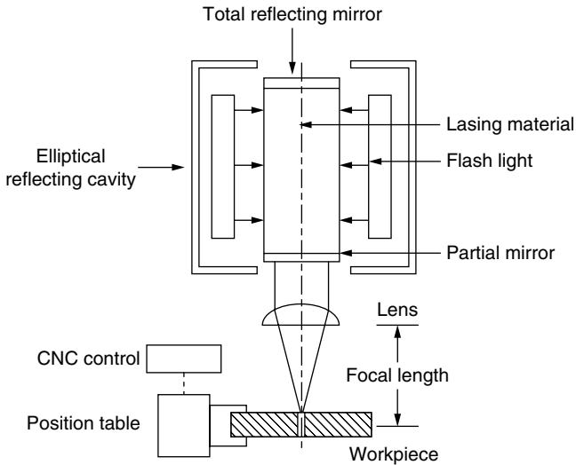
Figure 5.32 LBM schematic.
