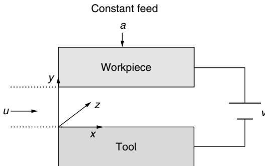
Figure 4.6 Working gap with plane-parallel electrodes at a constant gap voltage.
