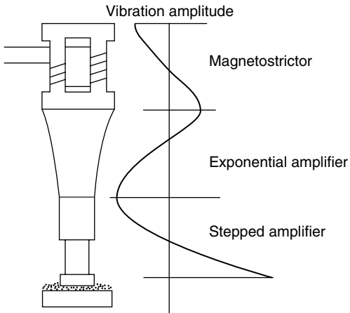
Figure 2.8 Two-step amplification in USM.
