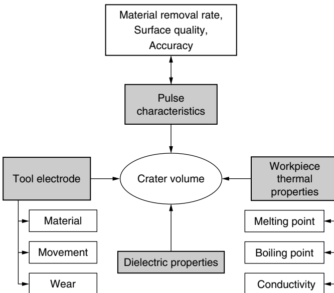
Figure 5.12 Parameters affecting EDM performance.
