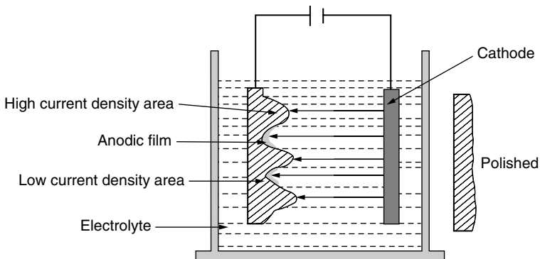
Figure 3.16 Electropolishing process.
