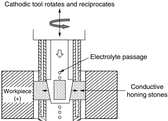
Figure 6.7 ECH schematic.
