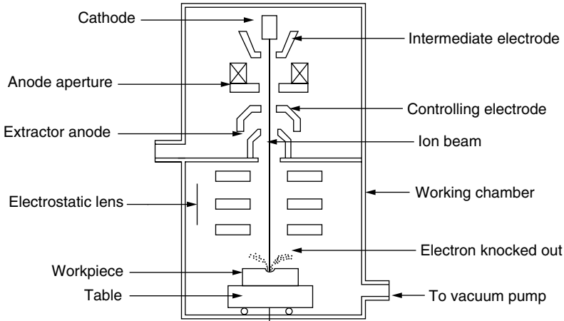
Figure 5.56 IBM system components.
