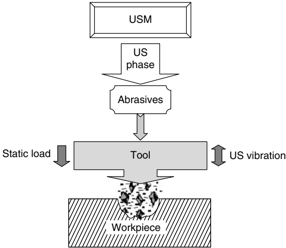
Figure 2.1 USM components.
