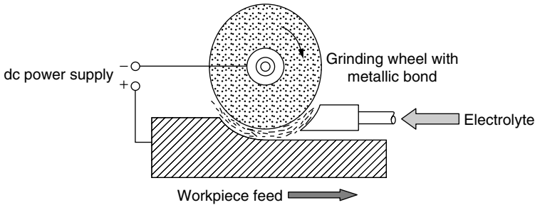
Figure 6.2 Surface ECG.
