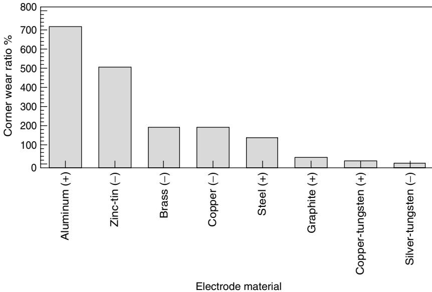
Figure 5.10 Corner wear ratios for different electrode materials (El-Hofy, 1995).
