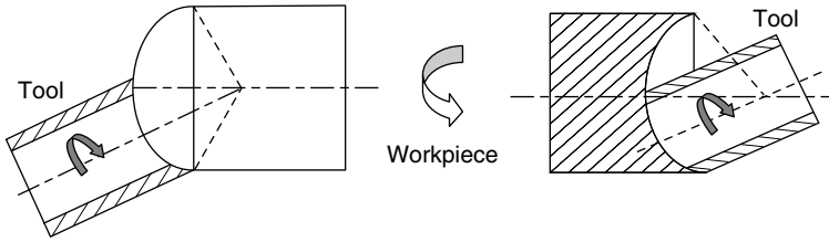
Figure 5.18 Rotary EDM.
