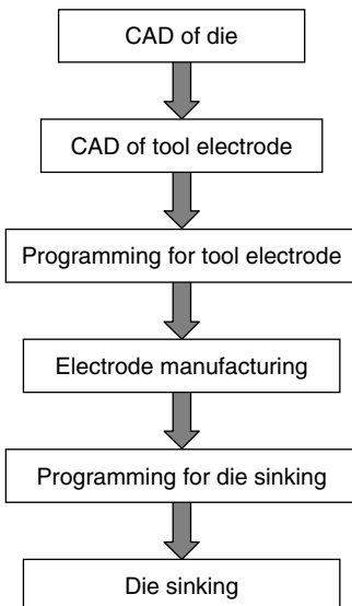
Figure 5.21 EDM die sinking flowchart.
