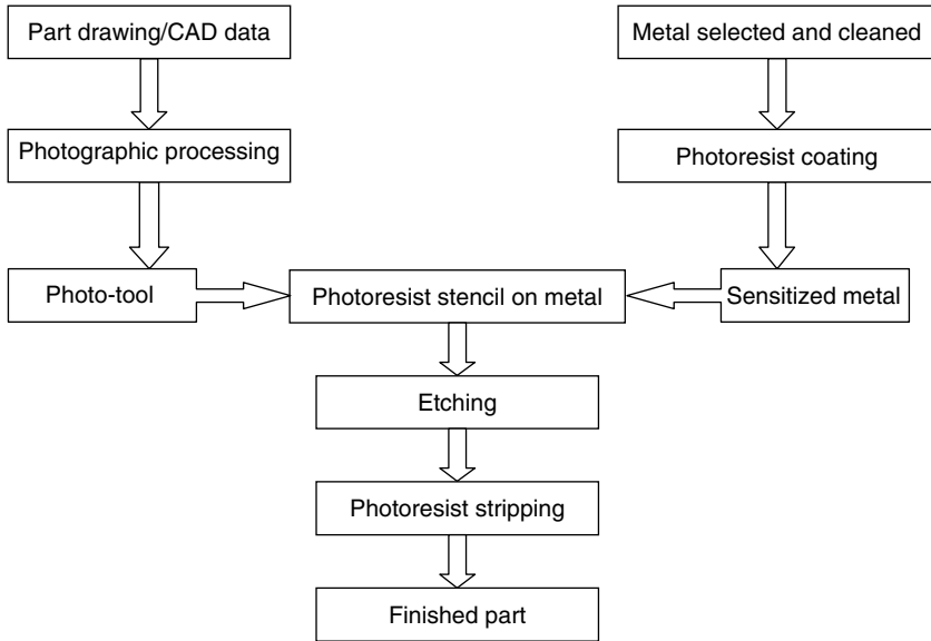
Figure 3.9 PCM flow diagram.
