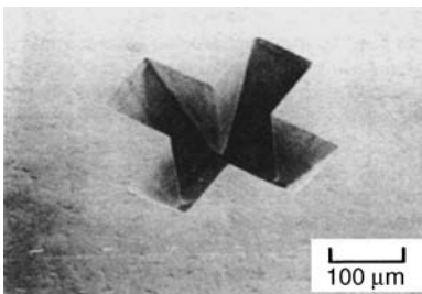
Figure 5.30 A microcavity with sharp corners by micro-EDM (Masuzawa and Tonshof, 1997).
