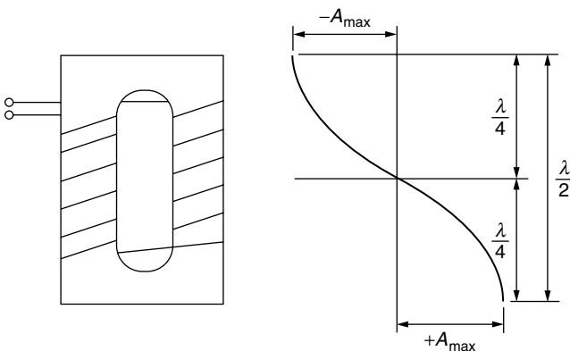
Figure 2.7 Variation in a wave of elongation along the length of the magnetostrictor (Kaczmarek, 1976).
