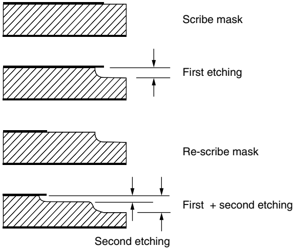
Figure 3.3 Contour cuts by CHM.
