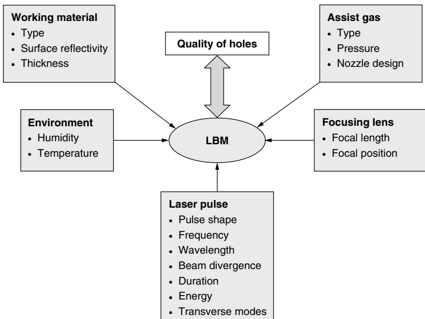
Figure 5.37 Parameters affecting the quality of laser-drilled holes.
