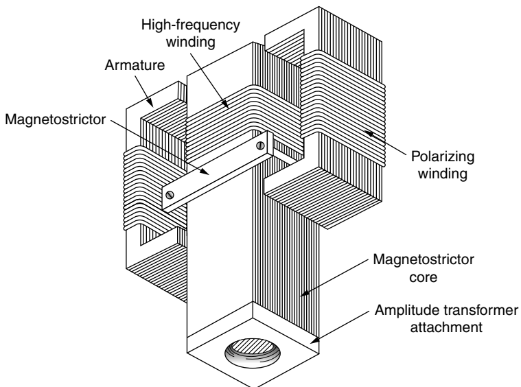
Figure 2.4 Magnetostriction transducer (Kaczmarek, 1976).
