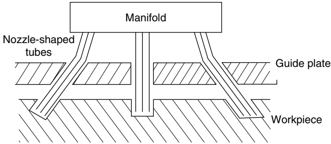
Figure 4.26 Drilling inclined holes.
