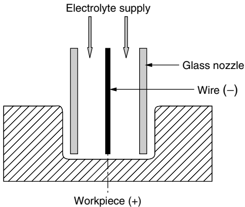
Figure 4.25 ES drilling schematic.
