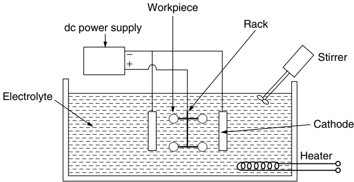
Figure 3.15 Electropolishing schematic.
