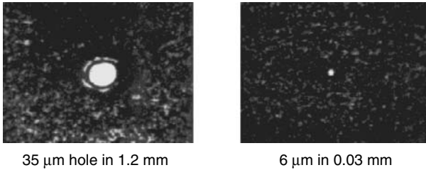
Figure 5.42 Fine drilling of holes in steel.
