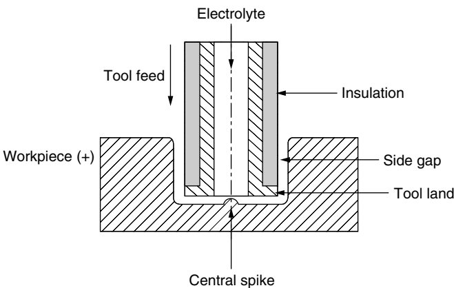
Figure 4.21 ECDR configuration.
