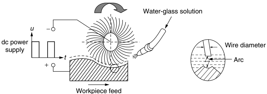
Figure 7.24 Brush mechanical EDM.
