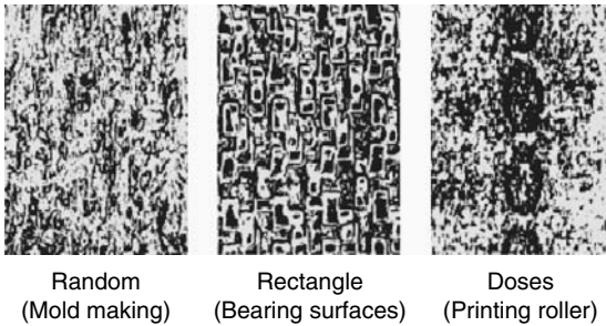
Figure 5.40 Structuring of surfaces with PM Nd-YAG laser radiation (Tonshof and Sturmer, 1995).
