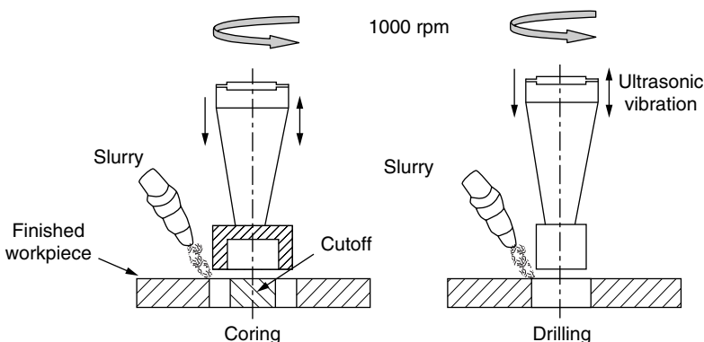
Figure 2.12 Rotary USM.
