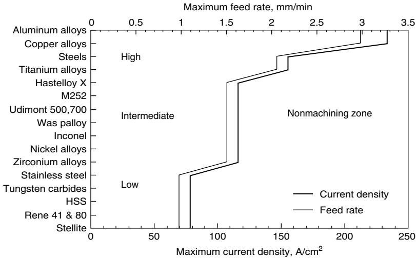
Figure 6.6 Machinability ratings in ECG (El-Hofy, 1995).
