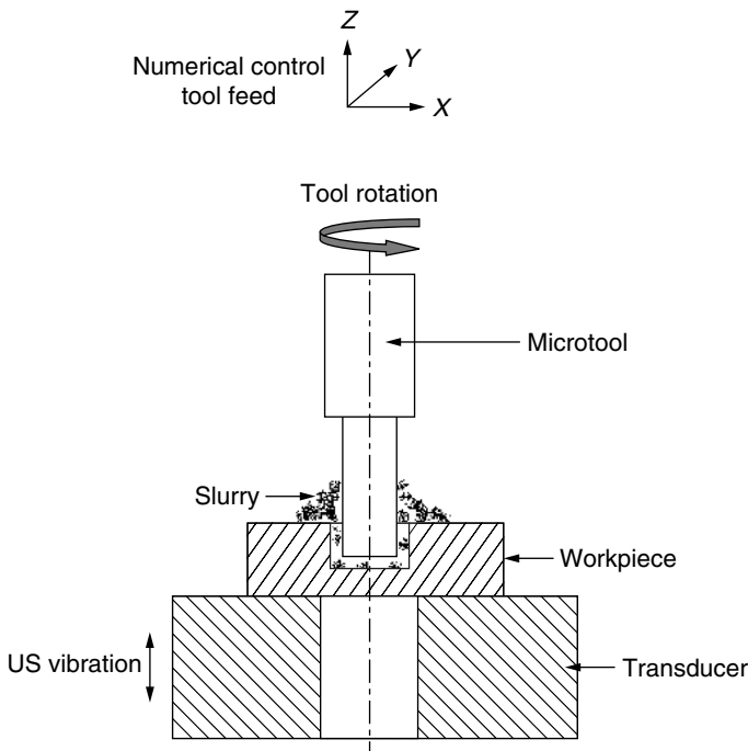
Figure 2.17 Micro-ultrasonic machining.
