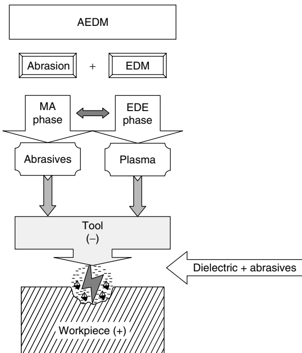
Figure 7.19 AEDM components.
