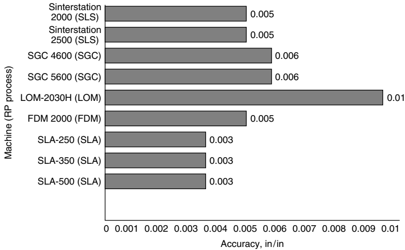
Figure 8.14 Accuracy levels for RP techniques (Wright, 2001).
