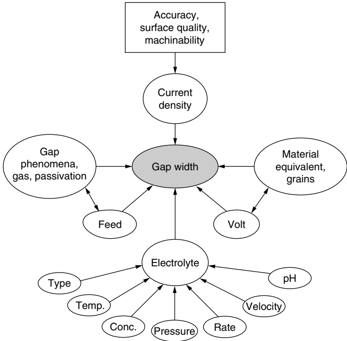
Figure 4.12 Parameters affecting ECM accuracy, surface quality, and productivity.
