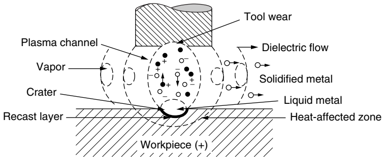
Figure 5.5 EDM spark description.
