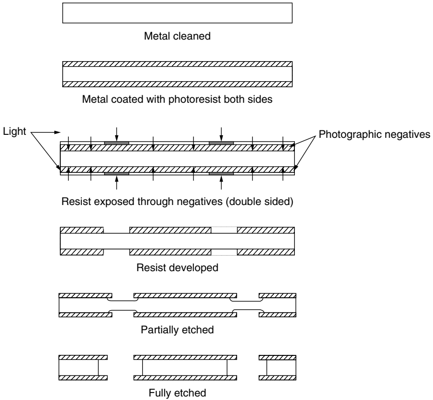
Figure 3.10 PCM steps (Thusty, 1999).
