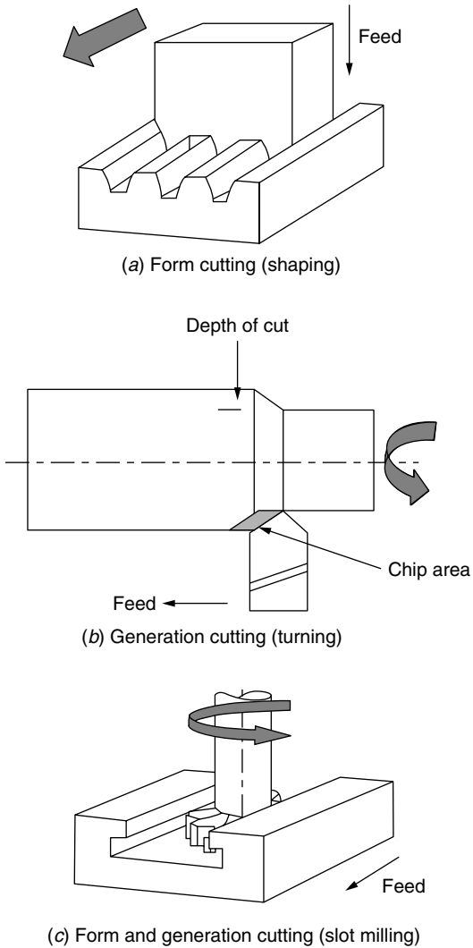
Figure 1.3 Metal cutting processes.
