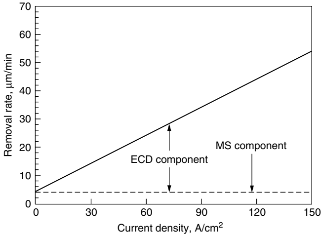
Figure 6.14 ECS removal rates at different current densities (El-Hofy, 1990).
