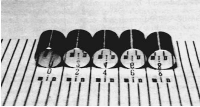
Figure 6.17 Specimens polished by ECB (Hoshino et al. 1995).
