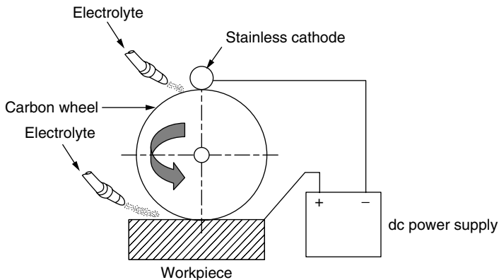
Figure 6.16 ECB schematic.
