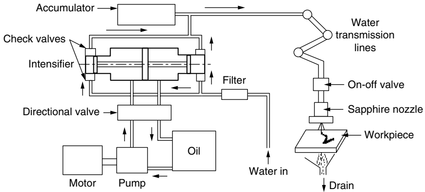
Figure 2.19 Schematic illustration of WJM system.
