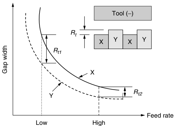
Figure 4.14 Surface roughness generation in ECM.
