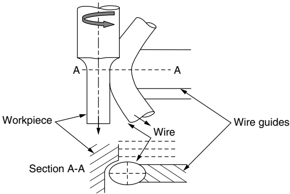
Figure 5.27 Principles of WEDG.
