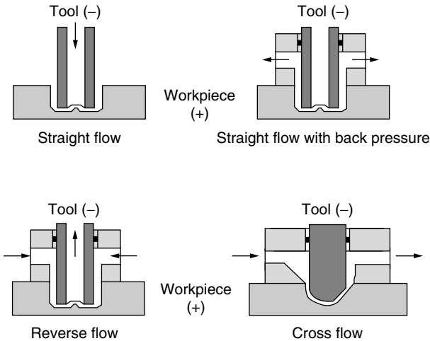
Figure 4.5 Modes of electrolyte feeding in ECM.
