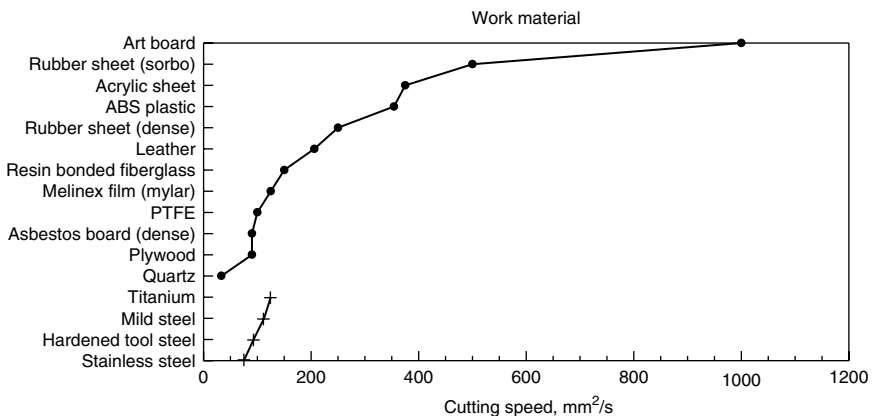
Figure 5.34 Cutting speeds in \text{CO}_2 LBM (El-Hofy, 1995).
