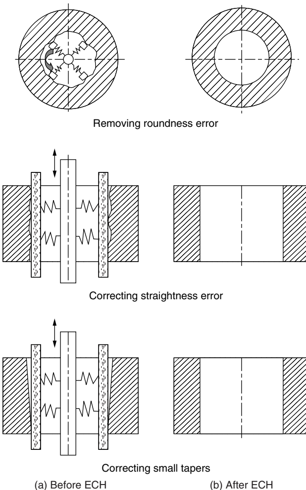
Figure 6.9 ECH effects on bore errors.
