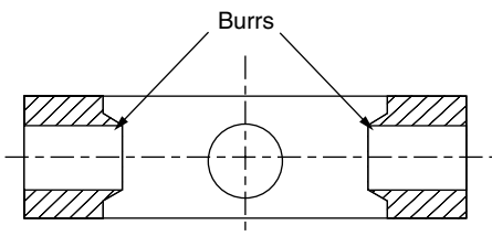
Figure 4.29 Burrs formed at intersections of holes.
