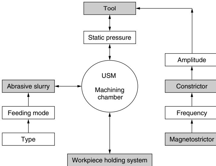
Figure 2.3 USM system components.
