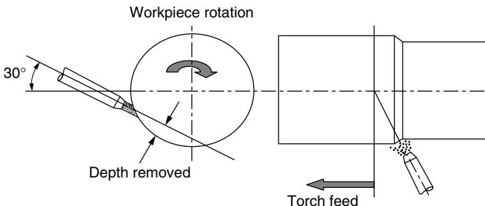
Figure 5.55 Plasma arc turning.
