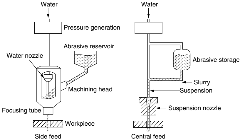
Figure 2.27 Injection and suspension jets.
