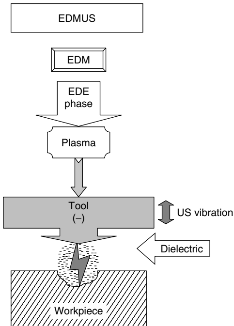
Figure 7.21 EDMUS components.
