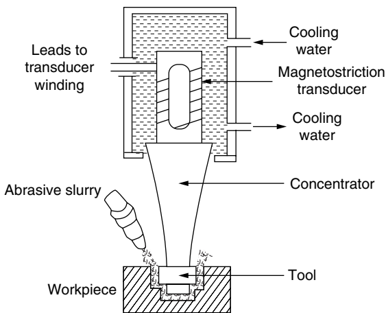
Figure 2.2 Main elements of an ultrasonic machining system.
