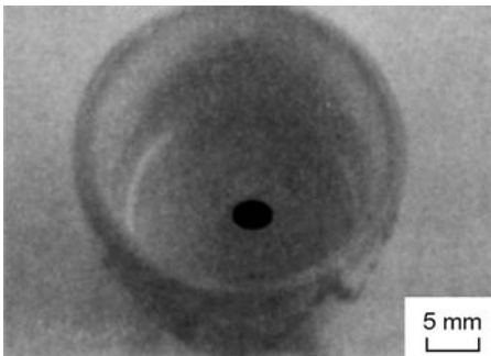
Figure 5.25 China pot machined by EDM. (Fukuzawa et al., 1995).
