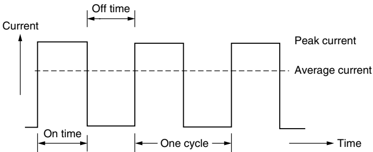
Figure 5.2 Typical EDM pulse current train for controlled pulse generator.
