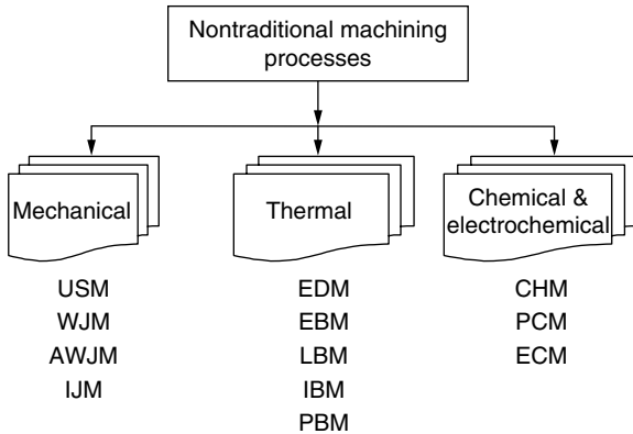
Figure 1.5 Nontraditional machining processes.
