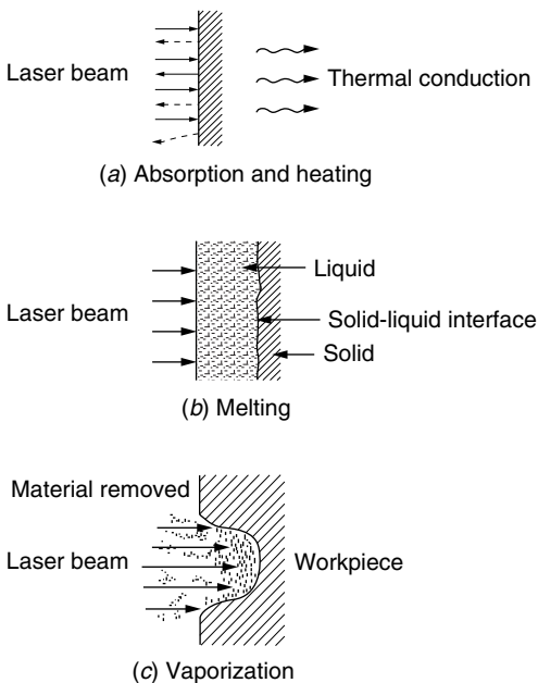
Figure 5.33 Physical processes occurring during LBM.
