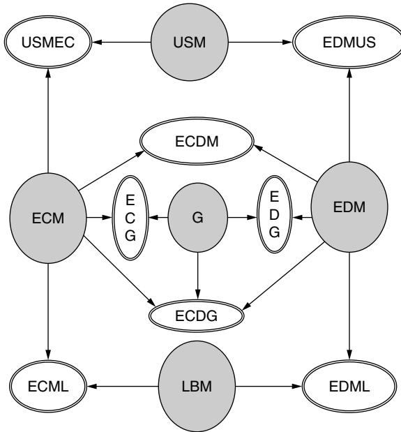
Figure 1.9 Hybrid machining processes.
