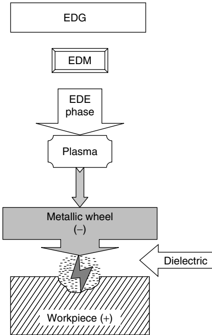
Figure 7.14 Elements of EDG.
