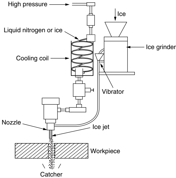
Figure 2.28 IJM schematic, modified from Geskin et al. (1995).
