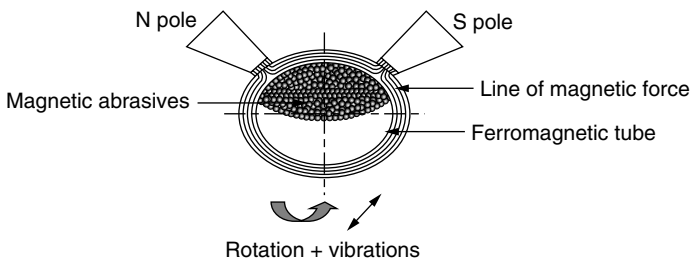
Figure 2.33 Magnetic finishing of magnetic tubes.
