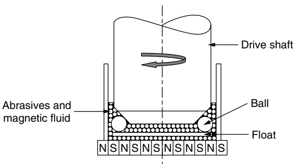
Figure 2.31 Magnetic finishing of balls (Kalpakjian, 1997).
