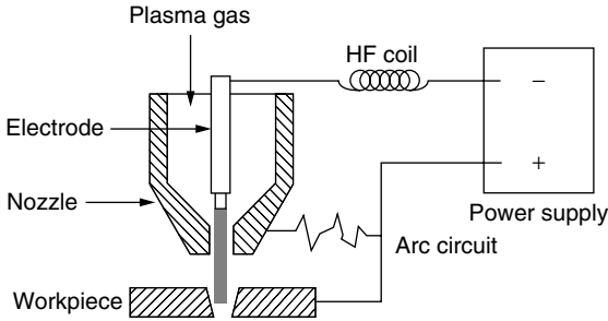
Figure 5.49 Transferred plasma arc system.
