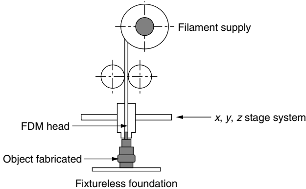
Figure 8.6 Fused deposition modeling schematic.
