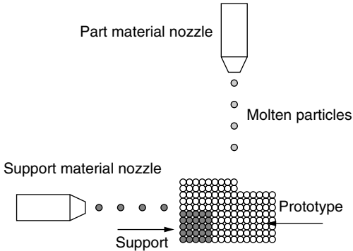
Figure 8.8 Ballistic particles manufacturing.
