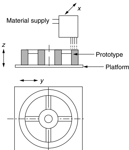
Figure 8.7 Multijet modeling principles.
