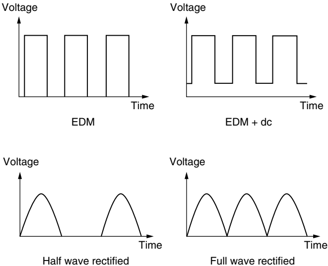
Figure 7.5 Voltage waveforms.
