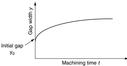
Figure 4.8 Variation of initial gap with machining time at zero feed.
