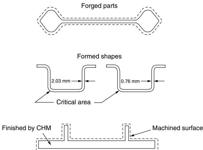
Figure 3.8 Thinning of parts by CHM (Tlustý, 1999).
