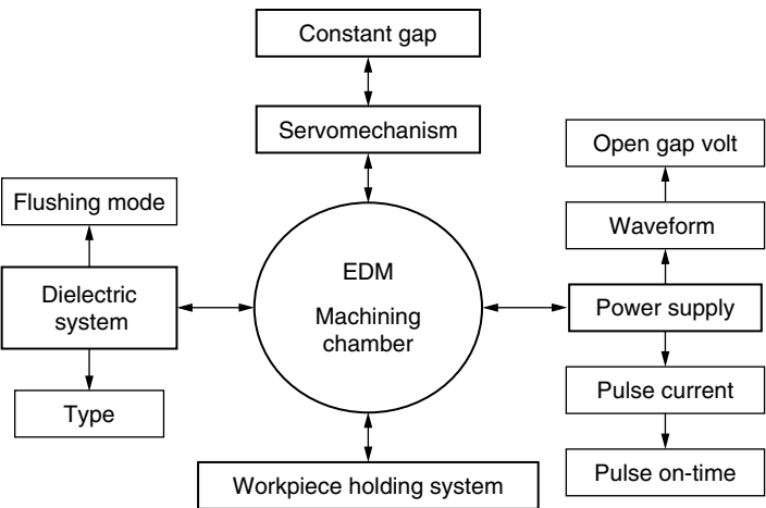
Figure 5.8 EDM system components.
