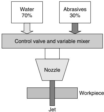
Figure 2.26 AWJM elements.
