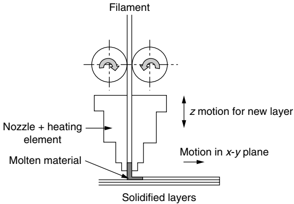
Figure 8.5 FDM principles.
