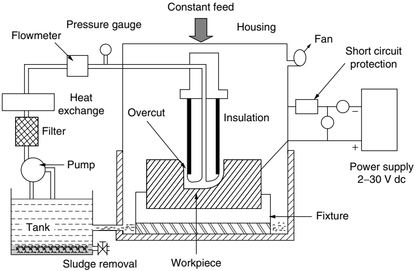
Figure 4.2 ECM elements.
