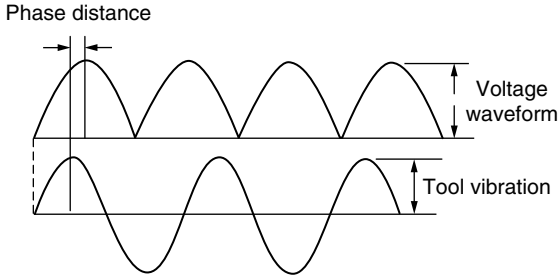
Figure 7.4 Voltage and tool-oscillation waveform (El-Hofy and McGeough, 1988).
