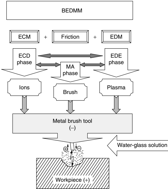
Figure 7.25 Material removal mechanisms in BEDMM.
