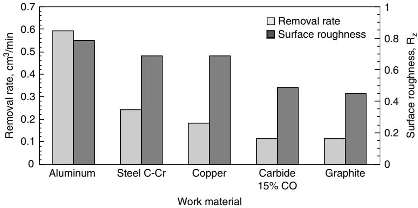
Figure 5.13 EDM removal rates and roughness for different materials (El-Hofy, 1995).
