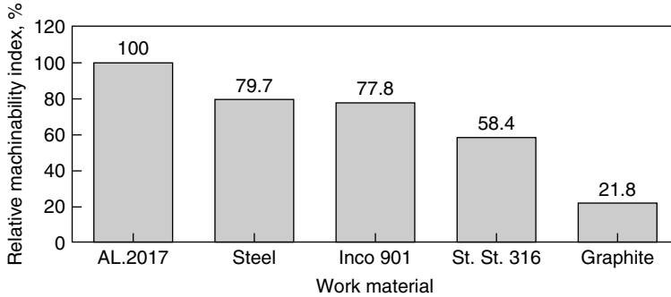
Figure 7.9 Machinability index for some materials normalized to 2017 aluminum (El-Hofy, 1995).
