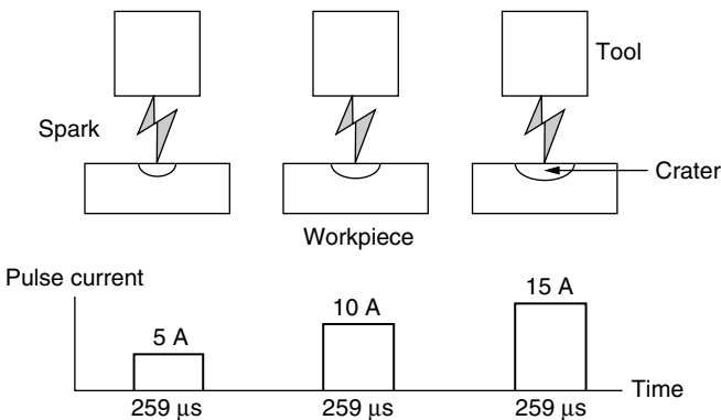
Figure 5.14 Effect of pulse current (energy) on removal rate and surface roughness.
