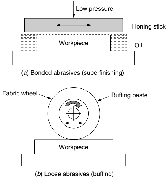
Figure 1.4 Abrasive machining.
