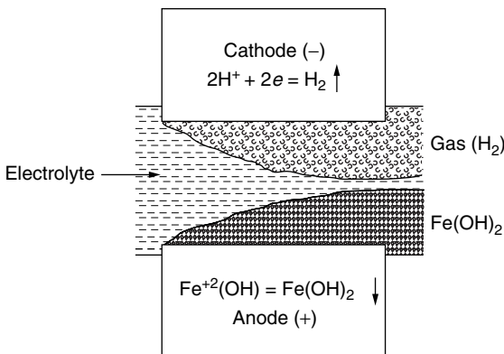
Figure 4.1 Electrochemical reactions during ECM of iron.
