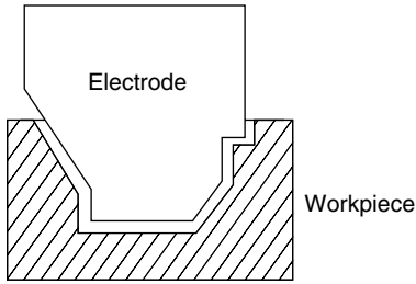
Figure 5.20 EDM die sinking.
