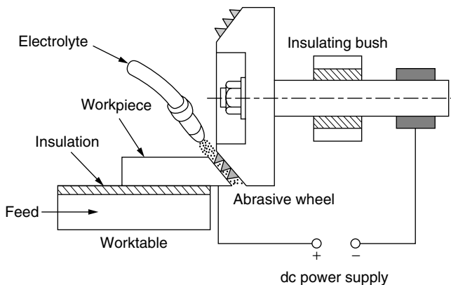
Figure 6.3 ECG machining system components.
