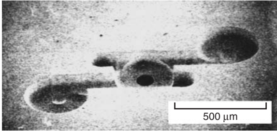
Figure 2.18 Micro-ultrasonic machined cavity (Masuzawa and Tonshof, 1997).
