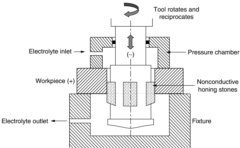
Figure 6.8 ECH machining system components.
