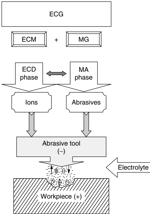
Figure 6.4 ECG process components.
