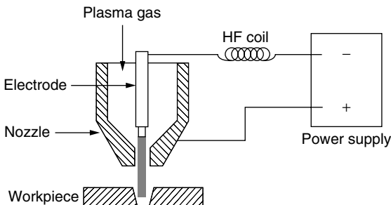
Figure 5.50 Nontransferred plasma jet system.
