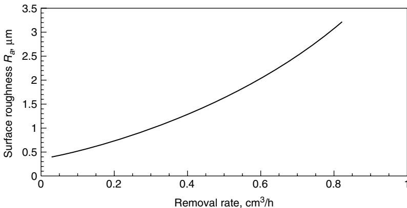
Figure 7.13 Removal rate and surface roughness in EDG (El-Hofy, 1995).
