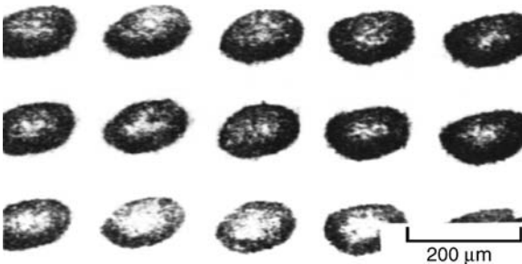
Figure 4.19 Micromachined indents by electrolyte jet ECM (Masuzawa and Tonshof, 1997).
