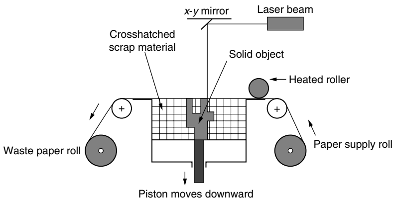
Figure 8.13 Laminated object modeling (LOM).
