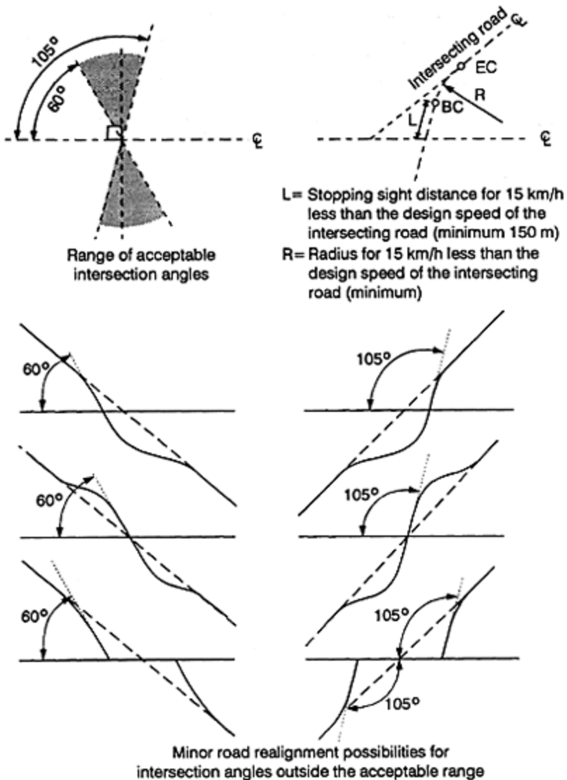
Figure 8.6 Alignment of intersecting roads (ref. 4).
