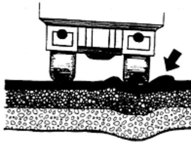
Figure 20.3 Shoving (ref. 2).
