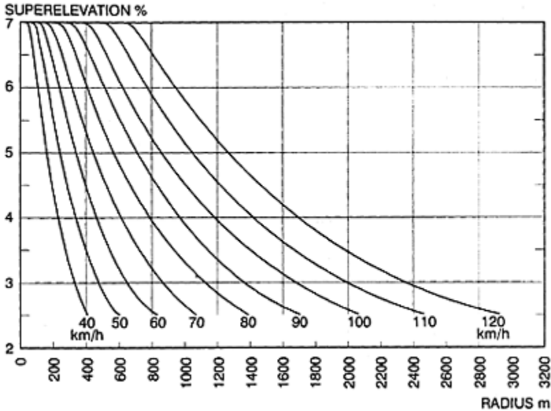
Figure 9.3 Superelevation design curves (ref. 4).
