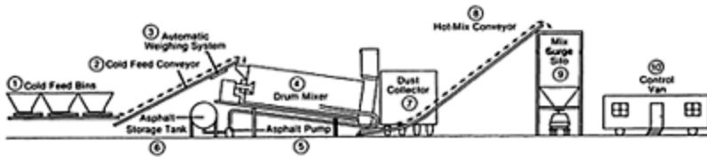
Figure 15.5 Drum mixer (ref. 5)
