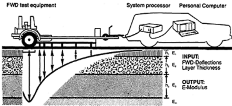
Figure 16.5 Falling weight deflectometer.
