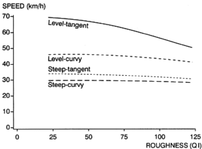
Figure 4.6 Speed as a function of road characteristics for a half-laden heavy truck (ref. 4).
