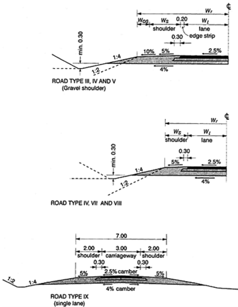
Figure 9.2 Typical cross-section (ref. 3).
