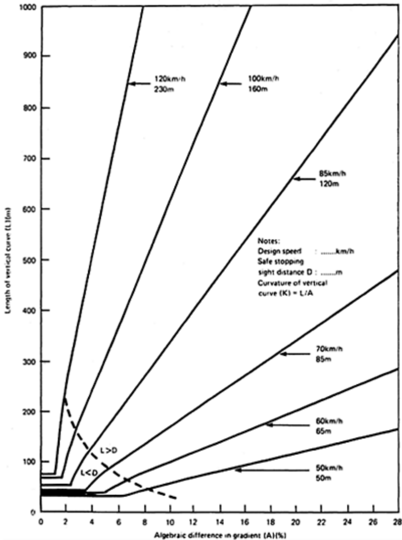
Figure 8.3 Length of crest vertical curves for safe stopping sight distance (TRRL Overseas Road Note 6, ref. 1).
