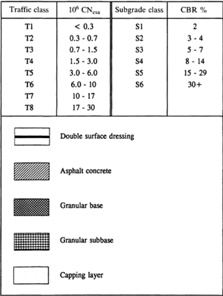
Figure 16.2 Key to the design charts in TRL Overseas Road Note 31 (ref. 2).
