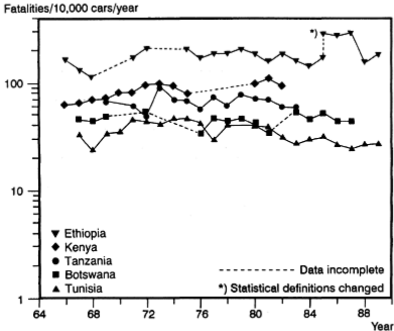
Figure 6.4 Fatality rates for selected African countries, all apparently in phase I.
