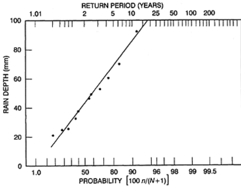
Figure 10.2 Extreme probability plot (ref. 1).
