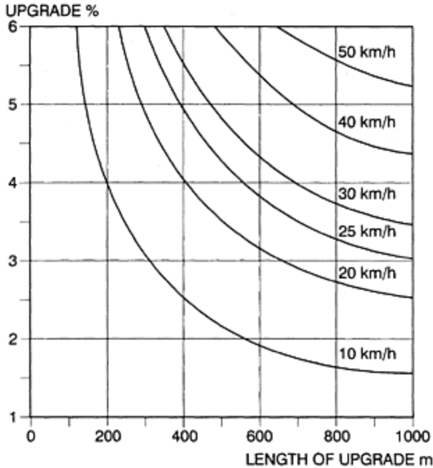
Figure 8.2 Speed reduction effect of upgrade (ref. 4).
