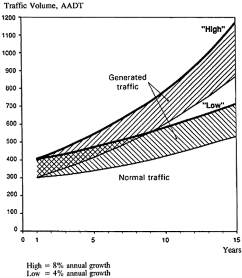
Figure 3.1 Example of traffic forecast.
