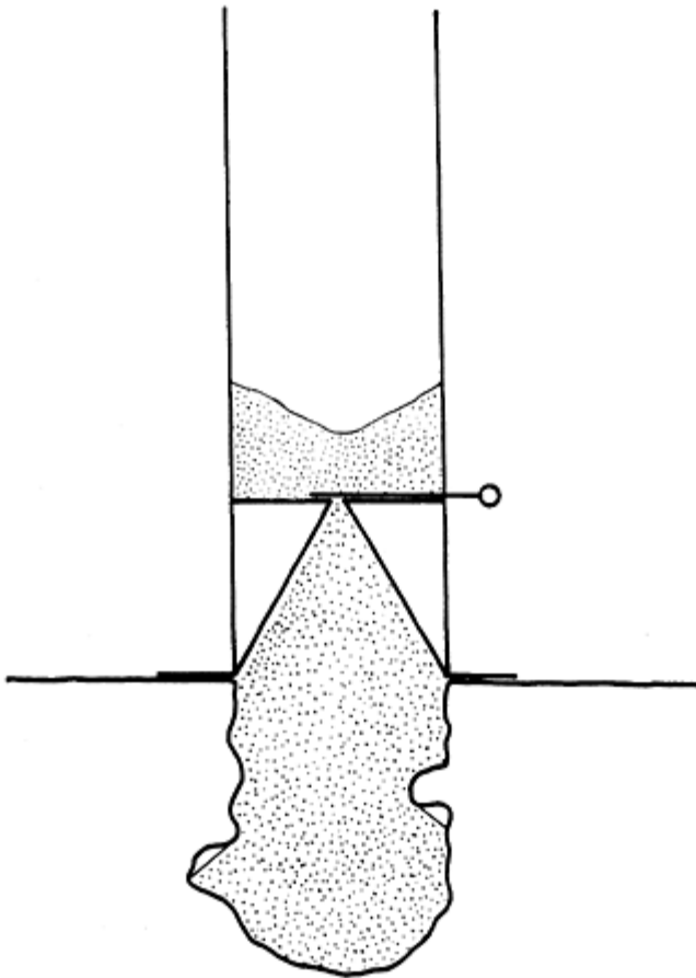
Figure 12.9 Sand cone.
