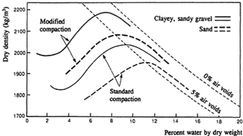
Figure 12.10 Example of compaction curves (ref. 7). (Crown copyright; reproduced with the permission of the Controller of HMSO.)
