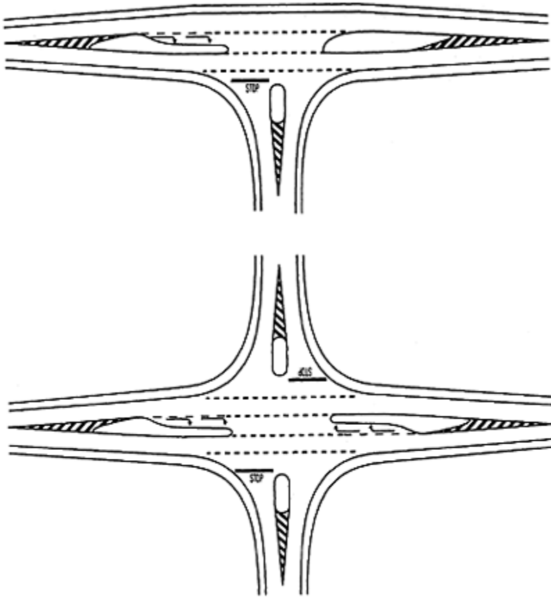
Figure 8.9 Channelized intersection layouts (ref. 2).
