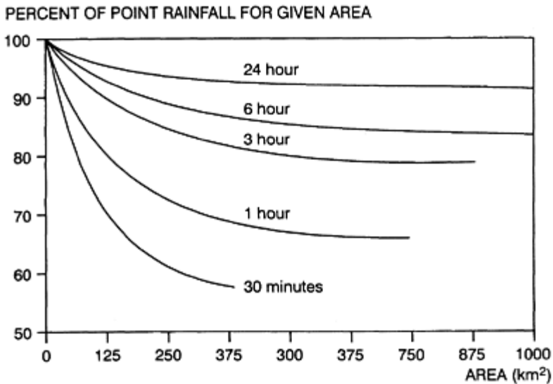
Figure 10.1 Area reduction for a five-year recurrence interval (ref. 1).
