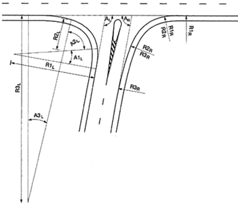
Figure 8.10 Design of the edge of the carriageway with a three-point curve (ref. 2).
