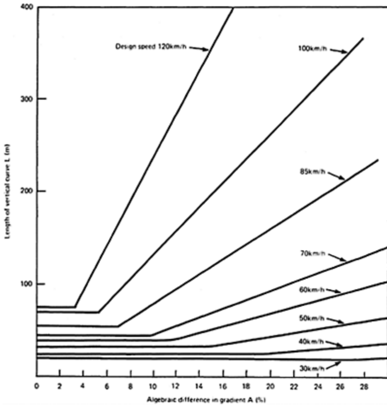
Figure 8.4 Length of sag vertical curve for adequate riding comfort (TRRL Overseas Road Note 6, ref. 1).
