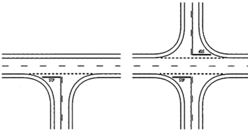
Figure 8.7 Intersection layouts for low-volume roads and for property access (ref. 2).
