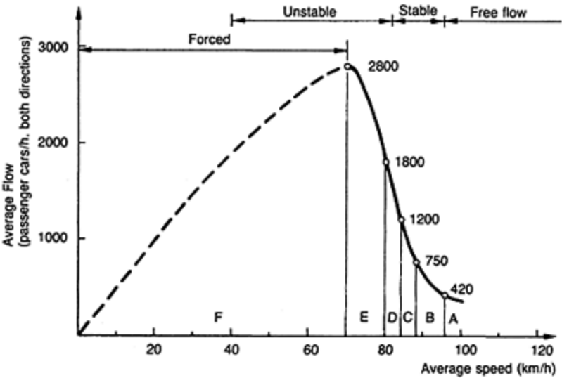
Figure 7.1 Speed-flow diagram.
