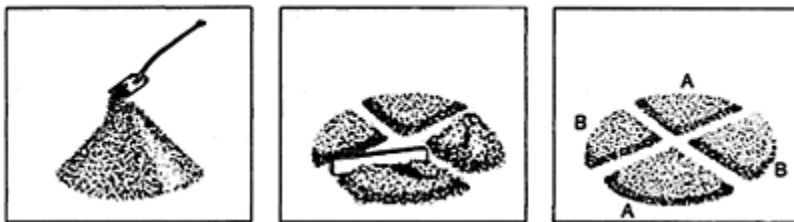
Figure 12.6 Quartering.
