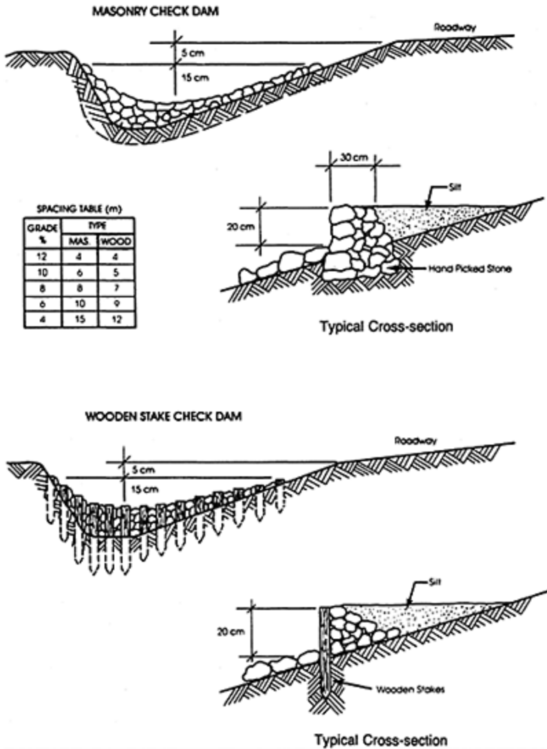
Figure 11.12 Ditch checks (ref. 4).
