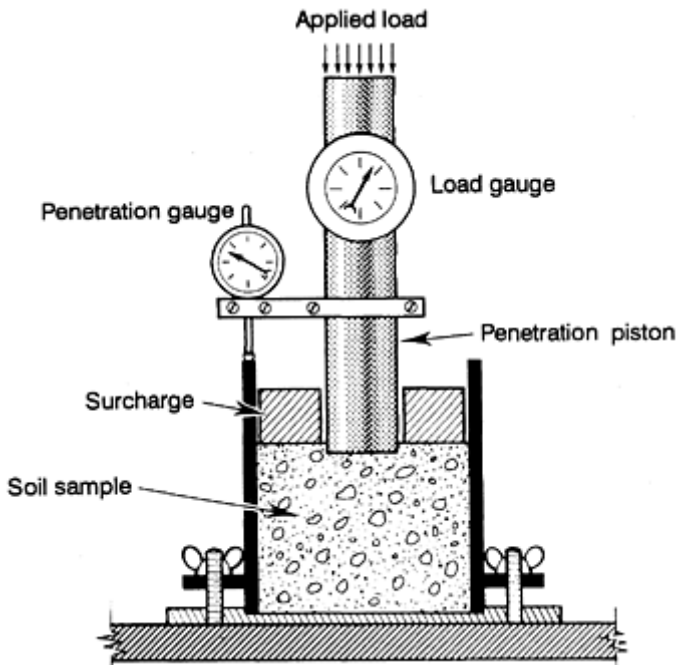
Figure 12.11 Equipment for CBR testing.
