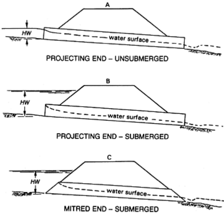
Figure 11.6 Inlet control (Transportation Research Board, ref. 3).
