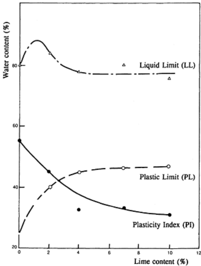
Figure 14.8 Effect of the addition of lime on a London clay (ref. 5). (Crown copyright; reproduced with the permission of the Controller of HMSO.)
