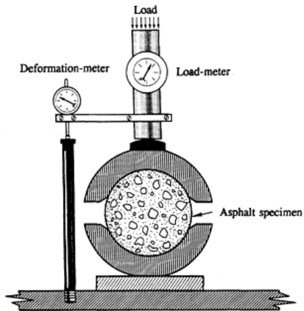
Figure 15.7 Marshall testing machine.
