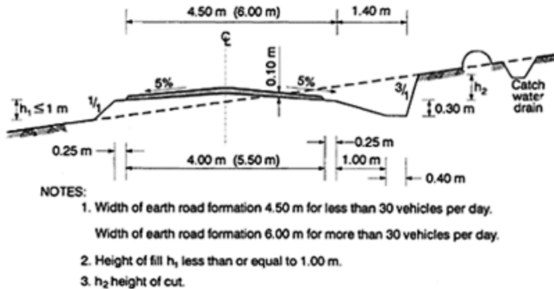
Figure 19.9 Standard cross-sections (copyright International Labour Organisation, ref. 11).
