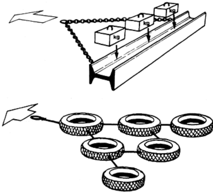
Figure 20.6 Beam drag and tyre drag (ref. 2).
