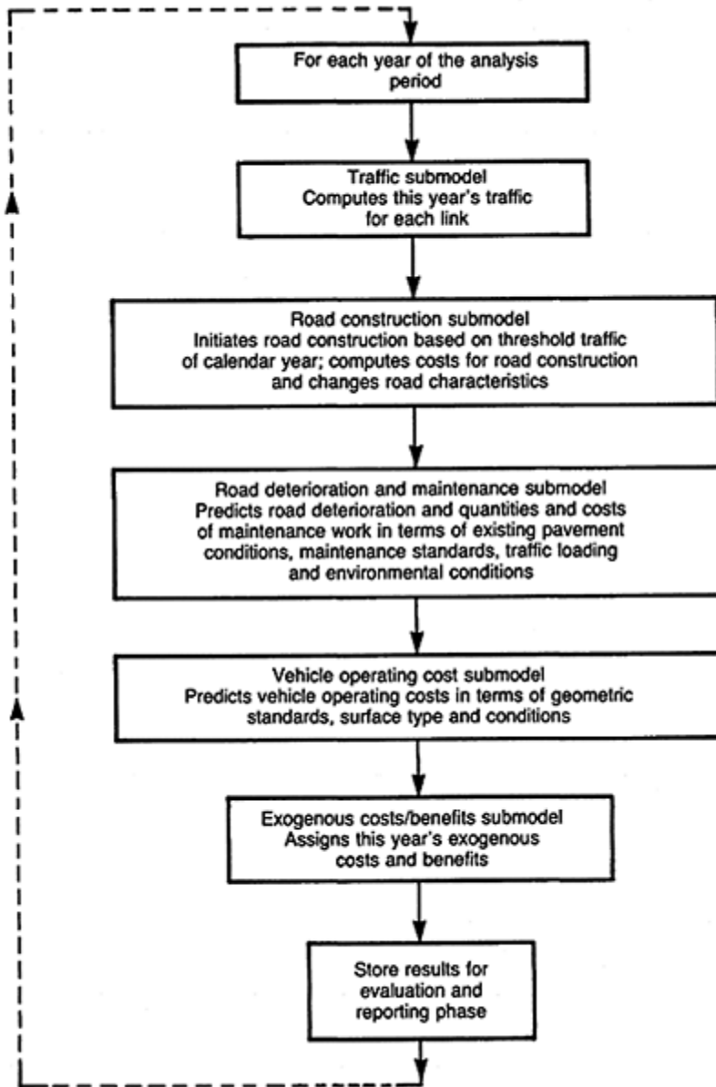
Figure 4.1 Simulation of a link alternative (ref. 4).
