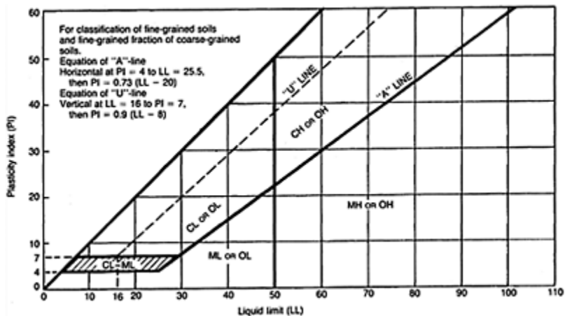
Figure 12.13 Unified Soil Classification System (ref.4)
