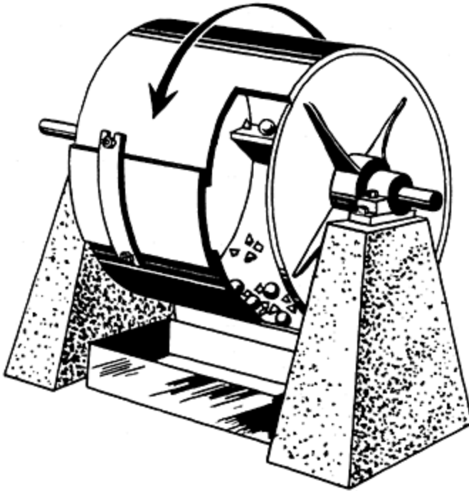
Figure 12.12 Los Angeles abrasion machine (ref. 8).
