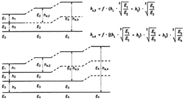
Figure 16.7 Three- and four-layer systems.
