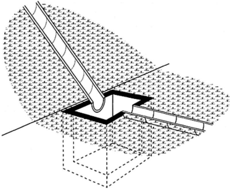
Figure 11.2 Chute outlet.
