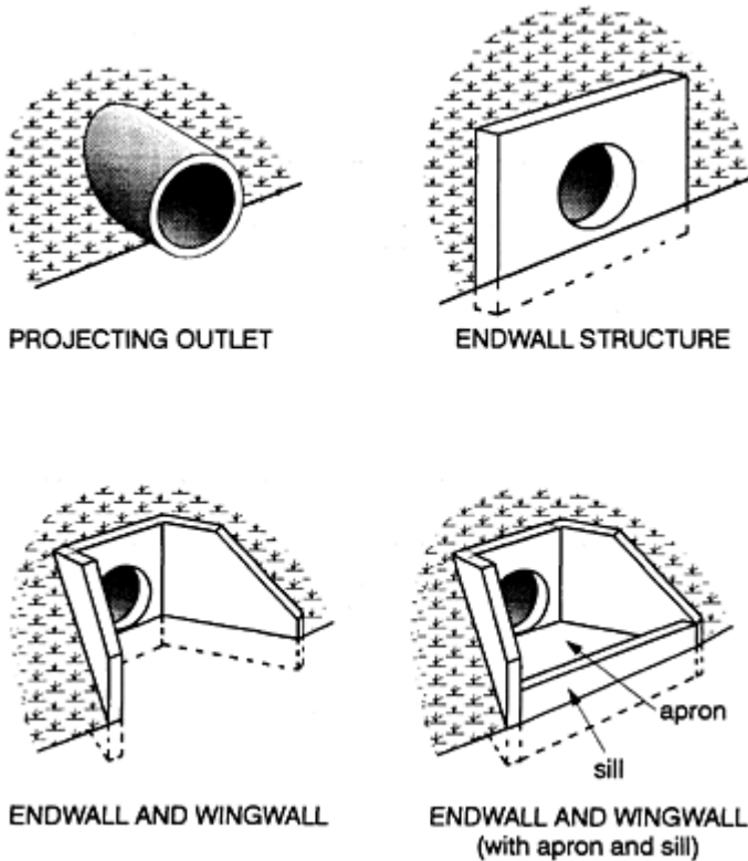
Figure 11.5 Types of culvert outlets.
