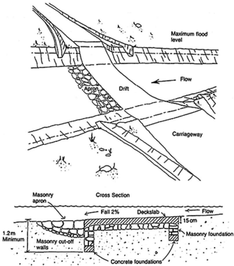
Figure 11.3 Drift (copyright International Labour Organisation) (ref. 1).
