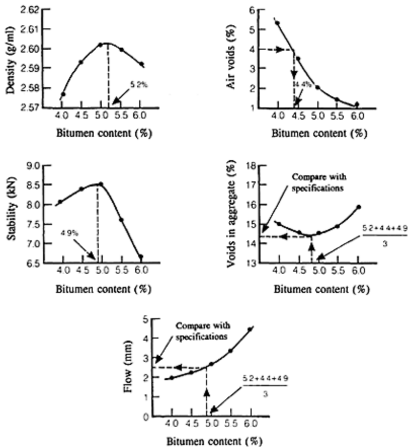
Figure 15.8 Results from a Marshall test (ref. 4).
