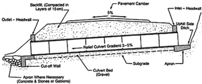
Figure 11.4 Pipe culvert (ref. 4).
