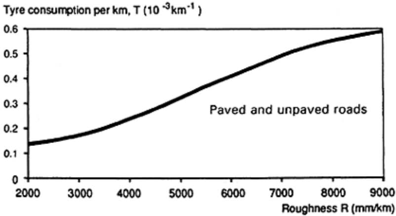
Figure 3.2 Tyre consumption equation for cars and light vehicles (TRRL Laboratory Report 1057, ref. 3).
