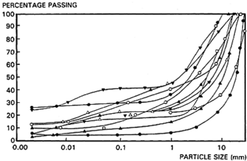
Figure 13.2 Typical gradings of lateritic gravels (ref. 2). (Crown copyright; reproduced with the permission of the Controller of HMSO.)
