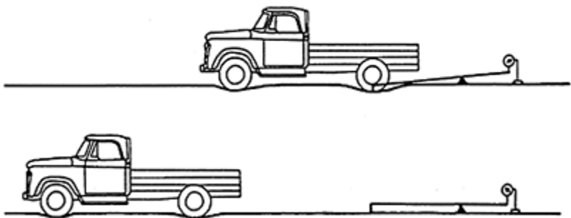
Figure 16.8 Benkelman beam measurement.
