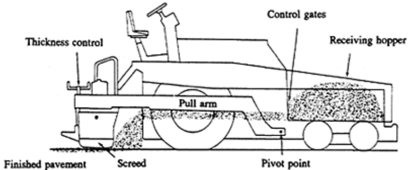
Figure 15.6 Asphalt paver (ref. 5).
