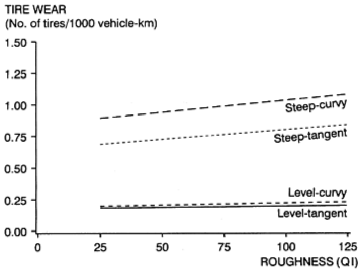
Figure 4.7 Tyre wear as a function of road characteristics for a half-laden heavy truck on a paved road (ref. 4).
