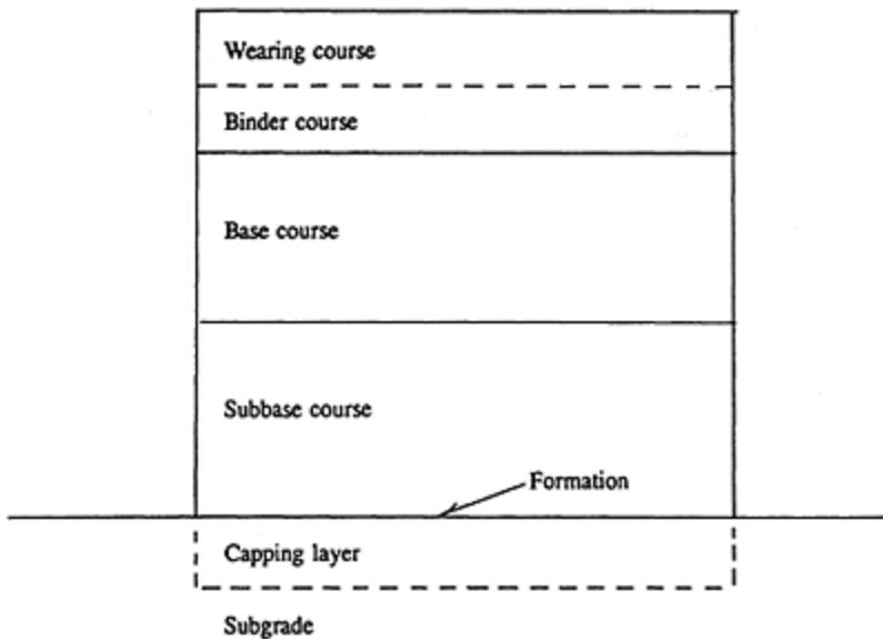
Figure 14.7 Terms used for the different pavement layers.
