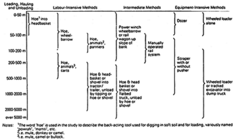
Figure 19.8 Available earthmoving methods (ref. 9).
