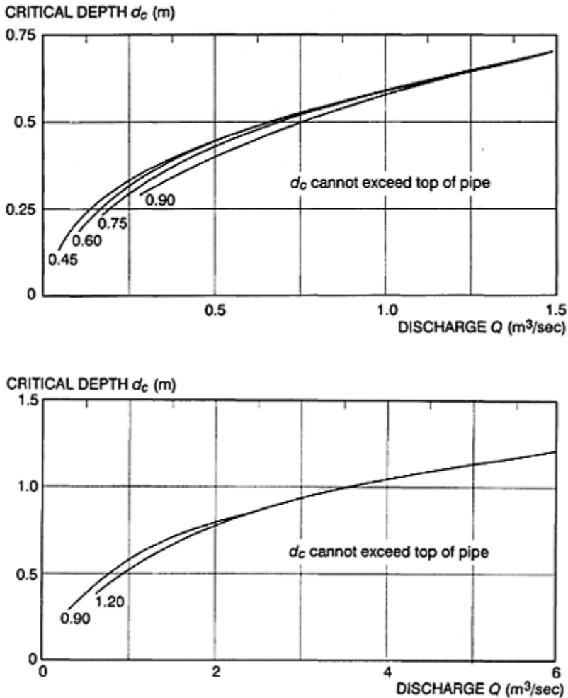
Figure 11.10 Critical depth for pipe culverts with different diameters in m (after Transportation Research Board, ref. 3).
