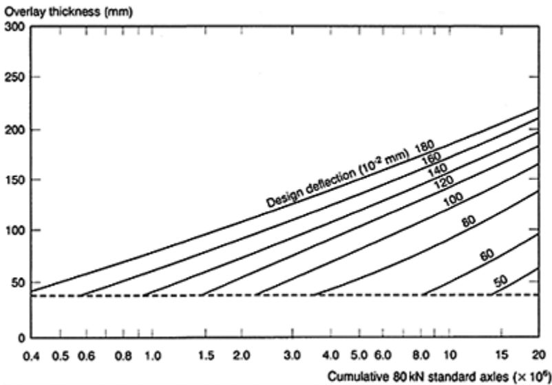
Figure 16.9 Overlay design chart for pavements with granular base (ref. 9).
