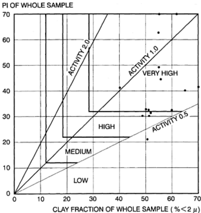
Figure 13.5 Potential swelling tendency of clays (ref. 5).
