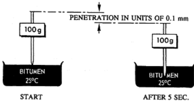
Figure 15.1 Penetration test.
