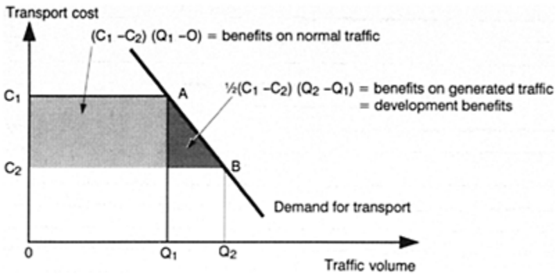
Figure 3.3 Vehicle operating cost savings.
