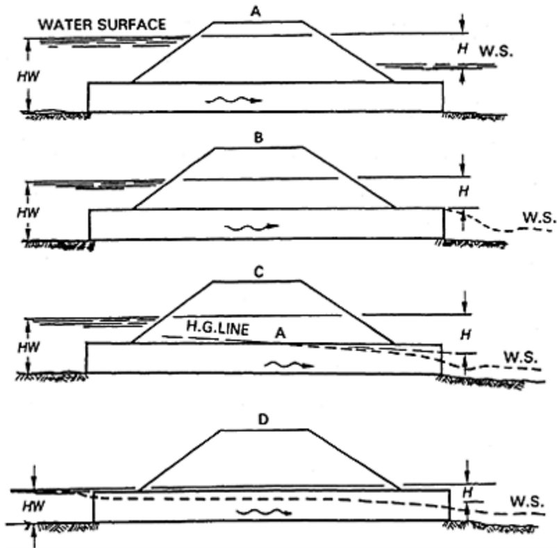
Figure 11.7 Outlet control (Transportation Research Board, ref. 3).
