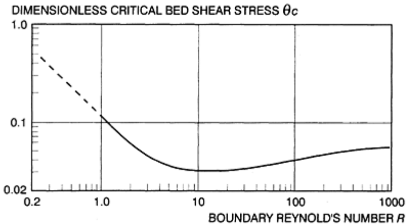
Figure 11.13 Shield's diagram (reproduced by permission of American Society of Civil Engineers, ref. 7).
