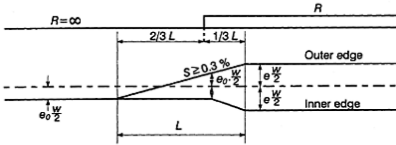
Figure 9.4 Development of superelevation for a circular curve without a transition curve (ref. 3).
