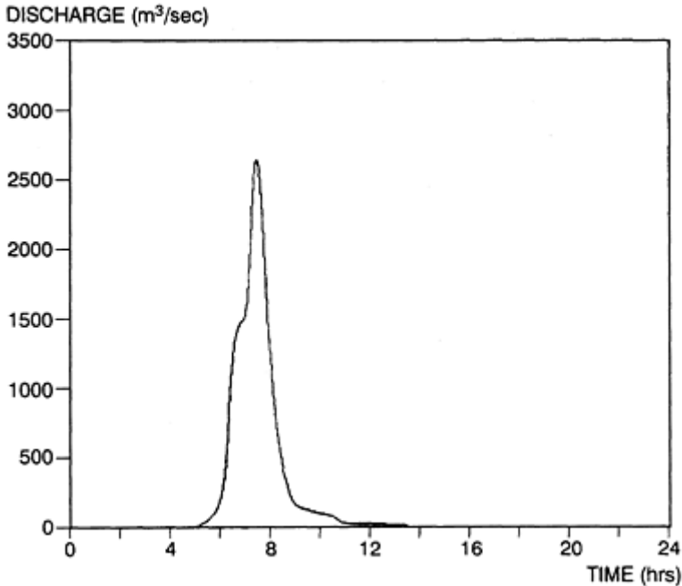
Figure 10.4 A flood hydrograph combining flows from several mountain catchments.
