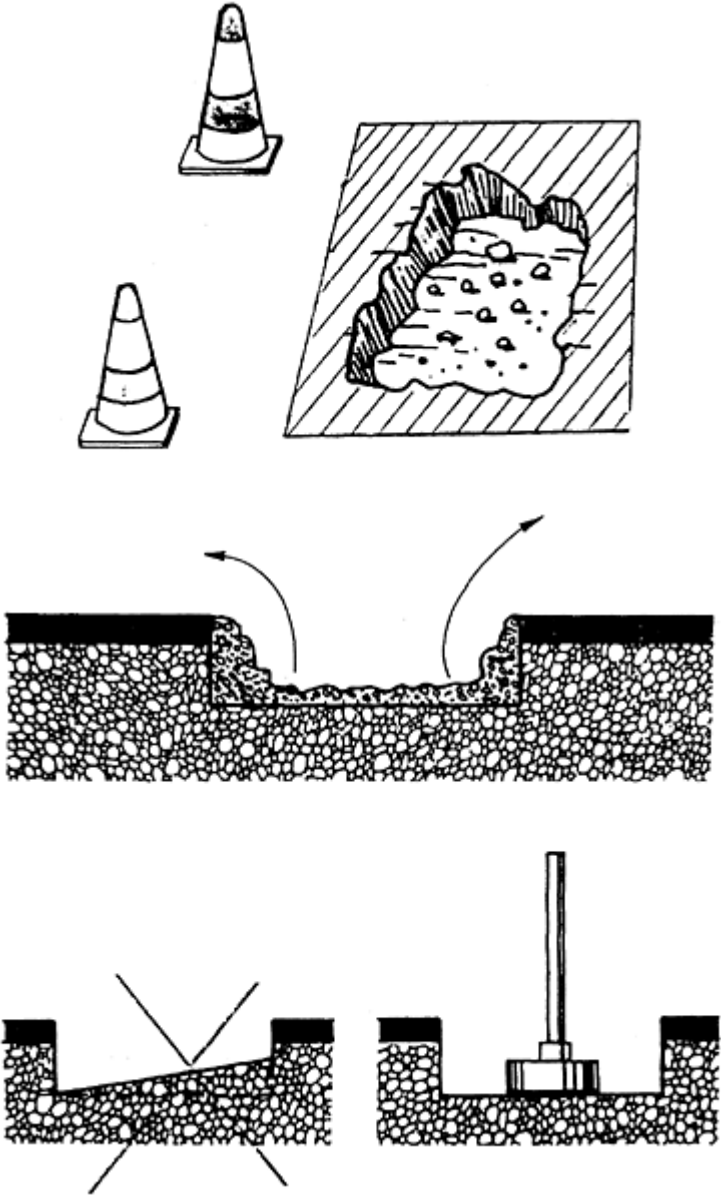
Figure 20.5 Patching of potholes (ref. 2).
