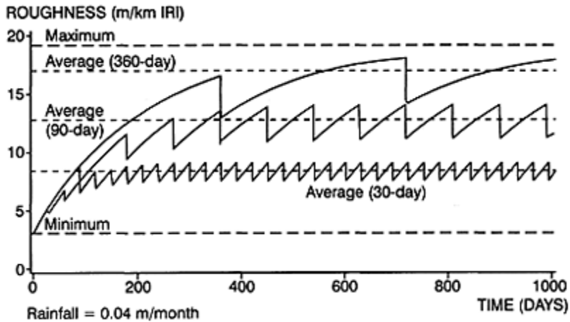
Figure 4.5 Roughness progression and effect of grading (ref. 6).
