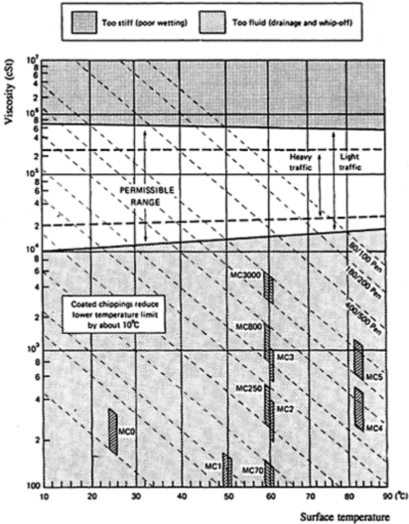
Figure 15.2 Choice of binder for surface dressing (TRRL Overseas Road Note 3, ref. 2).
