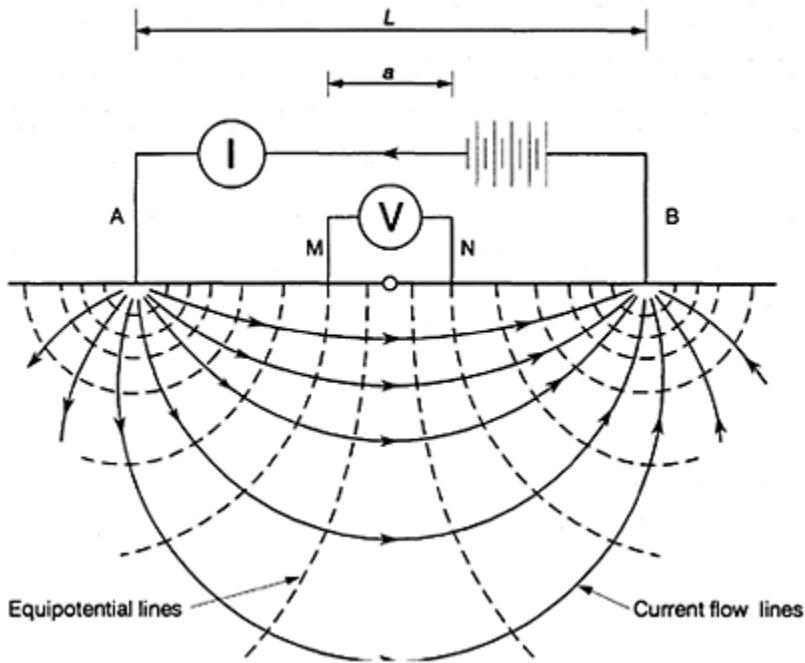
Figure 12.5 Equipotentials and current lines in a homogeneous earth.
