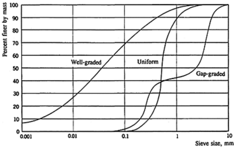
Figure 12.7 Particle size distribution curves.
