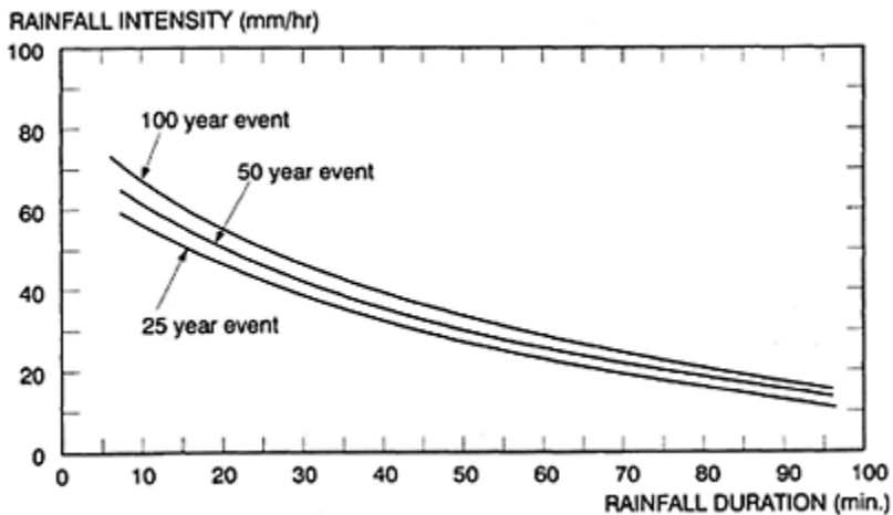
Figure 10.3 Intensity-duration curves.
