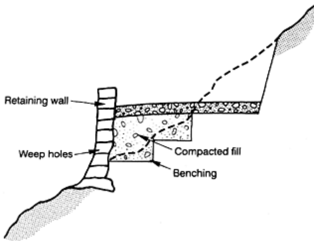
Figure 14.4 Cross-section of a road in steep side-sloping terrain.
