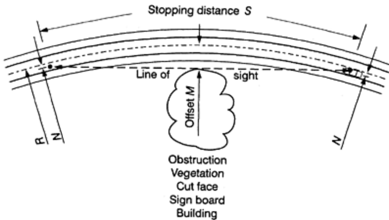
Figure 8.1 Minimum offset to obstruction adjacent to curve.
