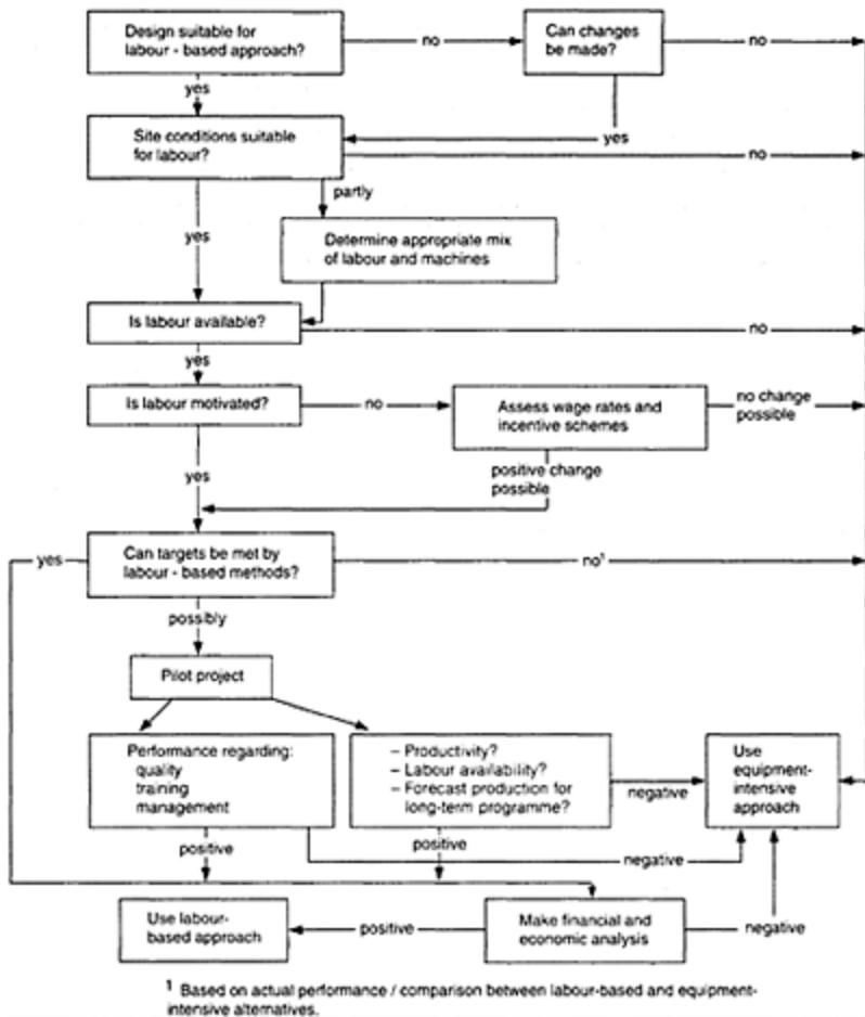
Figure 19.3 Decision-making relating to the choice of technology (copyright International Labour Office, ref. 2).
