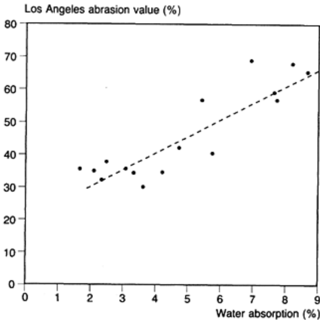
Figure 13.3 Relation between water absorption and Los Angeles abrasion value for typical West African lateritic gravels (ref. 4).
