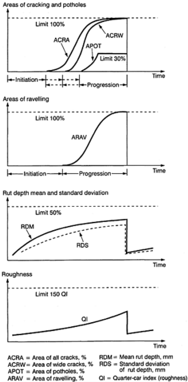
Figure 4.2 Pavement distress prediction (ref. 4).
