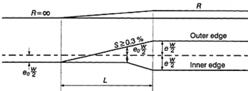
Figure 9.5 Development of superelevation for a circular curve with a transition curve (ref. 3).
