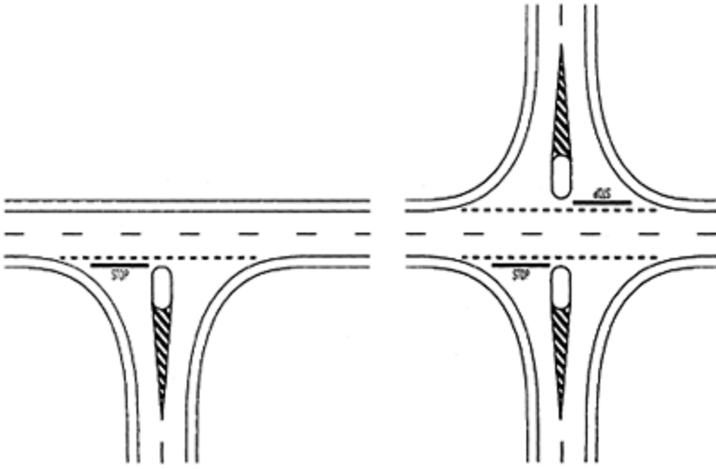
Figure 8.8 Intersection layouts for low-volume roads with light turning traffic from the major to the minor road (ref. 2).
