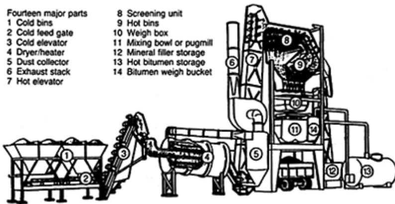
Figure 15.4 Batch mixer (ref. 4).
