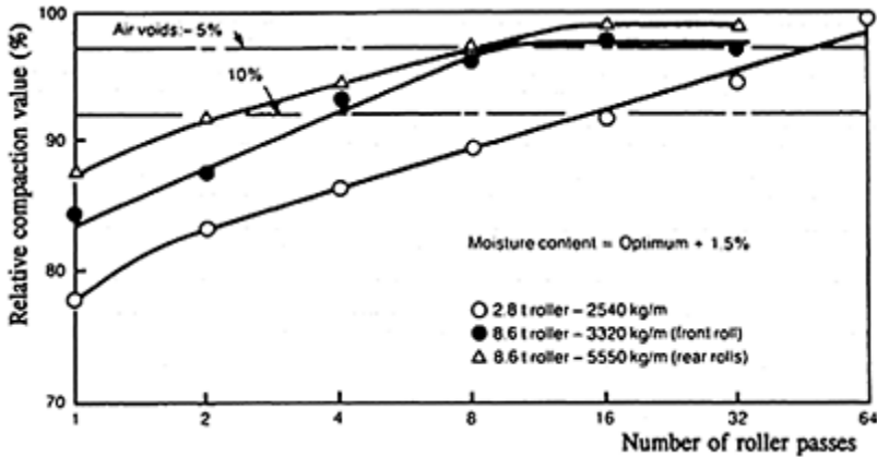
Figure 14.6 Relations between relative compaction of a sandy clay and the number of passes of smooth steel-wheeled rollers (ref. 4). (Crown copyright; reproduced with the permission of the Controller of HMSO.)
