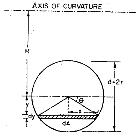
Fig. 17-6. Circular section.
