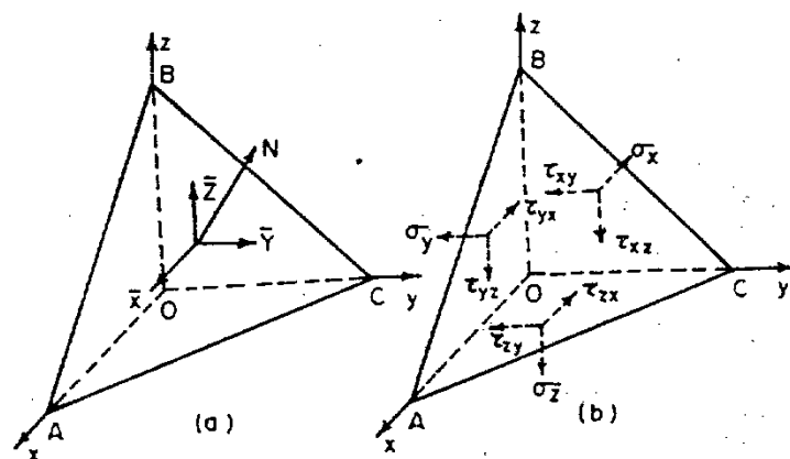
Fig. 22'4. Boundary conditions.
