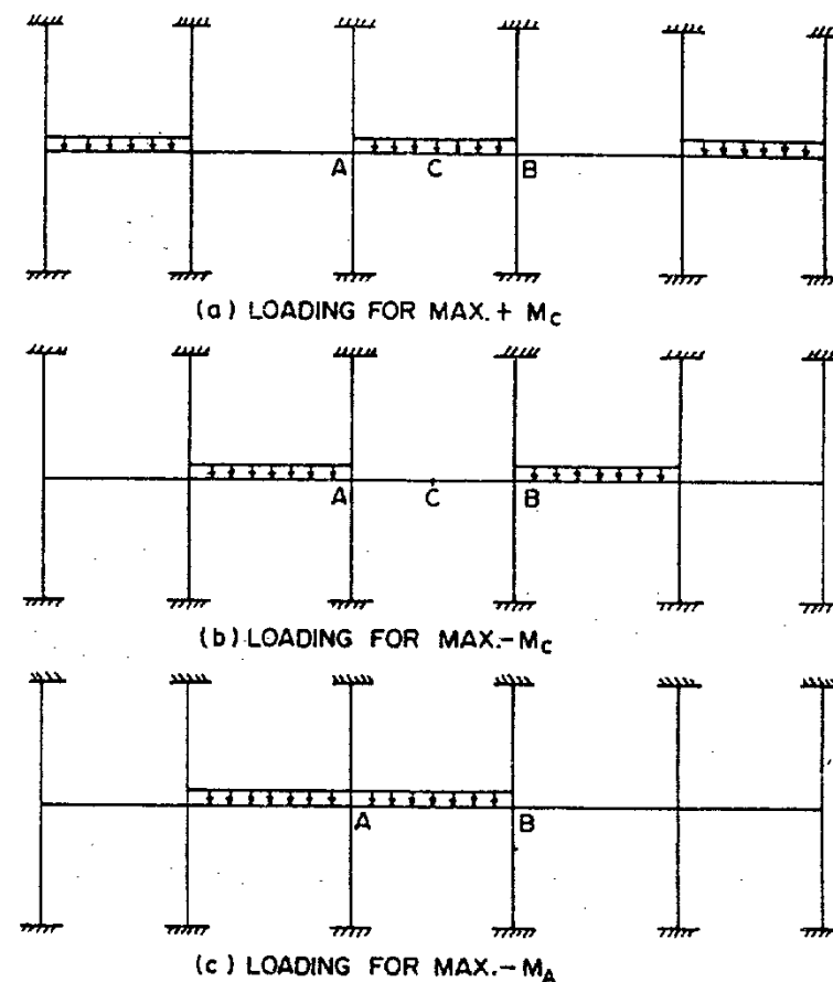
Fig. 27.3. Loading for bending moments in beams.
