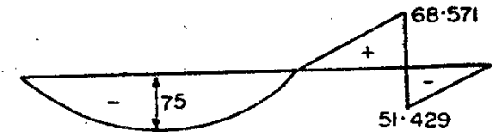
(b) FREE B.M.D.
