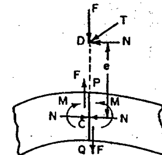
Fig. 16.2. Theoretical arch.
