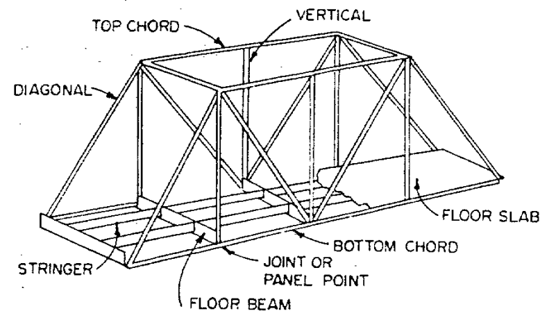
(a) TRUSS WITH FLOOR BEAMS
