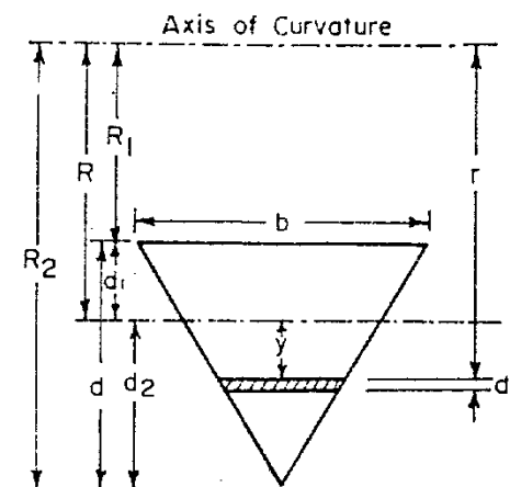
Fig. 17-5. Triangular section.
