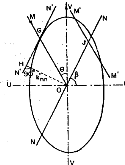
Fig. 21'12. Determination of k_{NN} .
