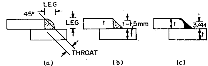
Fig. 23.2. Fillet welds.
