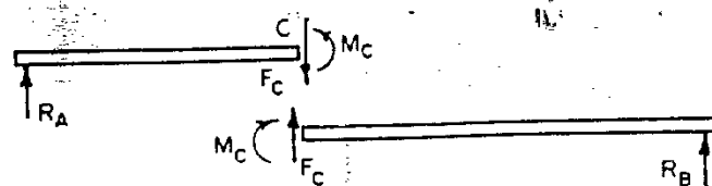
(b) FREE BODY DIAGRAMS OF THE TWO PARTS
