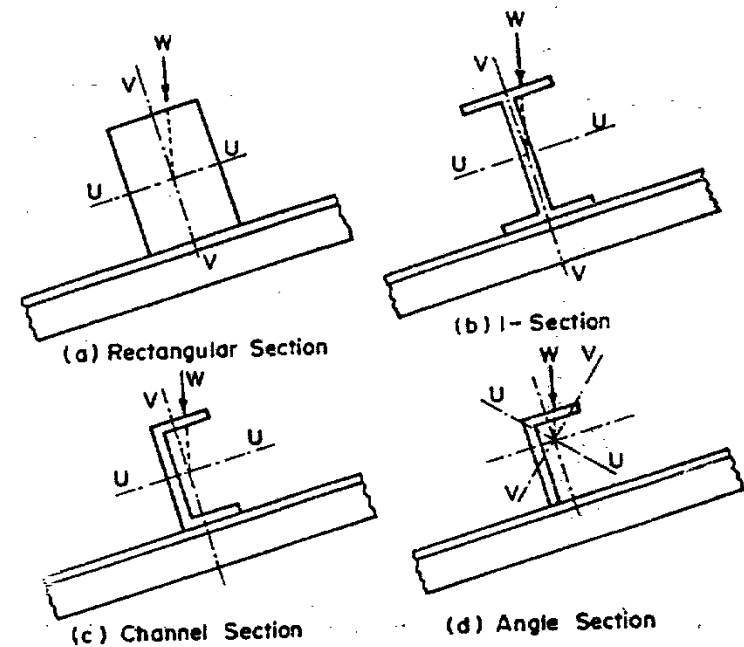
Fig. 21.1. Unsymmetrical bending.
