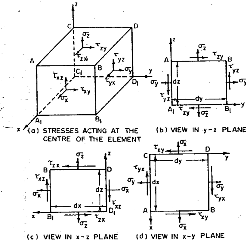
Fig. 22'1. Three dimensional stress field.
