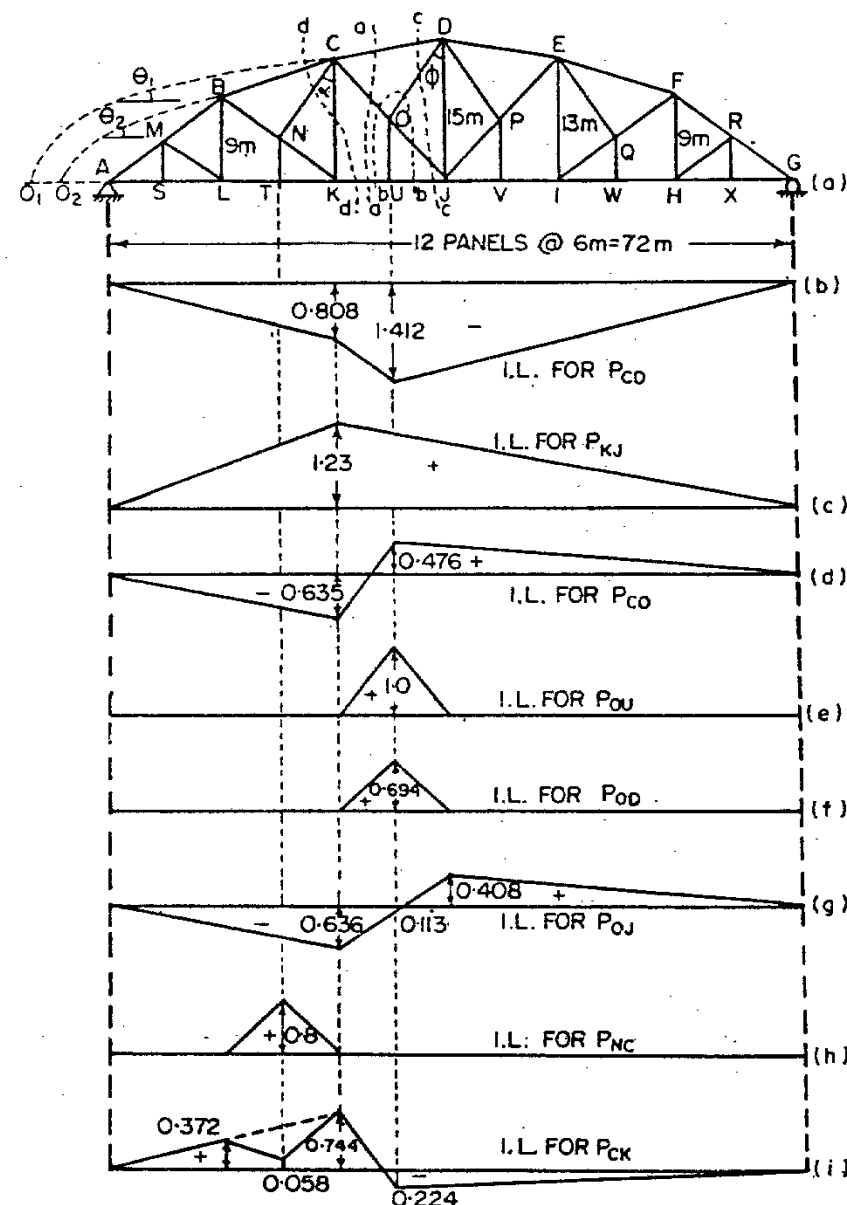
Fig. 4.8. Pettit truss with sub-ties
