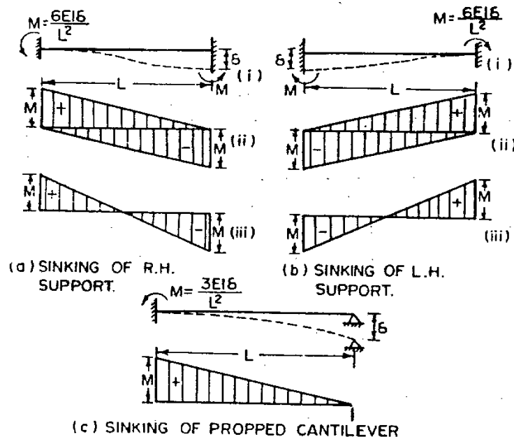
Fig. 10-11 Sinking of Supports
