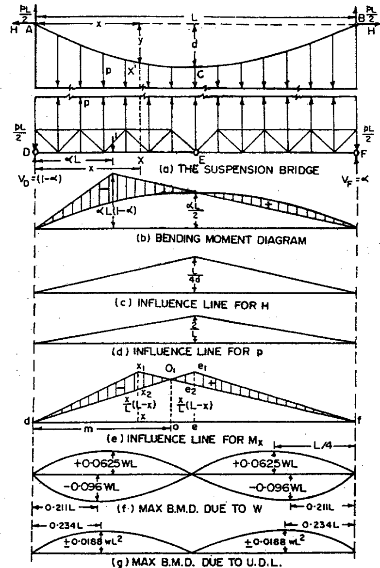
Fig. 15.13 Three hinged stiffening girder.
