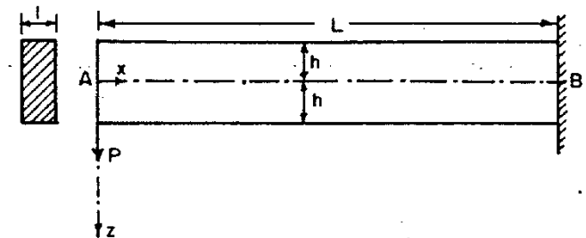
Fig. 22.11 Cantilever loaded at the end.
