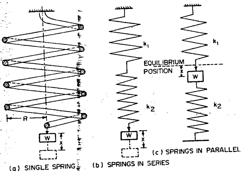
Fig. 19.2. Longitudinal vibrations of a helical spring.
