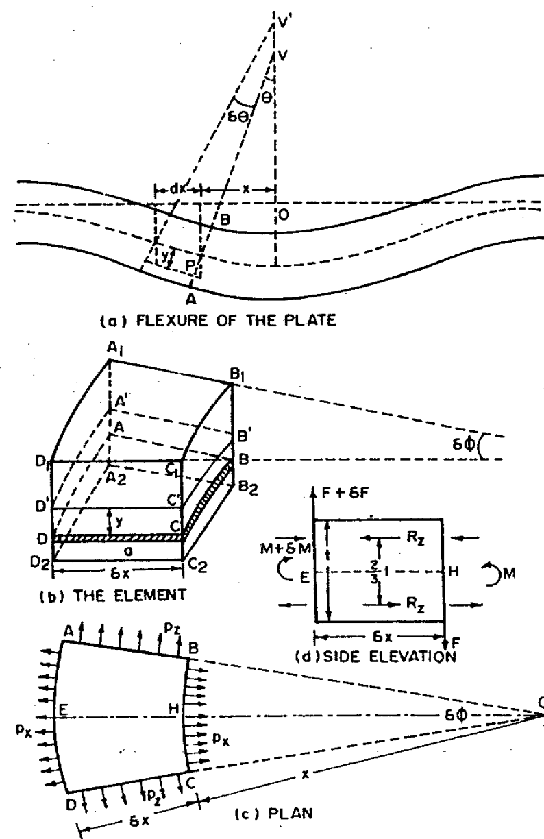
Fig. 20-1. Flat circular plate symmetrically loaded.
