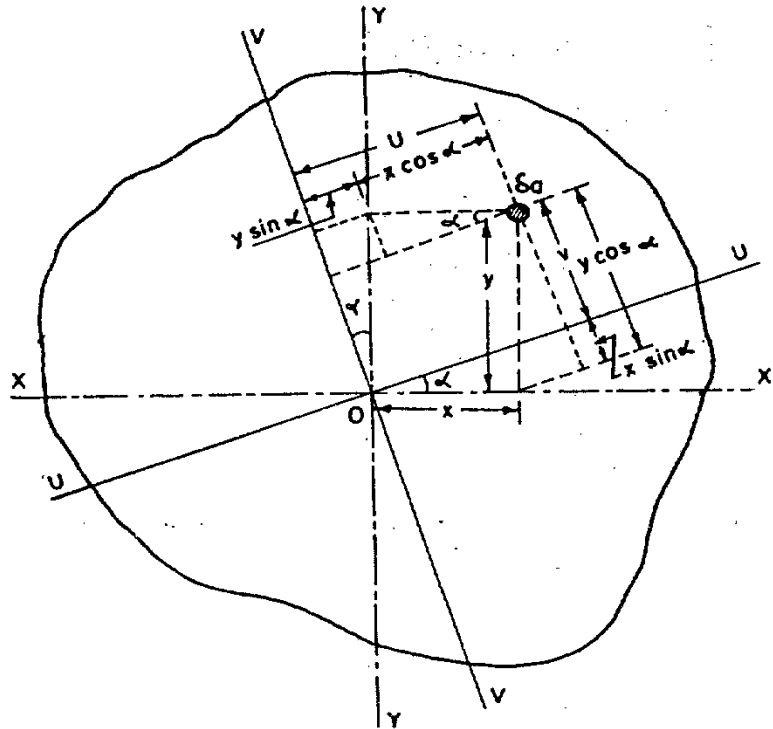
Fig. 21.2. Principal axes.
