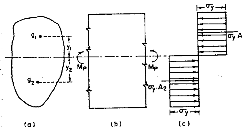
Fig. 26-8. Evaluation of fully plastic moment.
