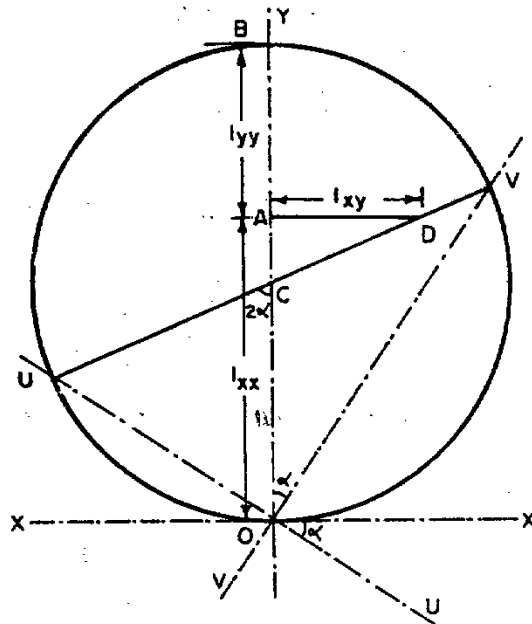
Fig. 21'4. Circle of Inertia (Dyadic Circle).
