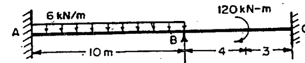
(a) THE BEAM WITH LOADING
