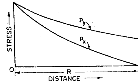
Fig. 18'4. Variations of p_x and p_y in a solid disc.
