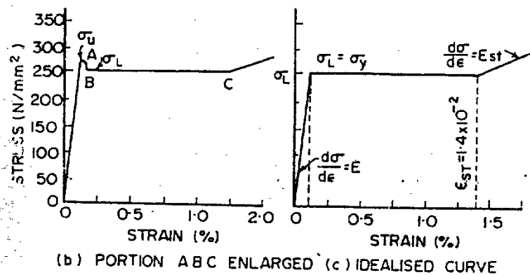
Fig. 26.1. Stress-Strain curves.
