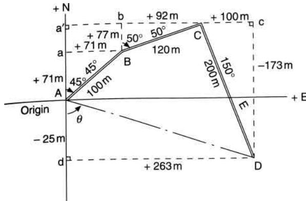
Fig. 11.6 Area by coordinates
