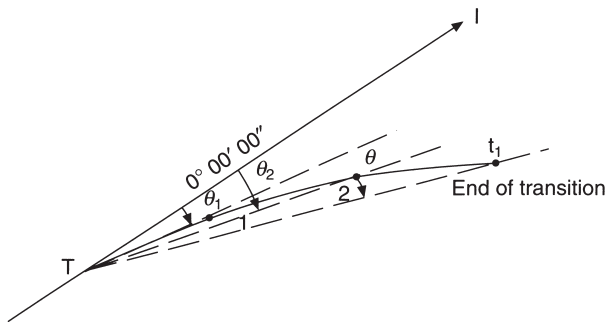
Fig. 10.29 Setting out the transitions
