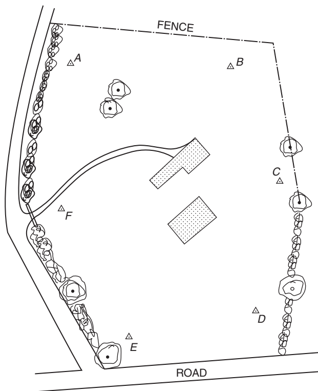
Fig. 1.4 Control points
