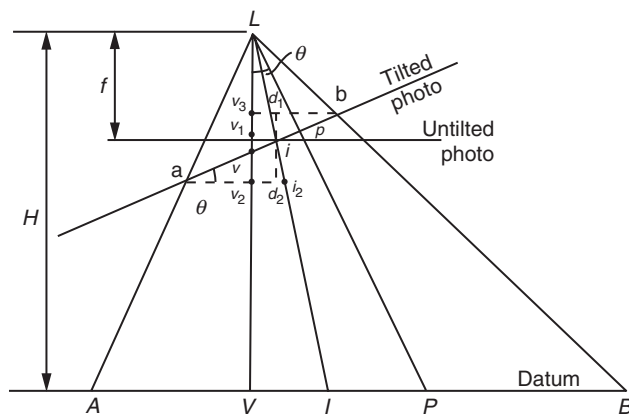
Fig. 14.9 Tilted photograph
