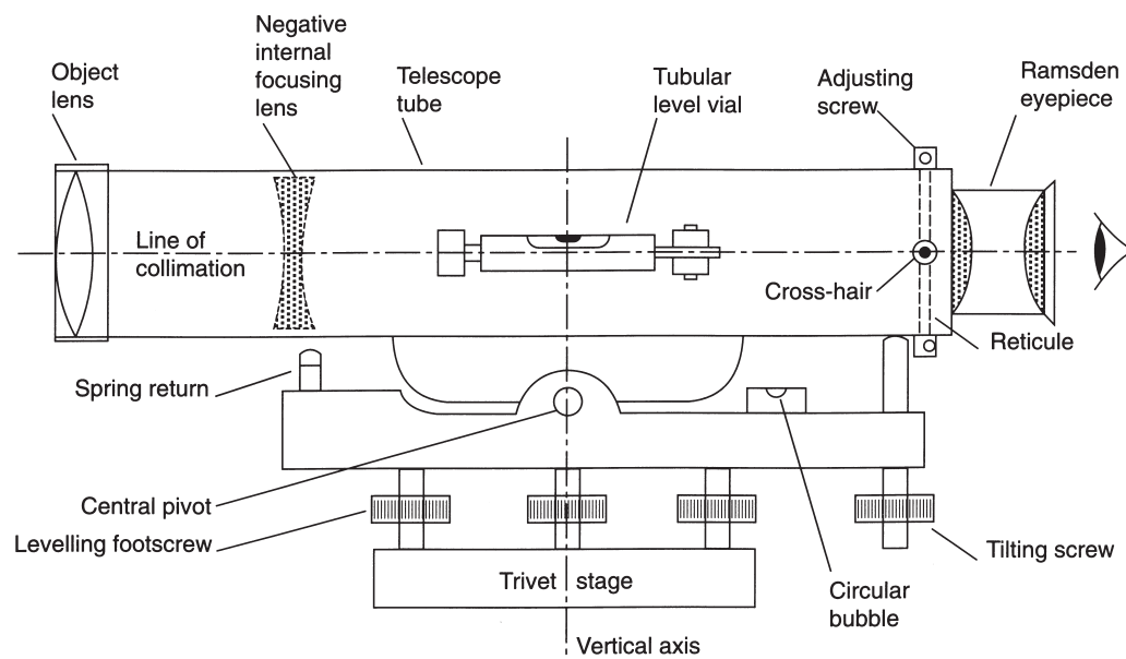
Fig. 3.10 Tilting level
