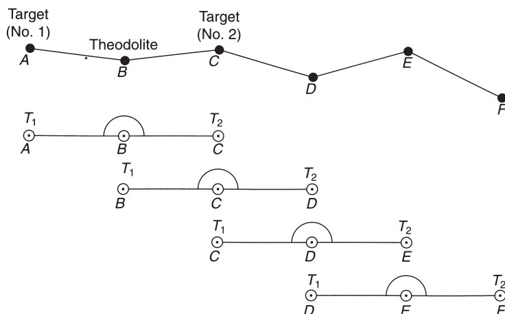
Fig. 6.17 Conventional three-tripod system
