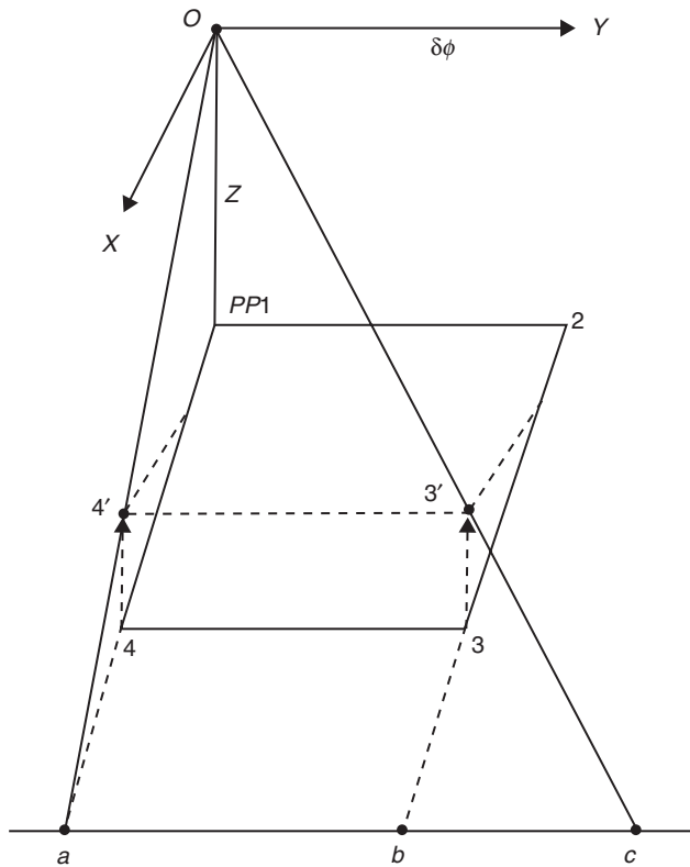
Fig. 14.29 Pitch of the aircraft
