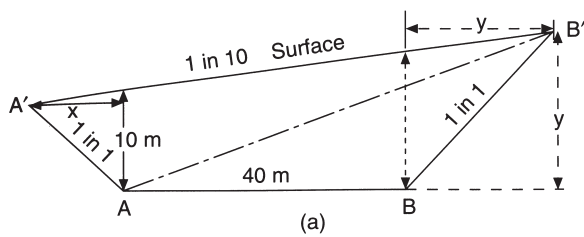
Fig. 11.23 Ground model
