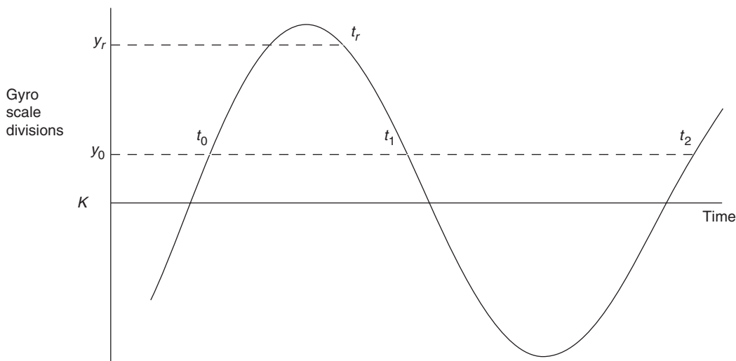
Fig. 13.18 Transit method
