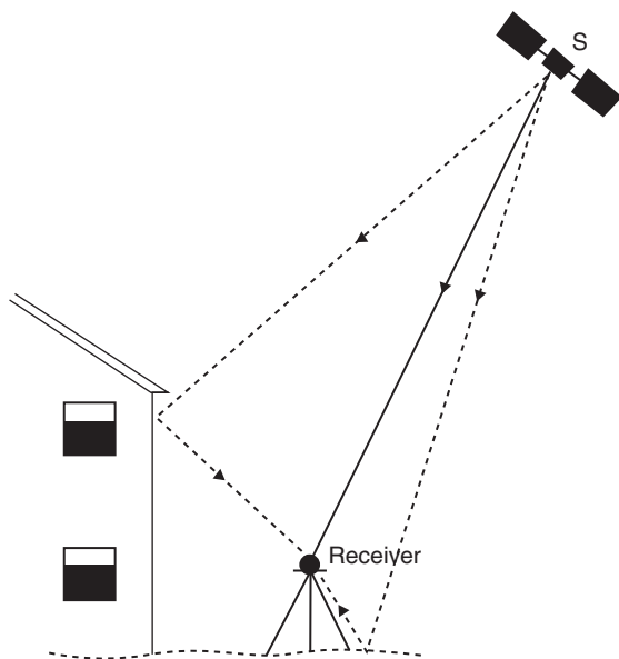
Fig. 9.18 Multipath effect
