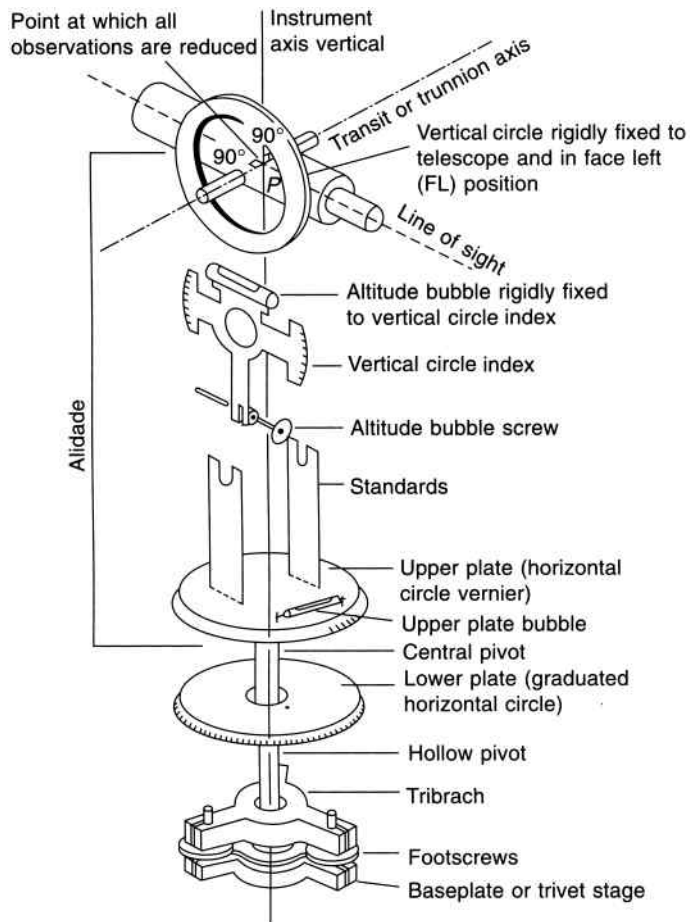
Fig. 5.3 Simplified theodolite
