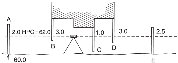
Fig. 3.22 Inverted sights
