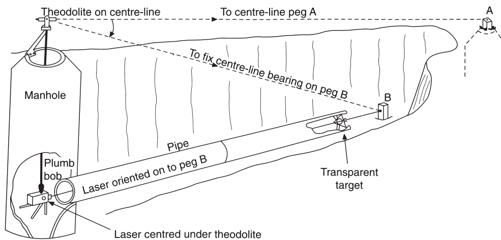
Fig. 12.24 Pipe laser in a manhole
