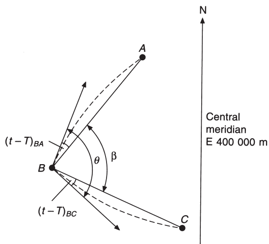
Fig. 8.22 t - T correction
