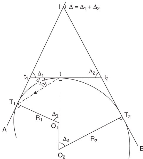
Fig. 10.14 Compound curve
