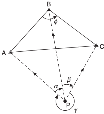
Fig. 6.27 Resection
