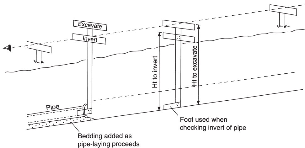
Fig. 12.19 Pipe laying
