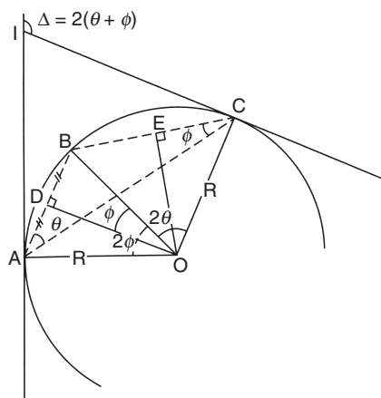
Fig. 10.23 Curve defined by three points
