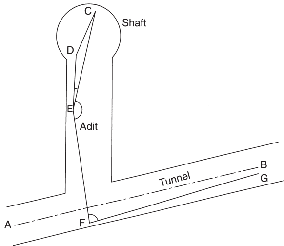
Fig. 13.8 Tunnel, shaft and adit
