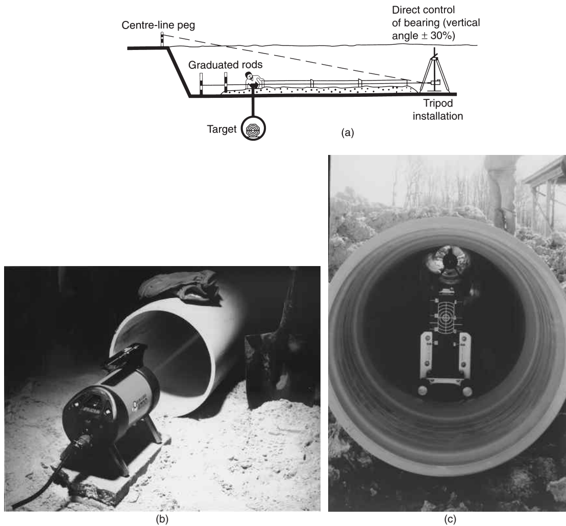
Fig. 12.23 (a) Pipe work, (b) pipe laser, (c) laser alignment in large-diameter pipe
