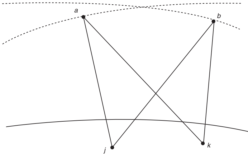
Fig. 9.14 Double difference
