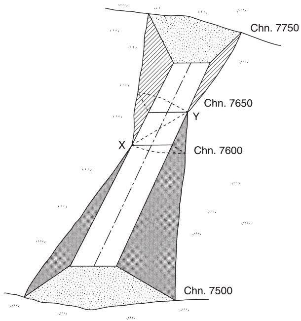
Fig. 11.26 Road excavation with cut and fill
