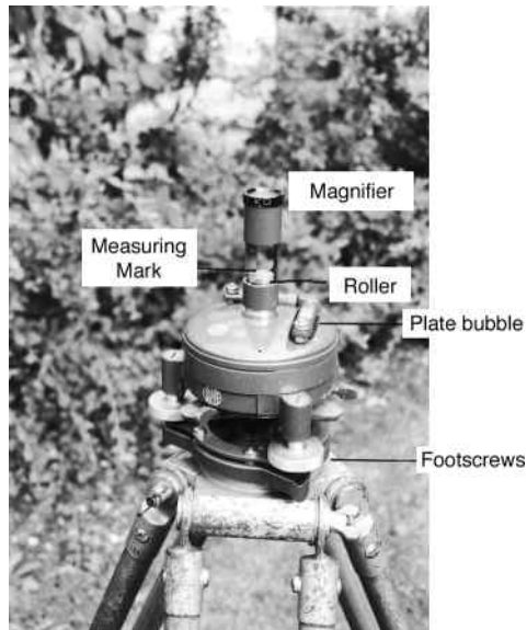
Fig. 4.7 Measuring head
