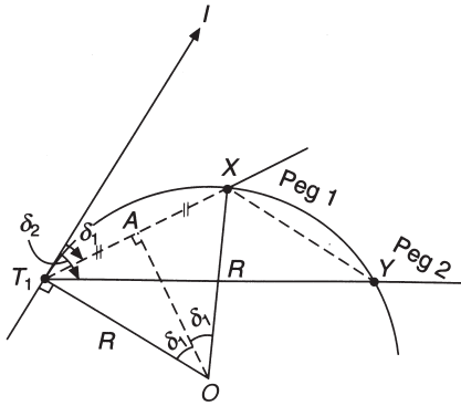
Fig. 10.4 Setting out with theodolite and tape
