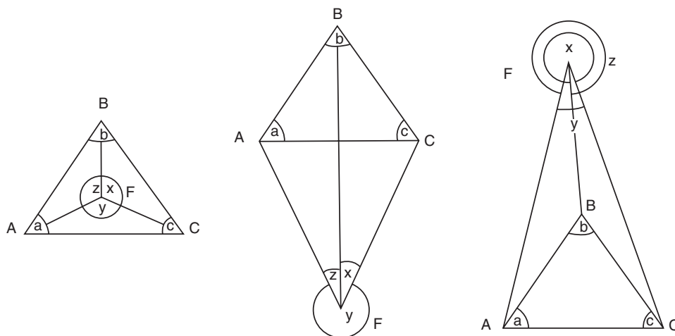
Fig. 6.28 Resection figures
