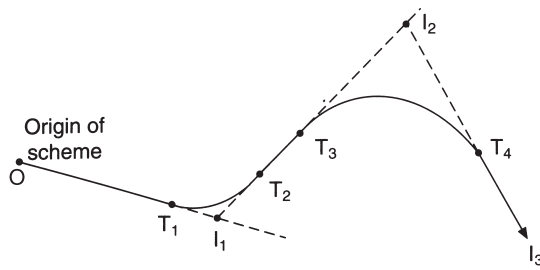
Fig. 10.3 Through chainage
