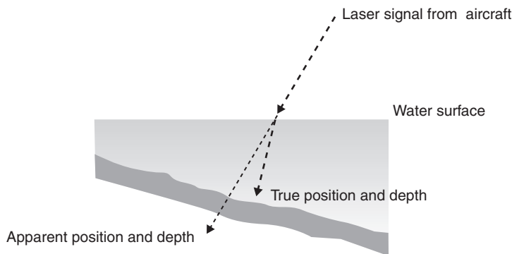
Fig. 14.47 Refraction effects in water
