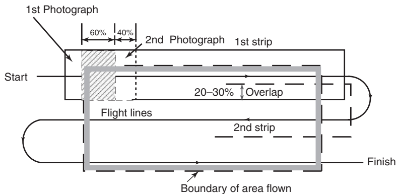
Fig. 14.16 Flight lines
