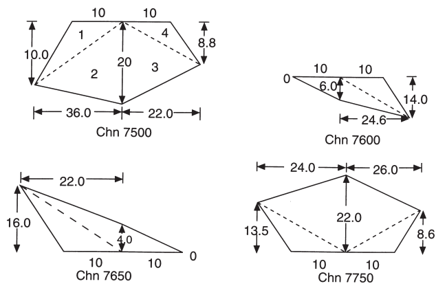
Fig. 11.27 Cross-sections
