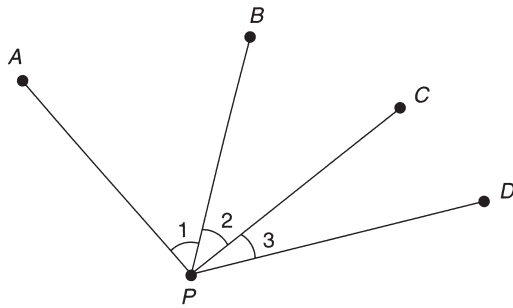
Fig. 5.31 Directions measurements
