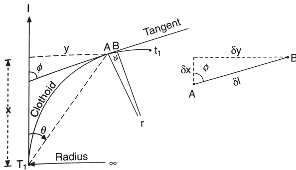
Fig. 10.50 Clothoid spiral
