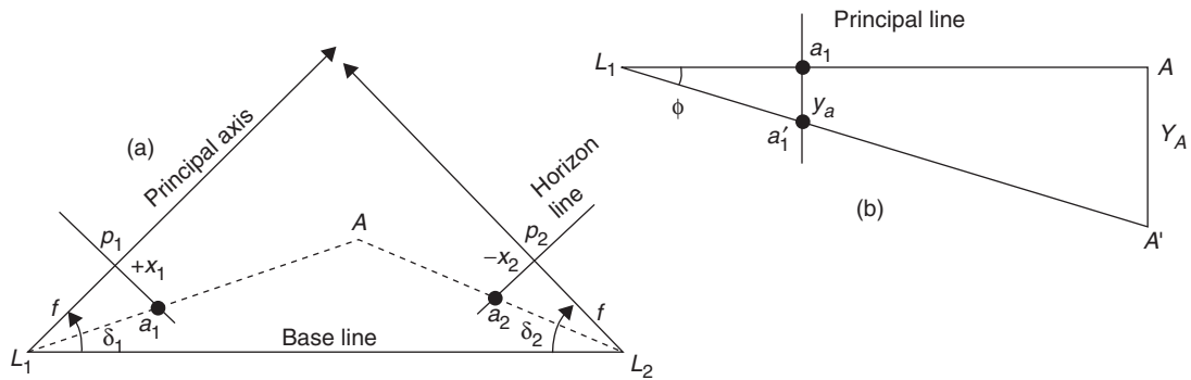
Fig. 14.38 (a) Plan view and (b) elevation
