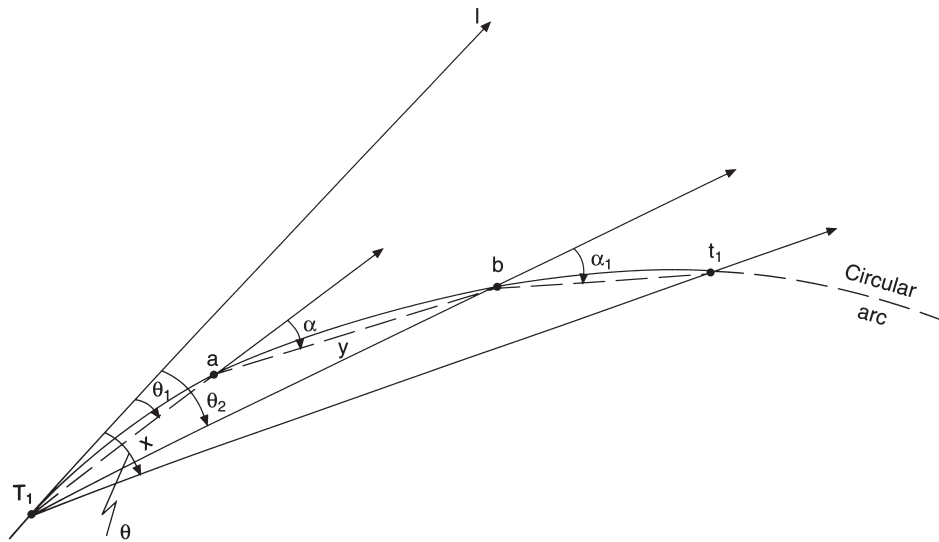
Fig. 10.37 Coordinates along a transition curve
