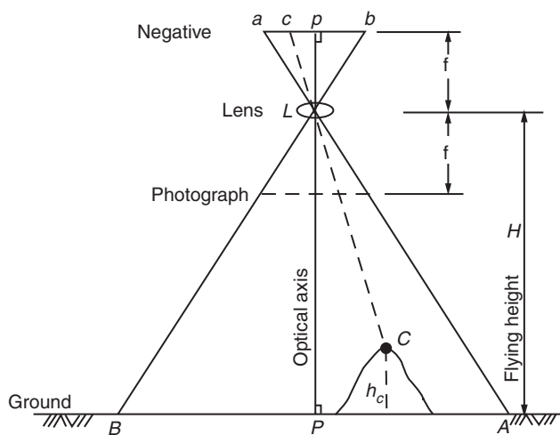
Fig. 14.8 Photo scale
