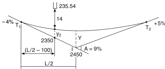
Fig. 10.48 Offset on a curve, at a given point
