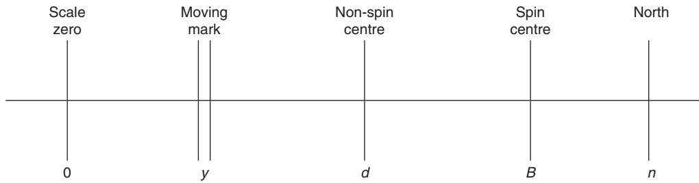
Fig. 13.16 Points of interest on the gyro scale
