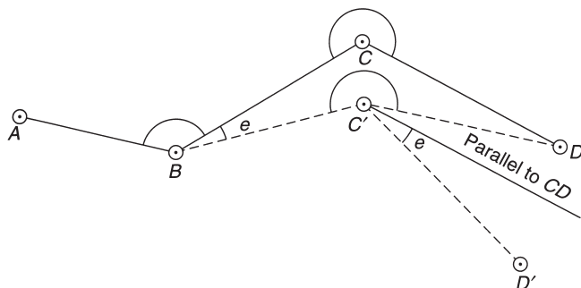
Fig. 6.18 Propagation of centring error
