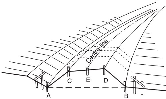
Fig. 12.27 Pegging out a route
