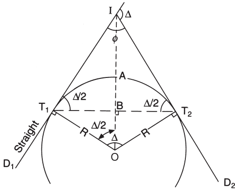
Fig. 10.1 Circular curve
