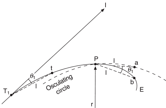
Fig. 10.31 Osculating circle
