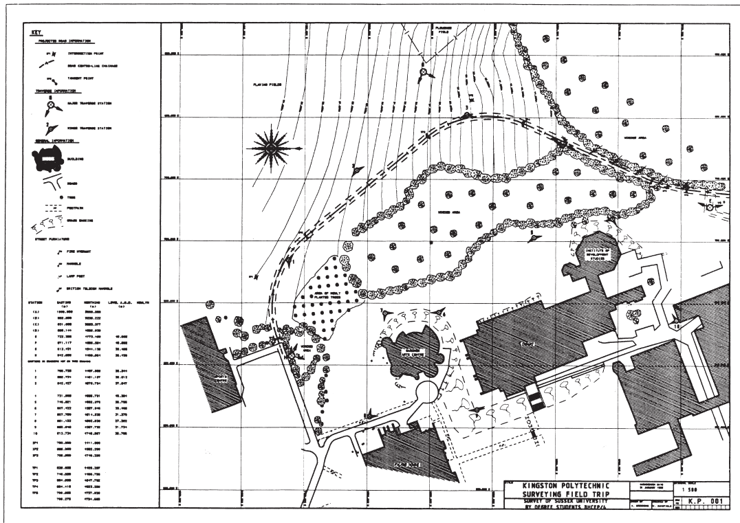
Fig. 1.13 Computer plot
