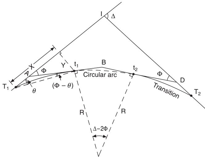
Fig. 10.28 Transition and circular curves
