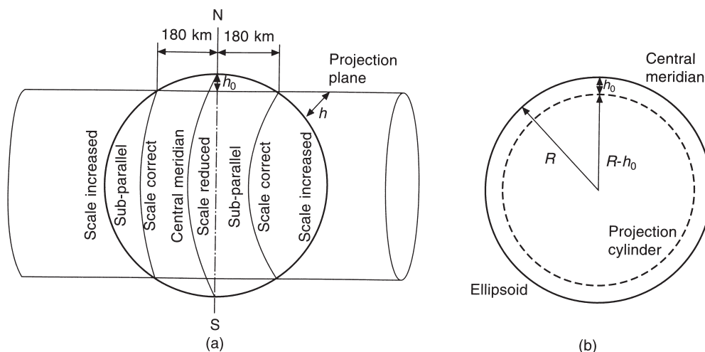
Fig. 8.18 Scale on the projection
