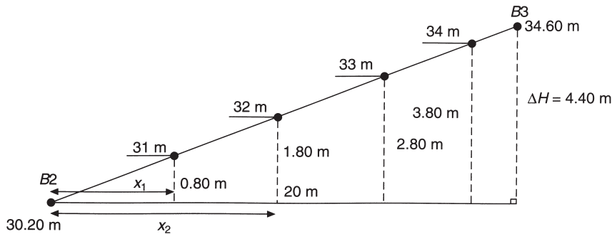
Fig. 3.29 Contour calculations
