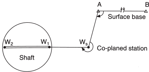
Fig. 13.4 Co-planing
