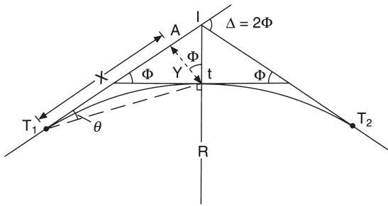
Fig. 10.30 Transitional curve throughout
