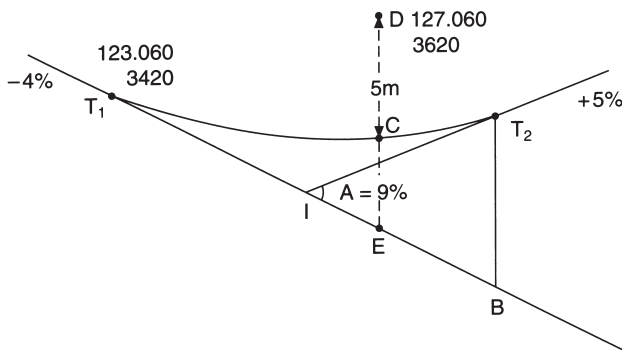
Fig. 10.45 Clearance at a given point
