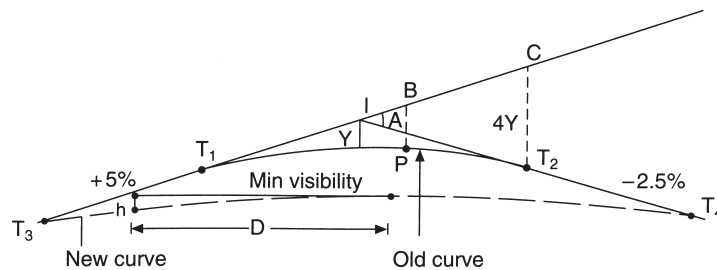
Fig. 10.46 Minimum visibility
