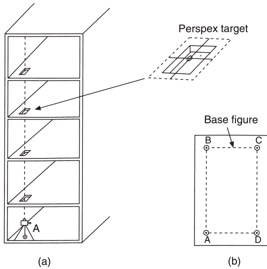
Fig. 12.15 (a) Elevation, and (b) plan
