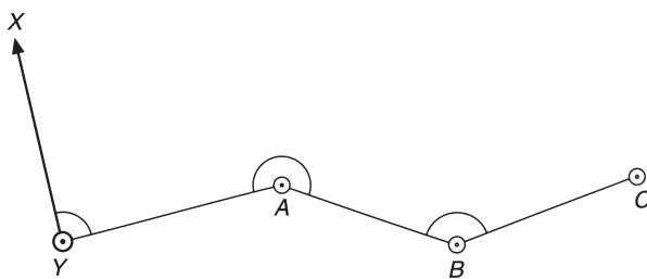
Fig. 6.13 Open (or free) traverse
