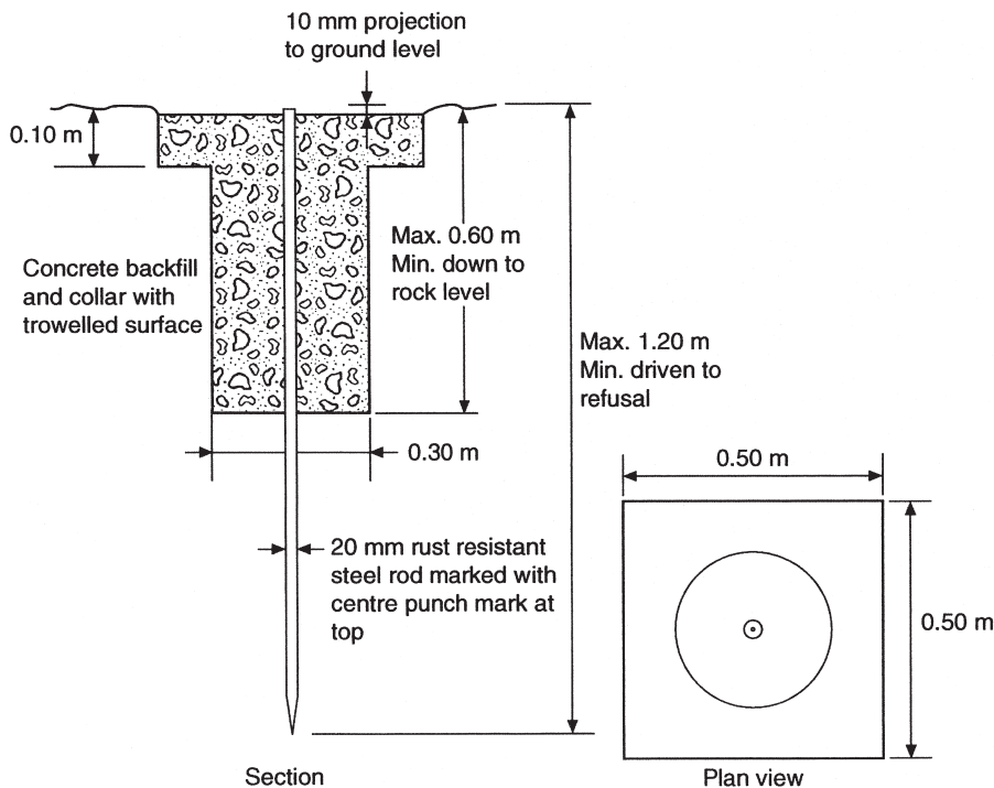
Fig. 6.14 Survey station
