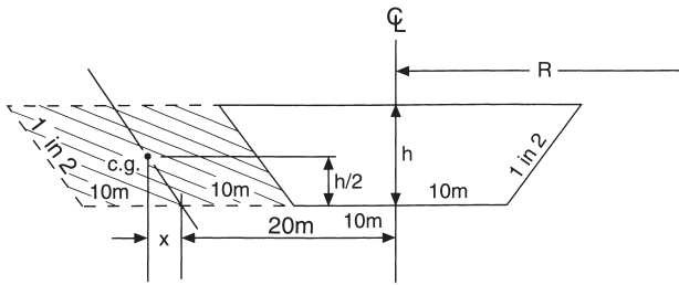
Fig. 11.31 Road cross-section
