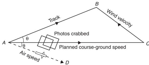
Fig. 14.19 The effect of crab
