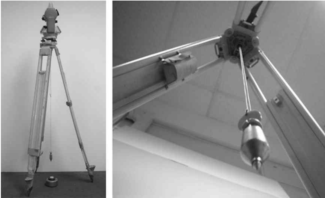
Fig. 5.27 Theodolite with plumb-bob
