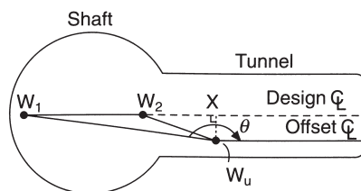
Fig. 13.20 Plan view
