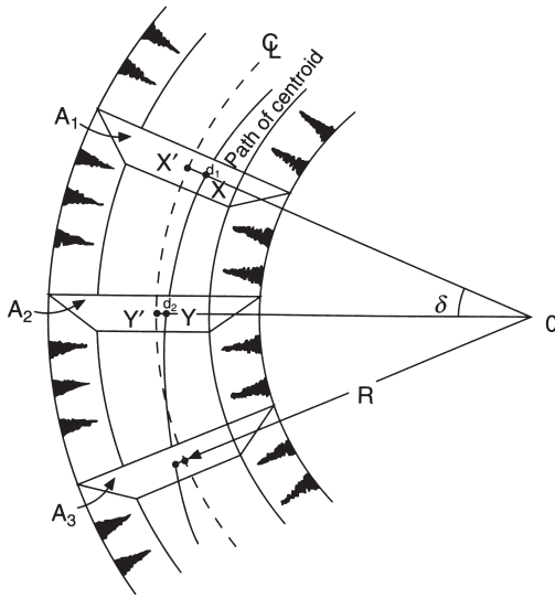
Fig. 11.25 Curved excavation
