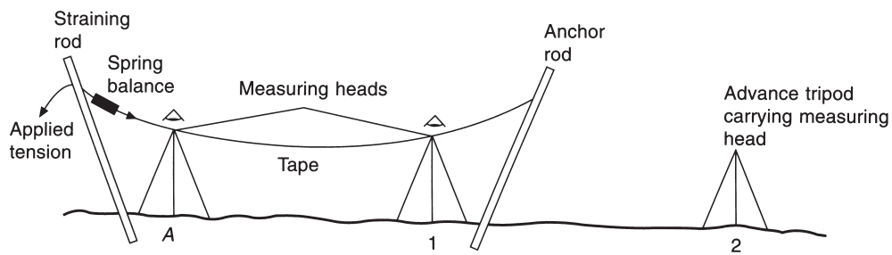
Fig. 4.5 Suspended tape
