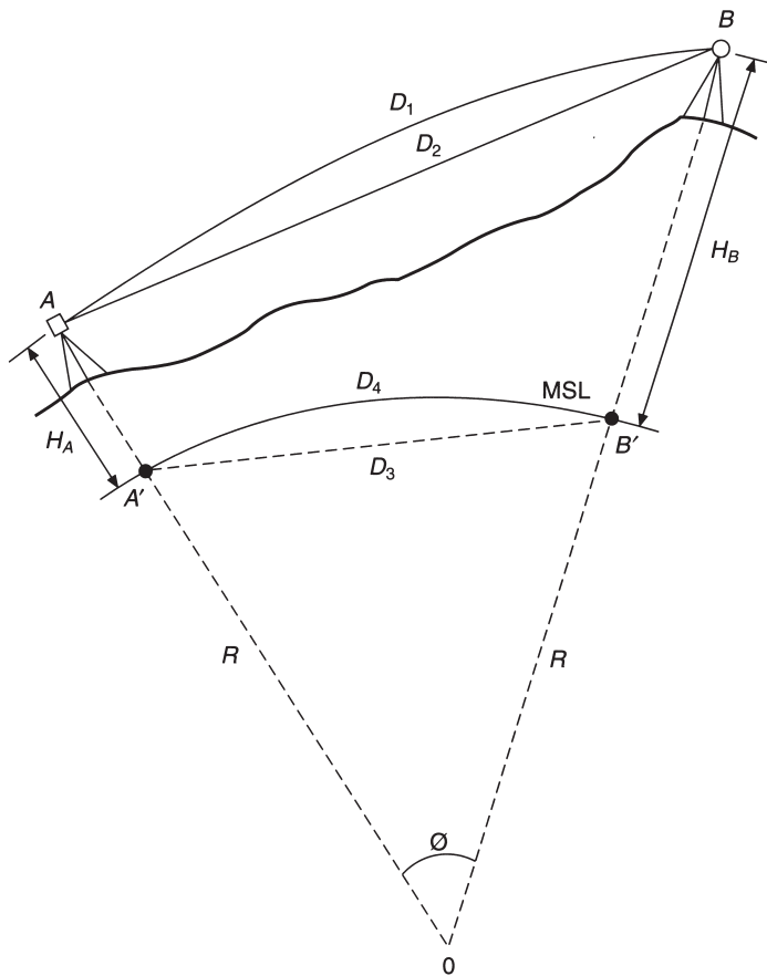
Fig. 4.24 Distance reductions
