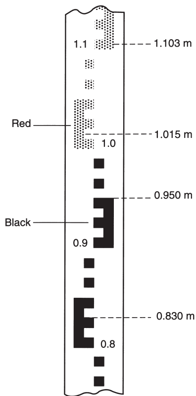
Fig. 3.9 Levelling staff
