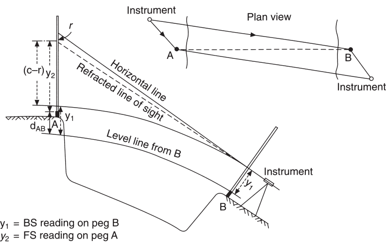
Fig. 3.32 Reciprocal levelling
