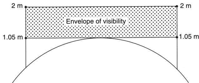
Fig. 10.41 Overtaking visibility
