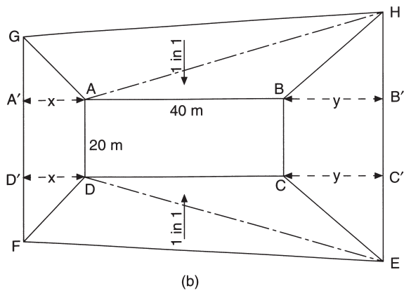
Fig. 11.24 Calculate volume of shape defined by planes
