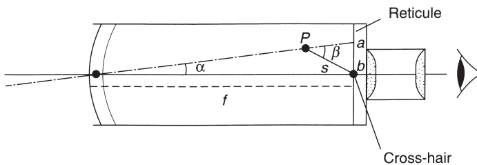
Fig. 3.15 Principle of compensator
