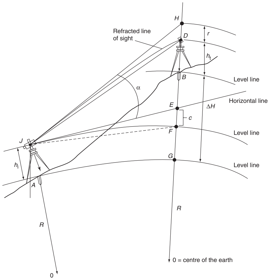
Fig. 3.43 Trigonometric levelling – long lines
