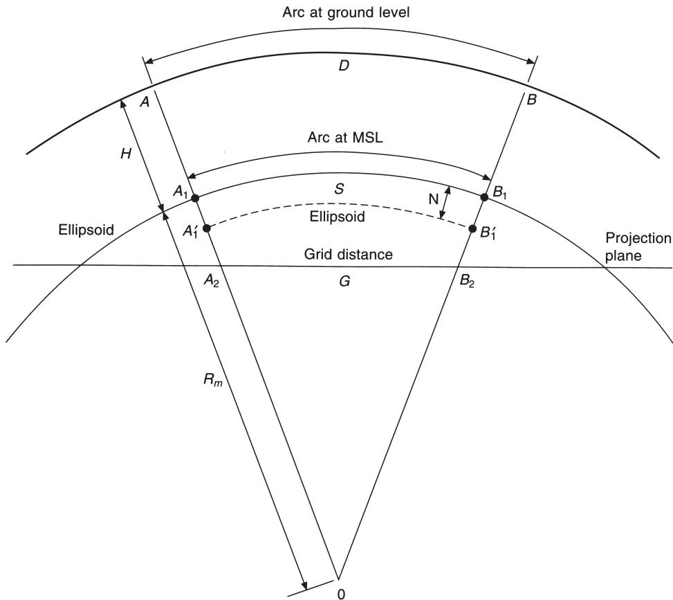
Fig. 8.20 Distance reduction
