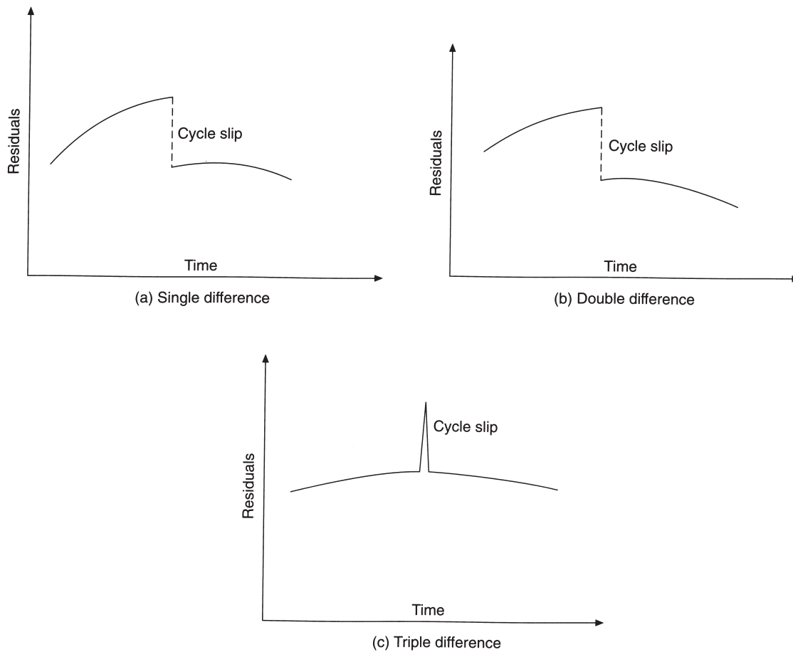
Fig. 9.16 Cycle slips
