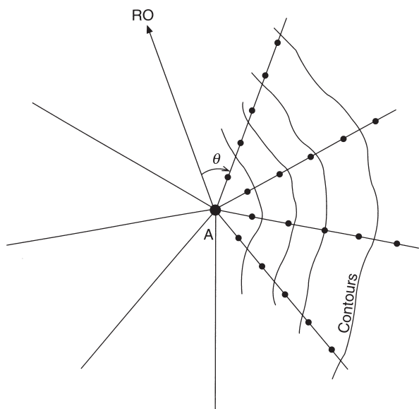
Fig. 3.47 Radiation method
