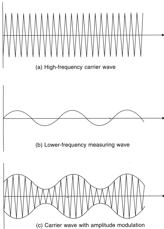
Fig. 4.14 Amplitude modulation of the carrier wave
