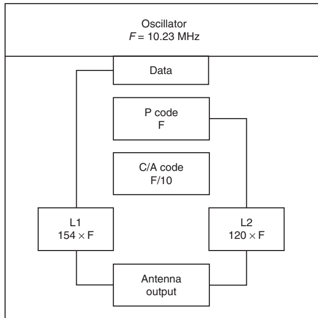
Fig. 9.3 GPS signal generation
