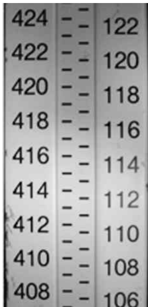
Fig. 3.33 Segment of a precise levelling staff
