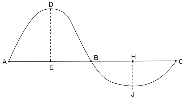
Fig. 11.37 Mass haul diagram
