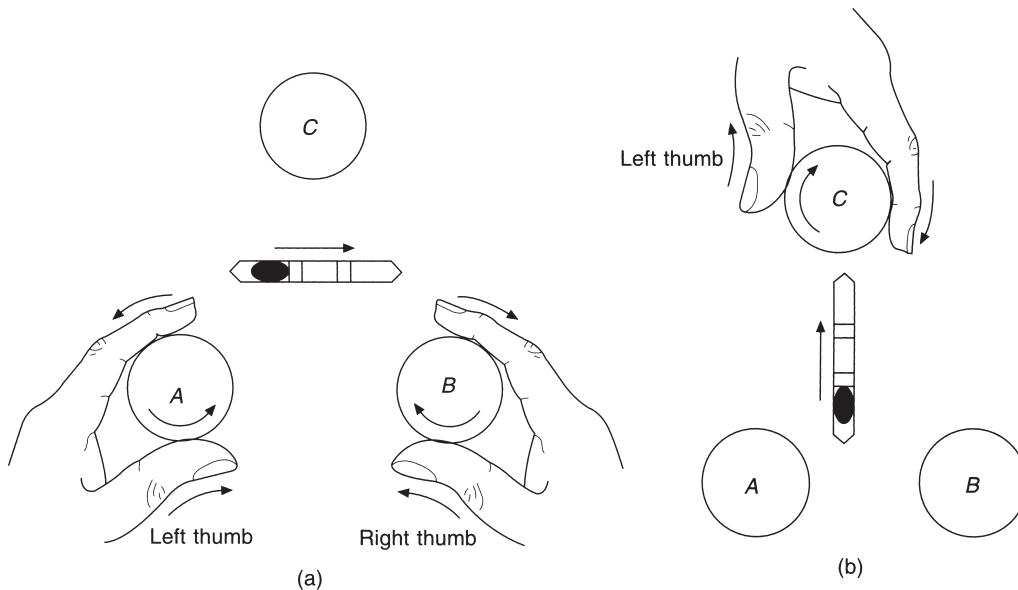
Fig. 5.28 Footscrews
