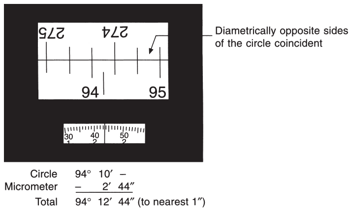
Fig. 5.7 Wild T2 (old pattern) theodolite reading system
