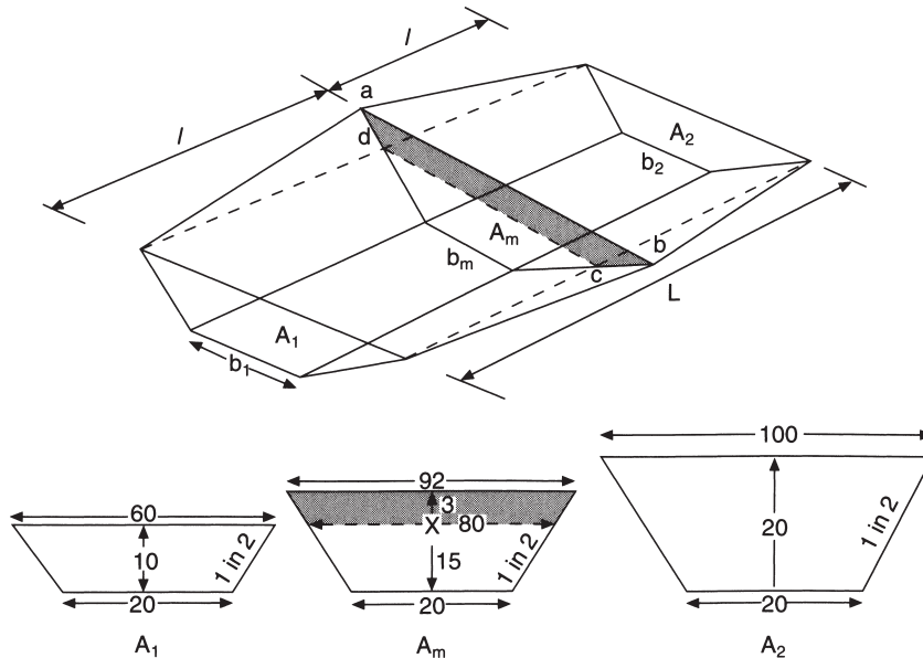
Fig. 11.21 End-area calculation
