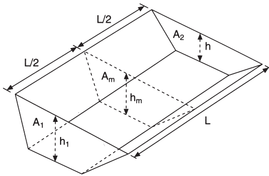
Fig. 11.20 Prismoid
