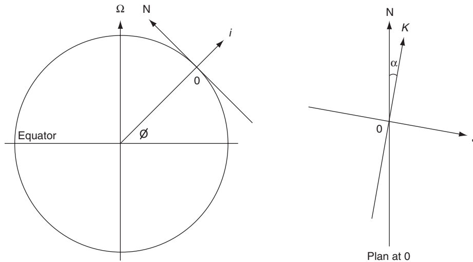
Fig. 13.13 (a) Meridian section through the earth, (b) Plan view at 0
