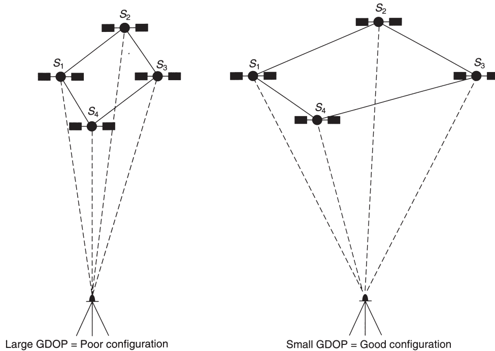
Fig. 9.19 Satellite configuration
