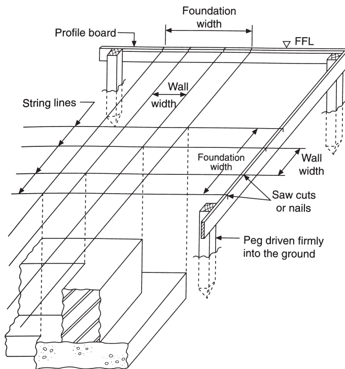
Fig. 12.8 Profile boards
