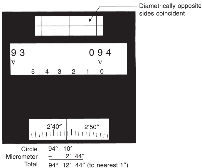
Fig. 5.8 Wild T2 (new pattern)
