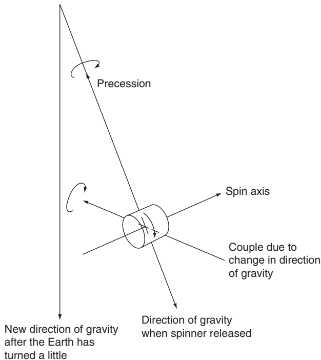
Fig. 13.15 Motion of the spinner
