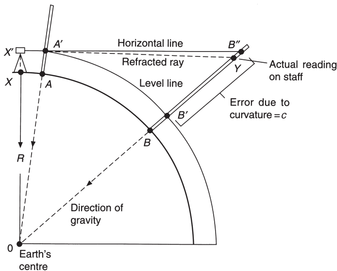
Fig. 3.6 Horizontal and level lines
