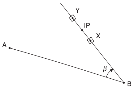
Fig. 12.5 Setting out with a steel tape
