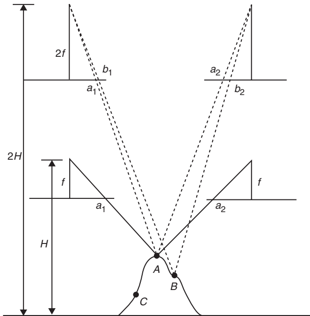
Fig. 14.20 Flying height
