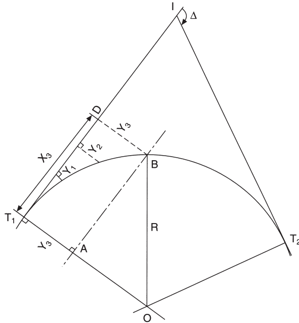
Fig. 10.16 Offsets from the tangent
