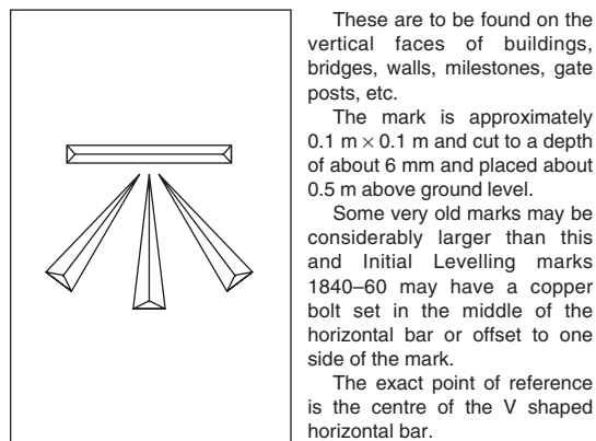
Fig. 3.2 Cut bench mark
