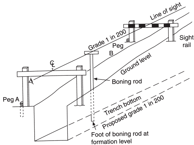
Fig. 12.17 Trench excavation
