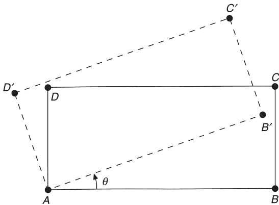
Fig. 6.12 Orientation error in a traverse
