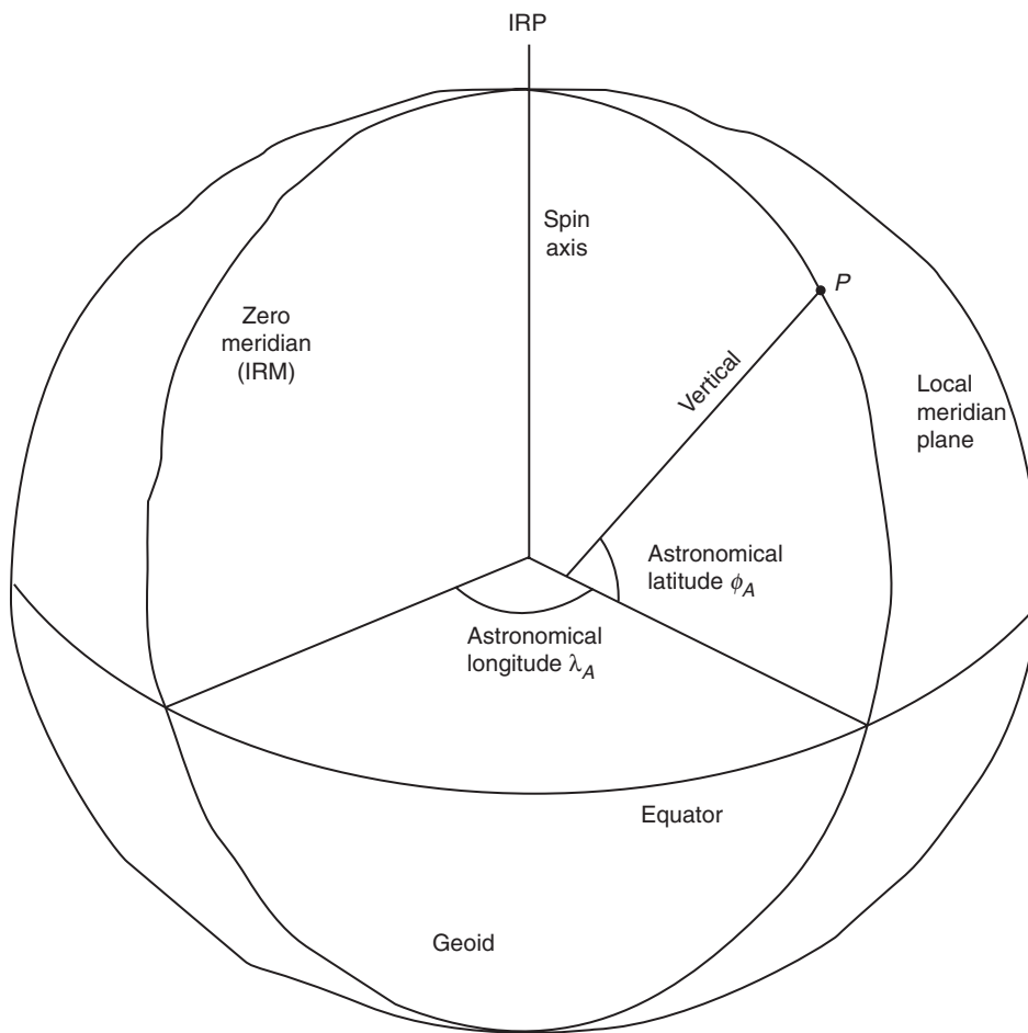
Fig. 8.6 Astronomical coordinates
