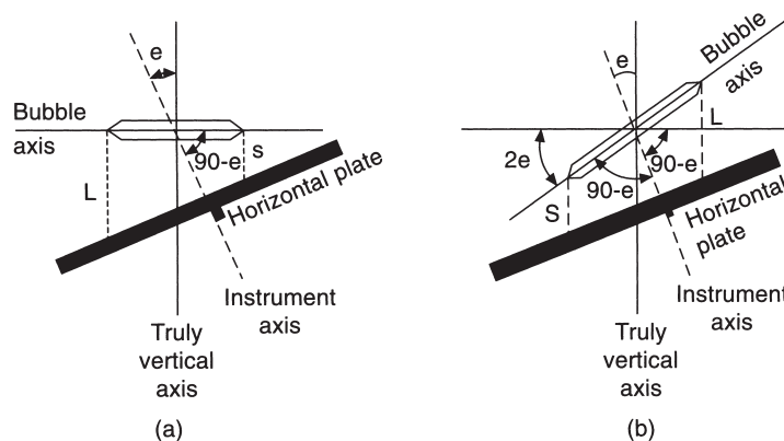
Fig. 5.22 Misaligned plate bubble. (a) When levelled over two footscrews, (b) when turned through 180^\circ
