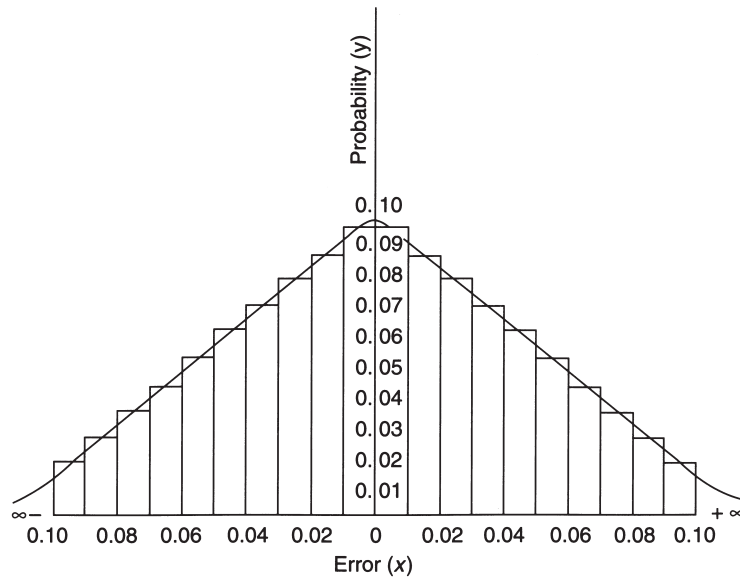
Fig. 2.2 Probability histogram
