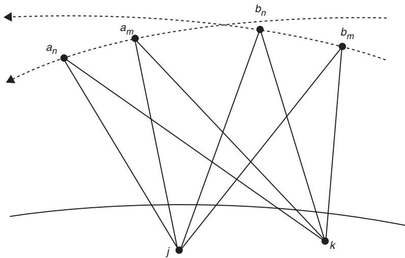
Fig. 9.15 Triple difference
