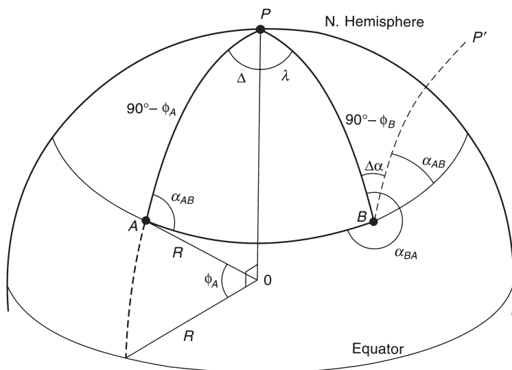
Fig. 8.13 Geodetic azimuth
