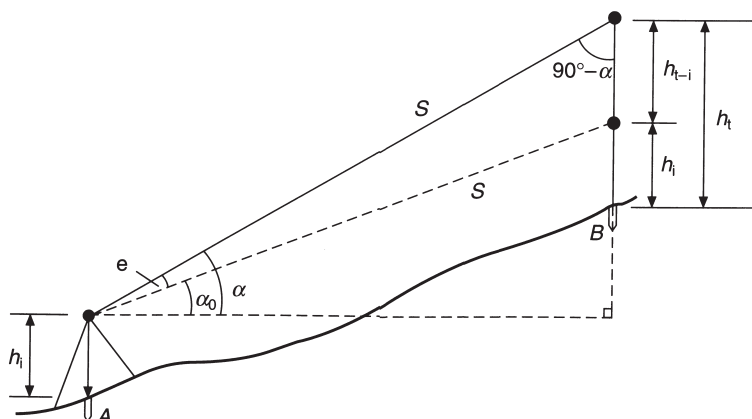
Fig. 3.45 Correction for unequal instrument and target height
