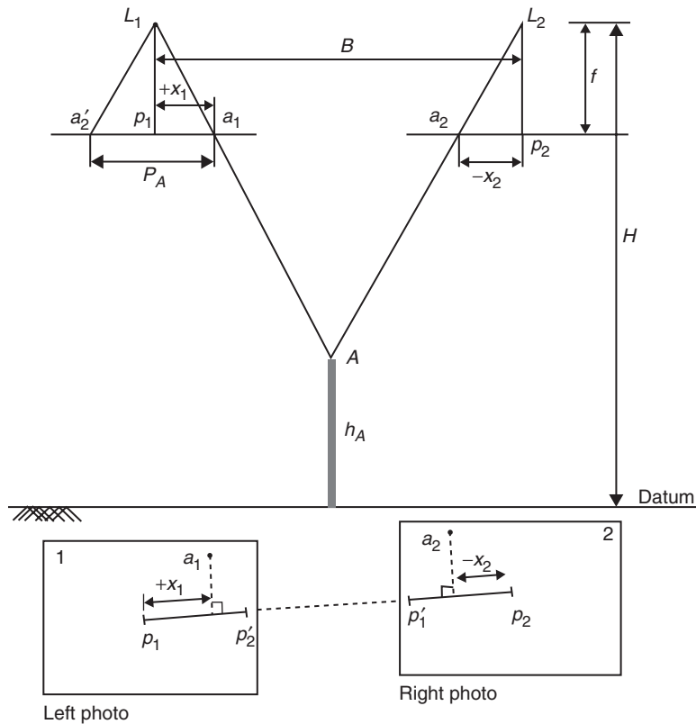
Fig. 14.24 Photo parallax
