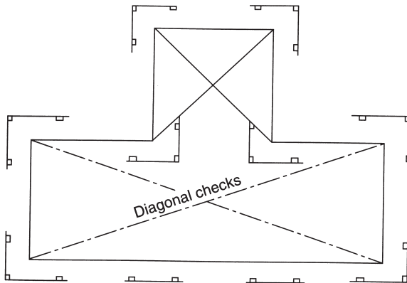
Fig. 12.9 Check measurements
