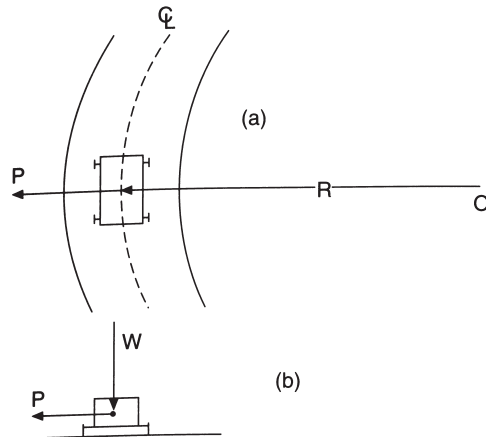
Fig. 10.24 Centrifugal force
