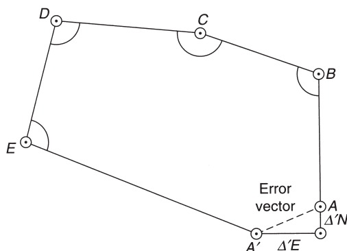
Fig. 6.21 Coordinate misclosure
