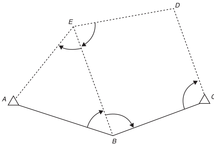
Fig. 7.13 Unreliable observations
