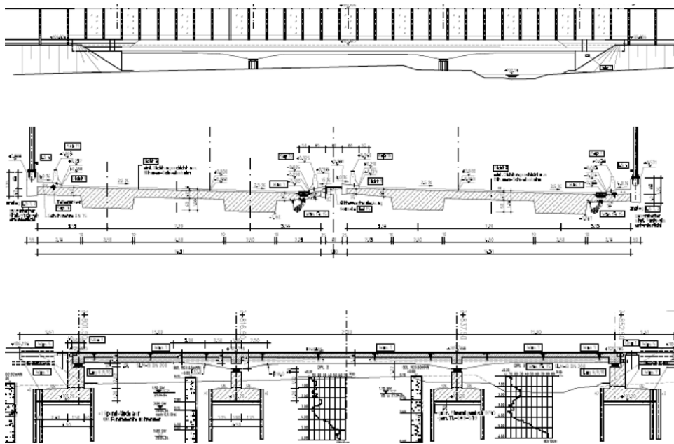
Figure 2.10 Design schemes of the prestressed concrete bridge
