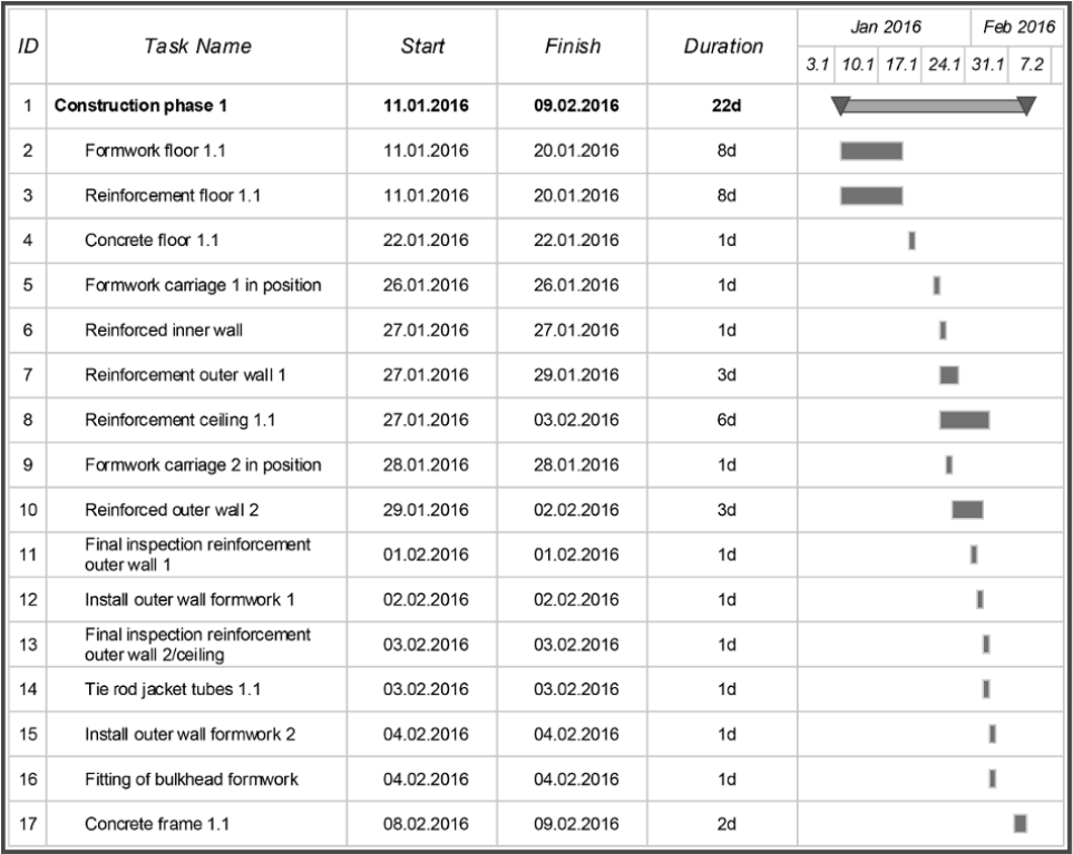
Figure 2.30 Schedule – Construction stage one
