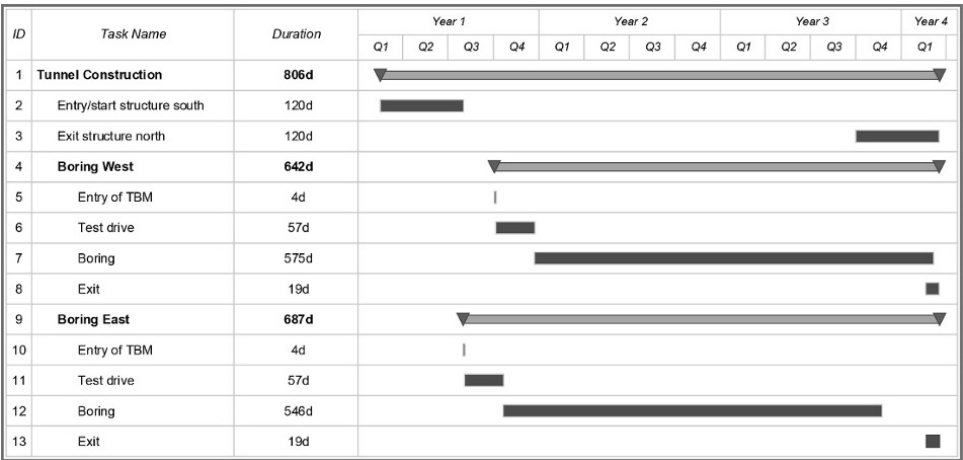
Figure 2.15 Example of a schedule for tunnel construction
