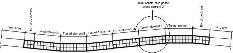
Figure 2.24 Floating assembly
