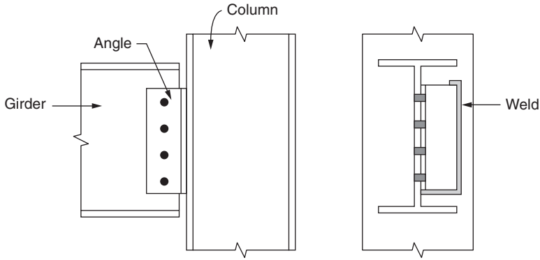
FIGURE 3.5 Single-angle connection.
