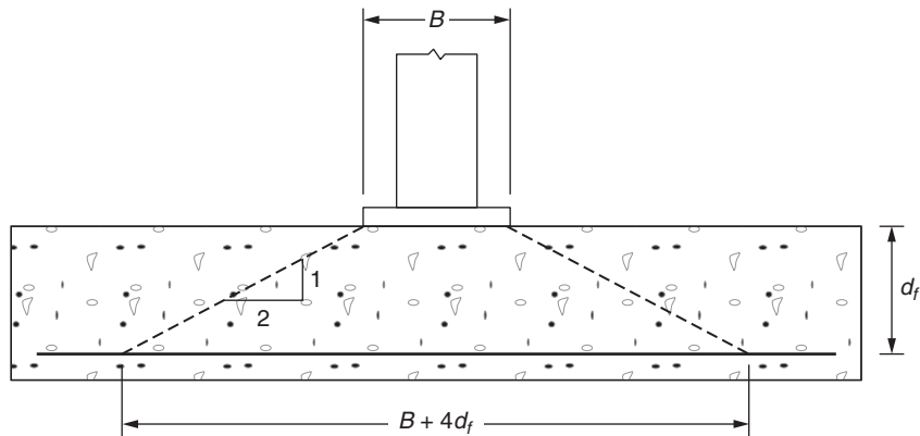
FIGURE 6.12 Concrete footing.
