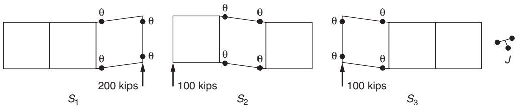
FIGURE 8.13 Independent mechanisms.
