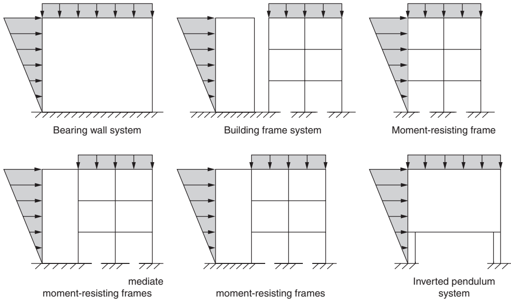
FIGURE 2.42 Structural systems.
