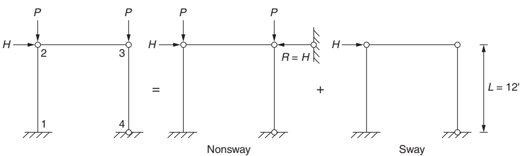
FIGURE 7.7 Details for Example 7.3.
