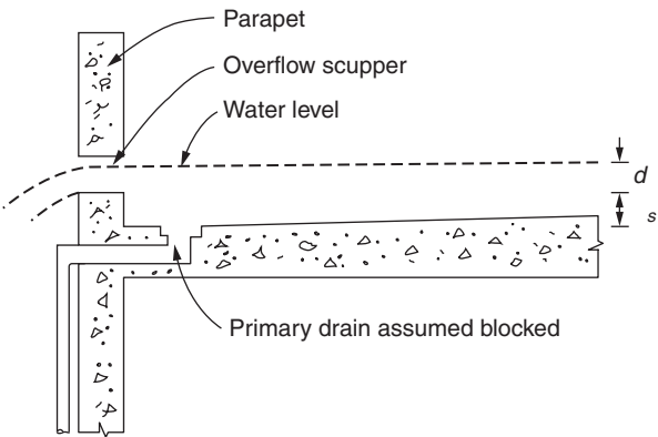
FIGURE 2.30 Roof drainage.
