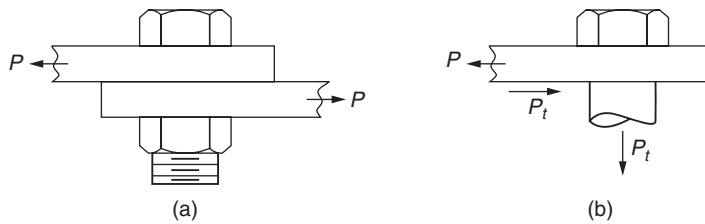
FIGURE 10.3 Slip-critical connection.
