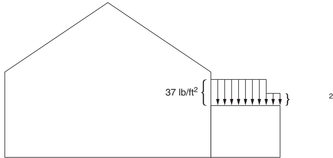
FIGURE 2.28b Sliding snow load on garage roof.
