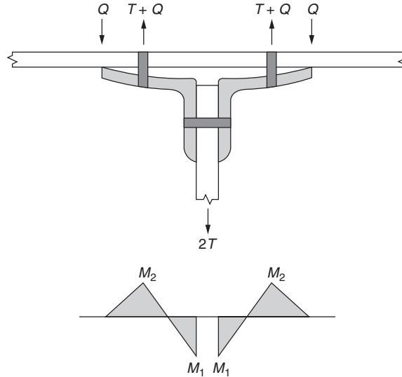
FIGURE 10.13 Double angle hanger with prying action.
