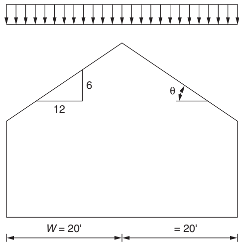
FIGURE 2.21 Balanced snow load on sloped roof.
