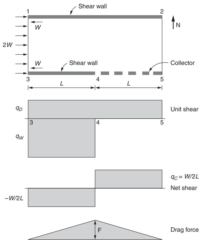
FIGURE 3.24 Collector force.
