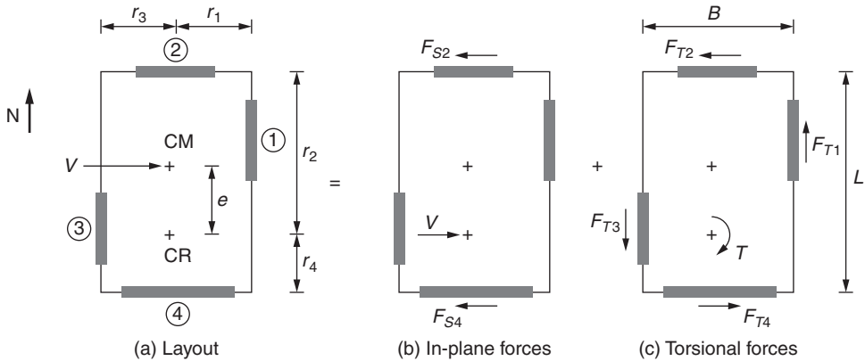
FIGURE 2.49 Rigid diaphragm.
