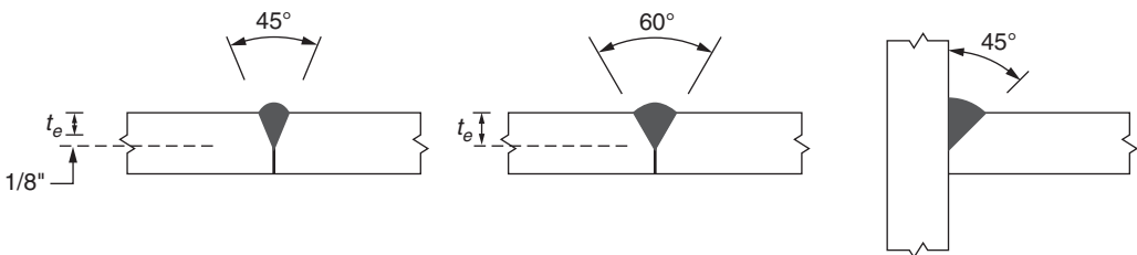
FIGURE 11.2 Partial joint penetration groove weld: SMAW.
