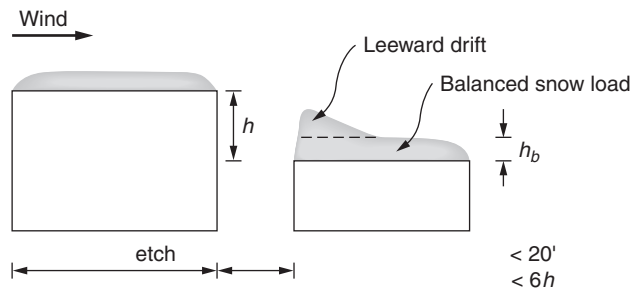
FIGURE 2.16 Drift formed on adjacent low structure.
