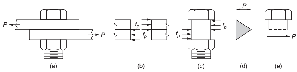
FIGURE 10.2 Snug-tight bolt stresses.
