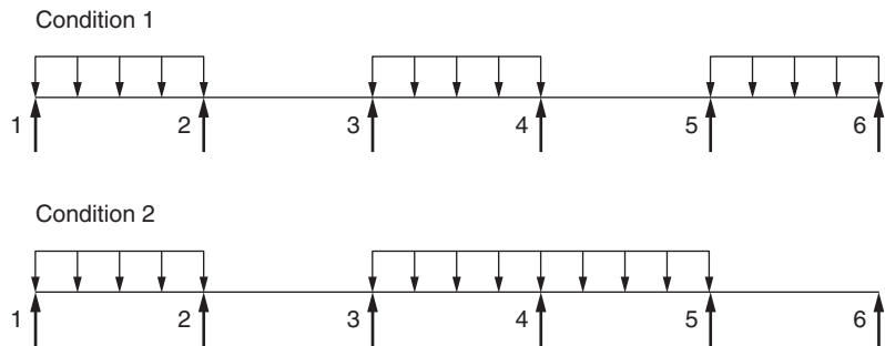
FIGURE 2.13 Partial loading conditions.
