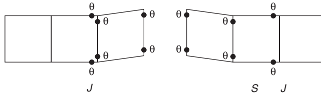
FIGURE 8.14 Combined mechanisms.
