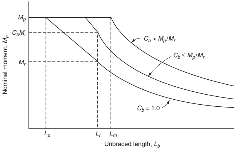
FIGURE 4.10 Lateral-torsional buckling.
