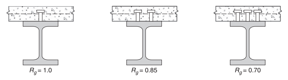
FIGURE 13.17 Stud group coefficient, ribs perpendicular to beam.
