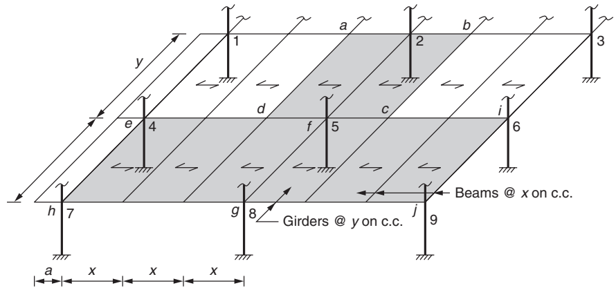
FIGURE 2.14 Influence areas.
