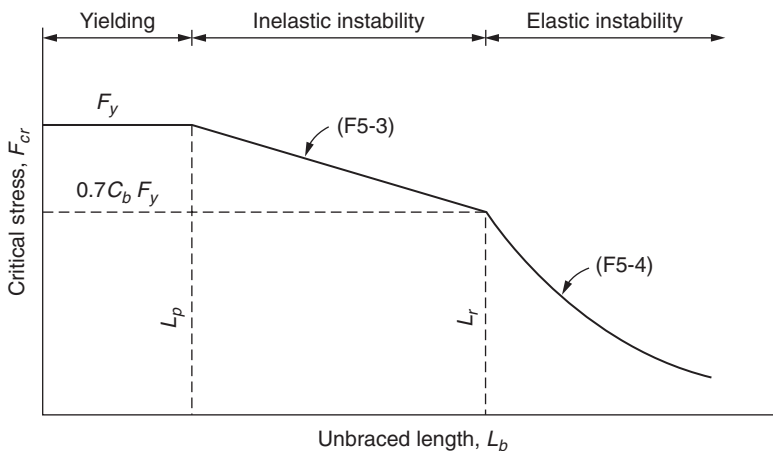
FIGURE 12.6 Variation of critical stress with lateral support.
