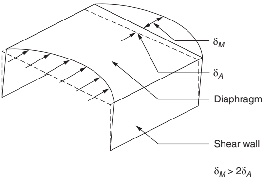
FIGURE 2.46 Flexible diaphragm.
