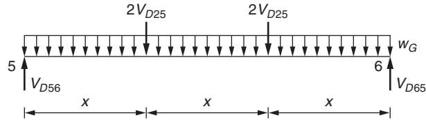
FIGURE 2.5 Dead load on girder 56.
