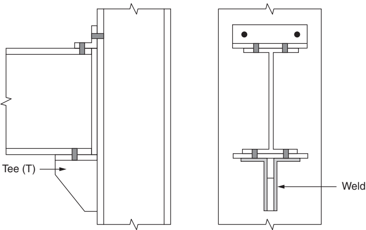
FIGURE 3.9 Stiffened-seated connection.
